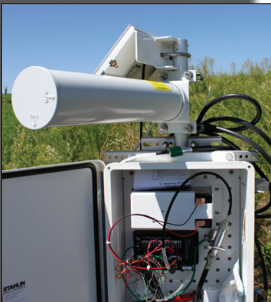
Figure 2. A wireless (remote) soil moisture monitoring station contains transmitting antenna, a solar panel, a seal battery, and a data logger/radio in an environmental enclosure.
