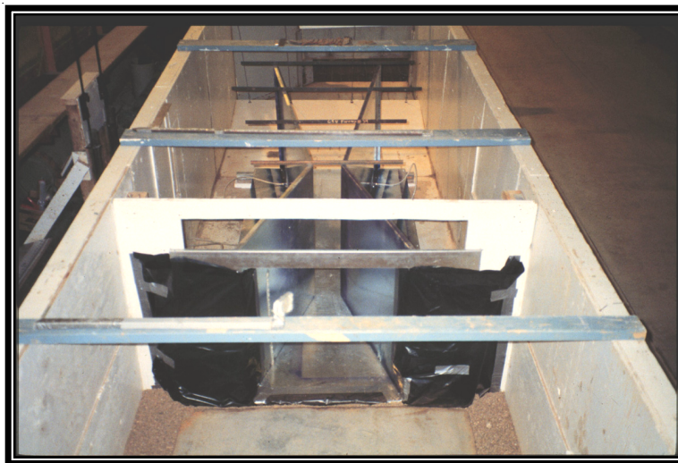
Performing field verification of cutthroat flume tests
