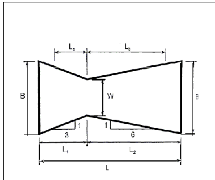
Figure 1. Cutthroat Flume Dimensions (Plan View)
