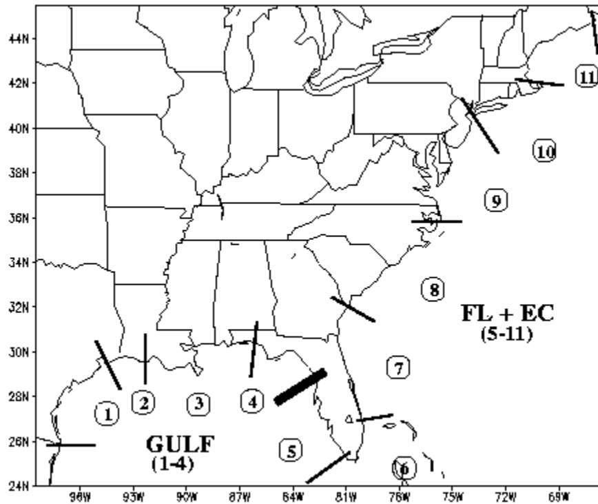
Figure 5: Location of the 11 coastal regions for which separate hurricane landfall probability estimates are made. The heavy bar delineates the boundary between the Gulf (regions 1-4) and the Florida Peninsula and East Coast (regions 5-11).
