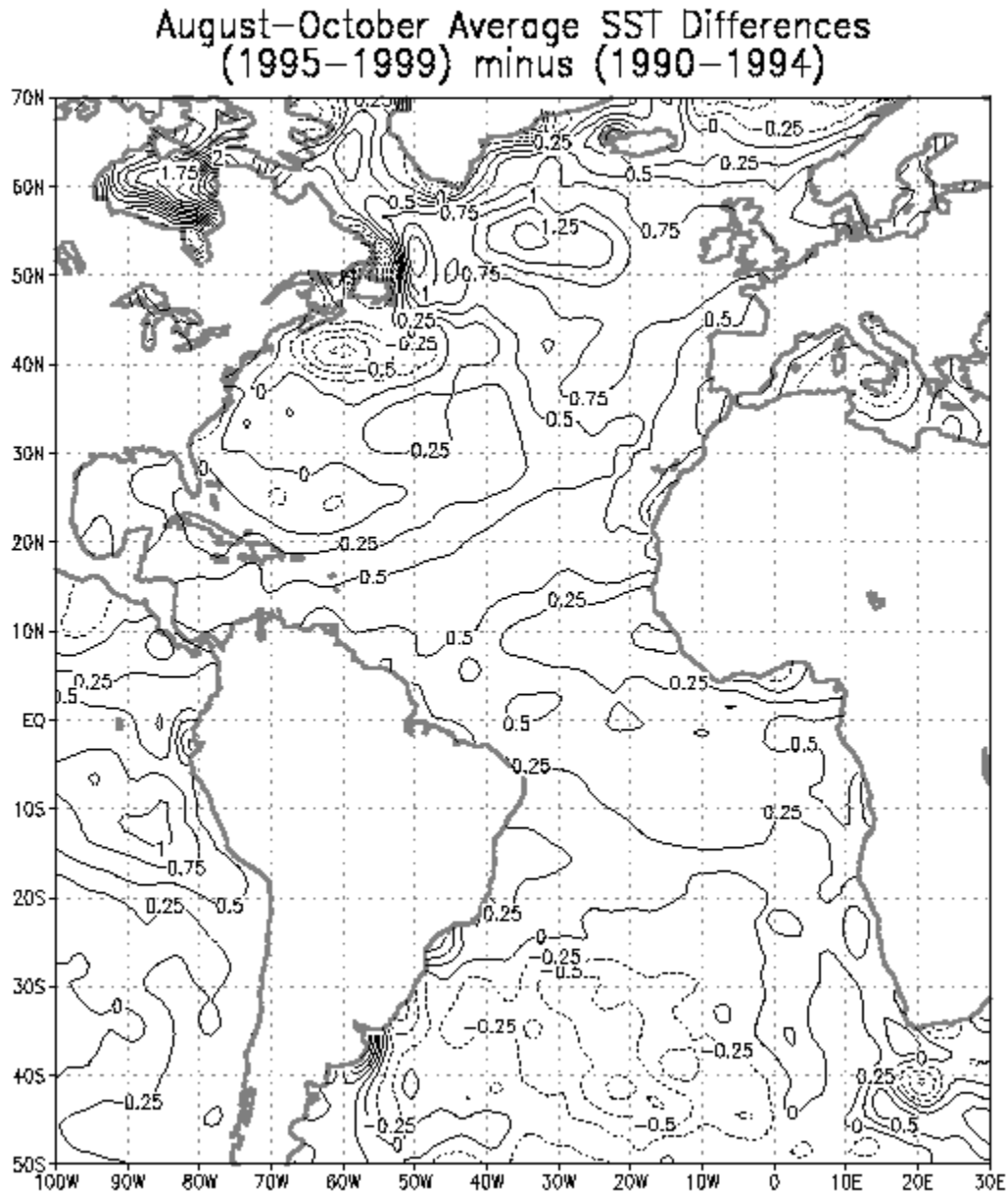
Figure 4: Differences (in °C) for August through October SST between the five-year periods 1995 to 1999 minus 1990 to 1994. Warm (positive) differences are analyzed with solid contours.
