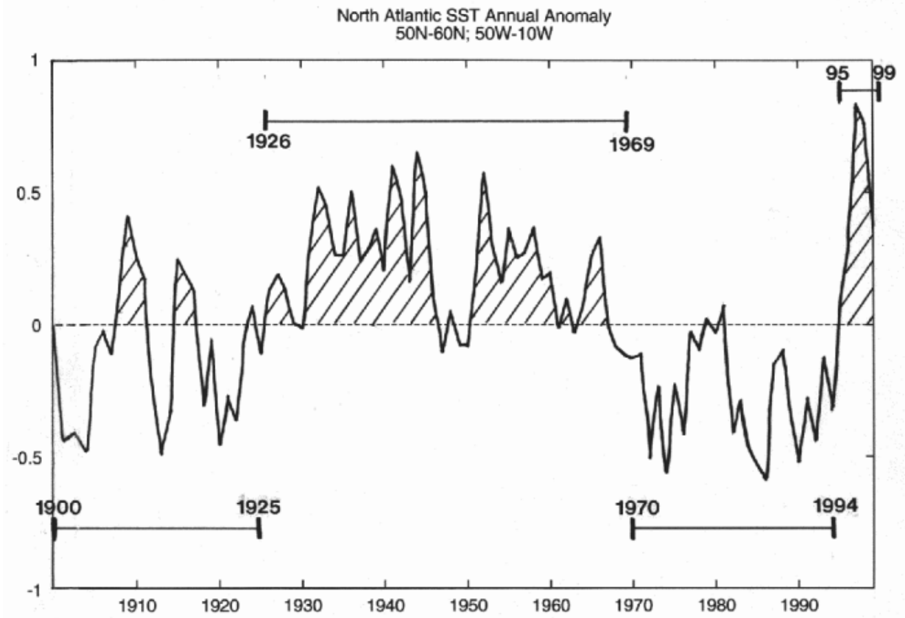
Figure 8: Time series of North Atlantic annual average SST anomalies (in °C) in the area between 50-60°N, 10-50°W for 1900 to 1999. The periods of positive SST anomalies are hatched.
