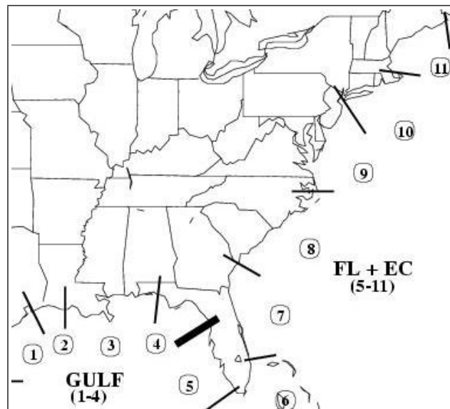
Figure 8: Location of the 11 coastal regions for which separate hurricane landfall probability estimates are made.
