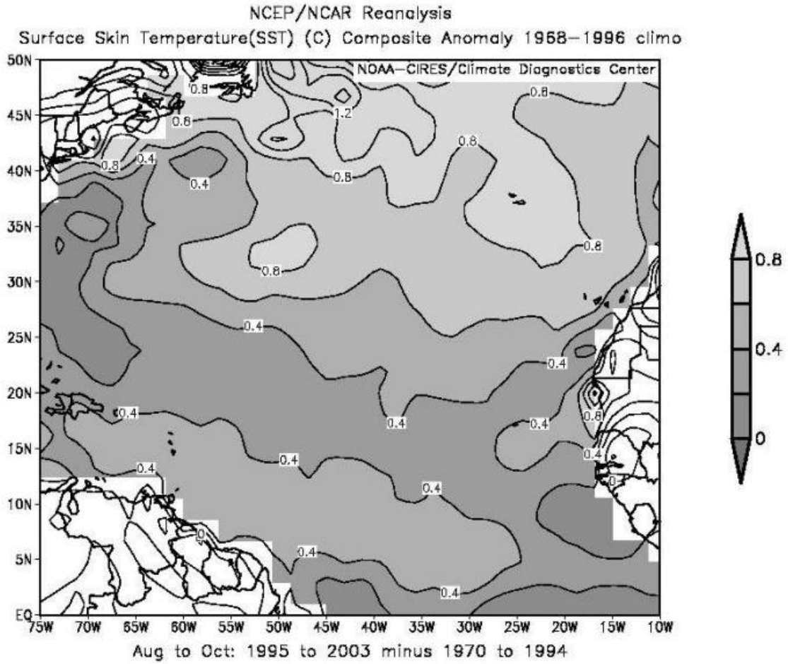
Figure 10: Increase of August-October SSTA (in °C) during 1995-2003 in comparison with the previous 25-year period of 1970-1994.
