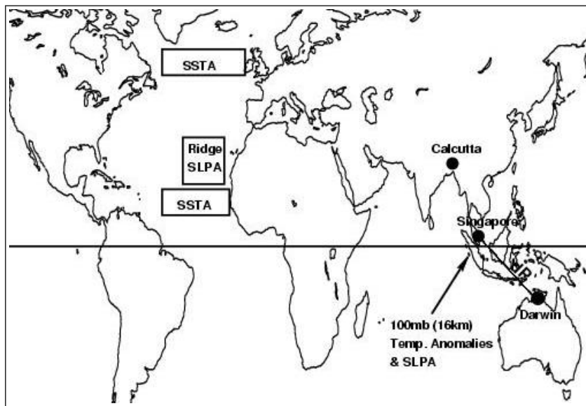
Figure 2: Additional predictor locations which are also considered in formulating our Atlantic seasonal hurricane forecasts.
