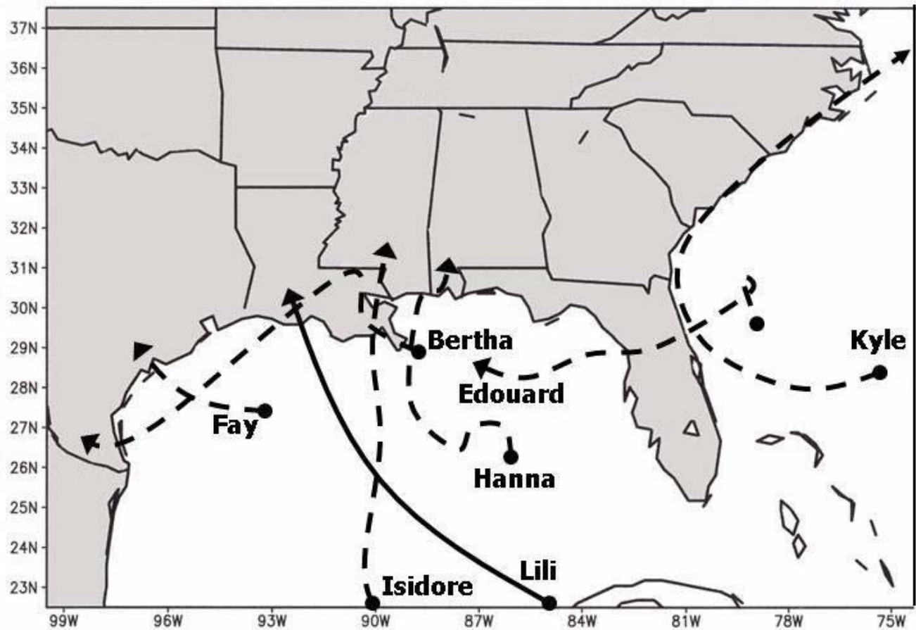
Figure 5: All 2002 U.S. landfalling tropical cyclones.
