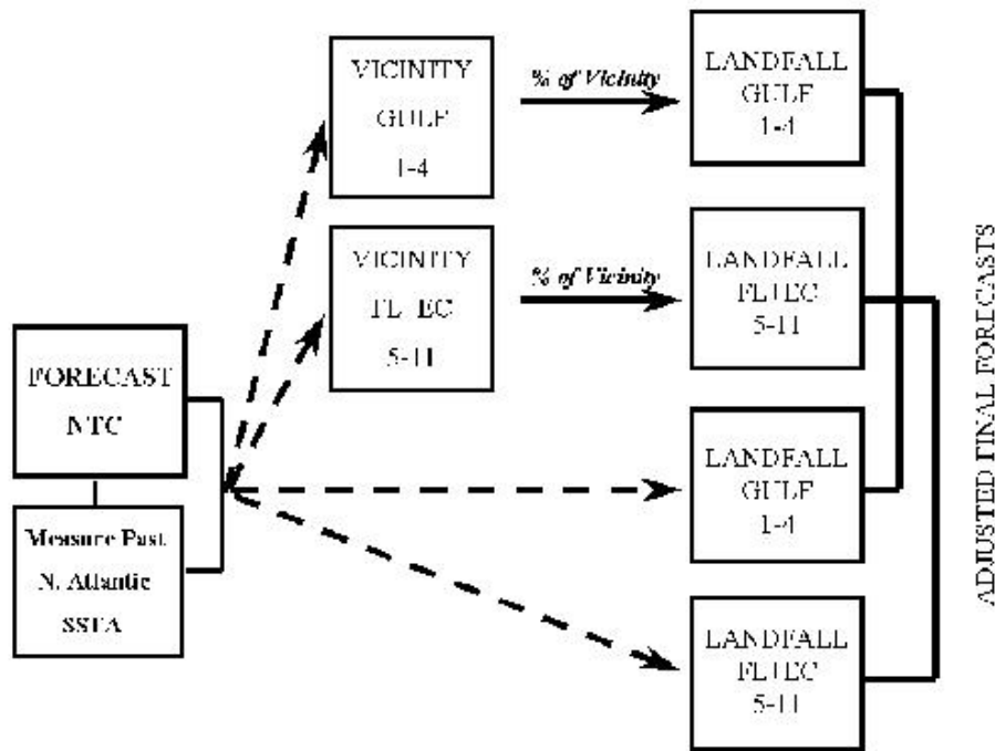
Figure 11: General flow diagram illustrating how forecasts of U.S. hurricane landfall probability are made. We forecast NTC and use an observed measure of the last few years of North Atlantic (50-60° N, 10° -50° W) SSTA*. Regression equations are then developed from the combination of forecast NTC and
