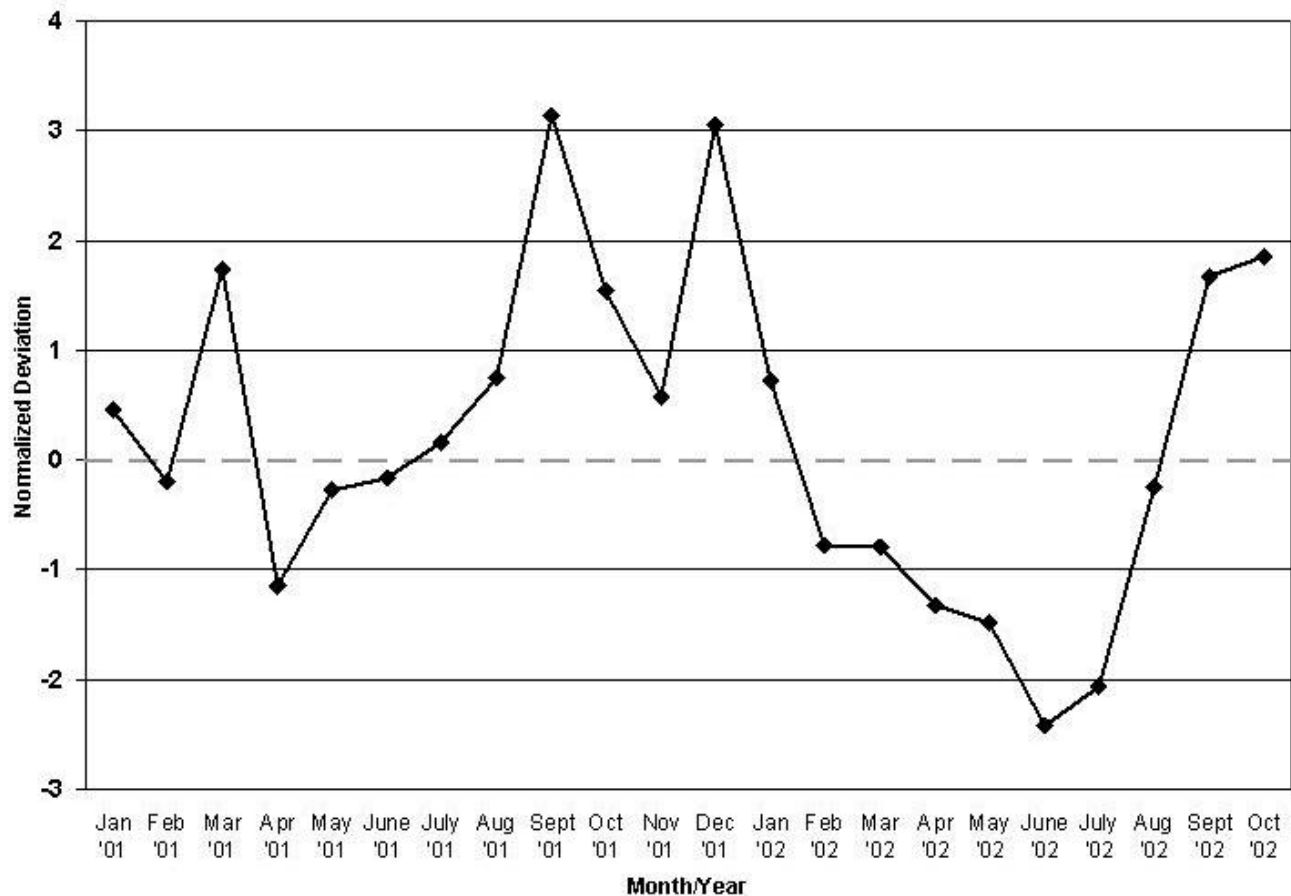
Figure 8: Normalized values of Atlantic SSTA minus SLPA monthly averages from January 2001 through October 2002. SSTA has been averaged from the Equator to 70°N, 20-60°W and SLPA from the
