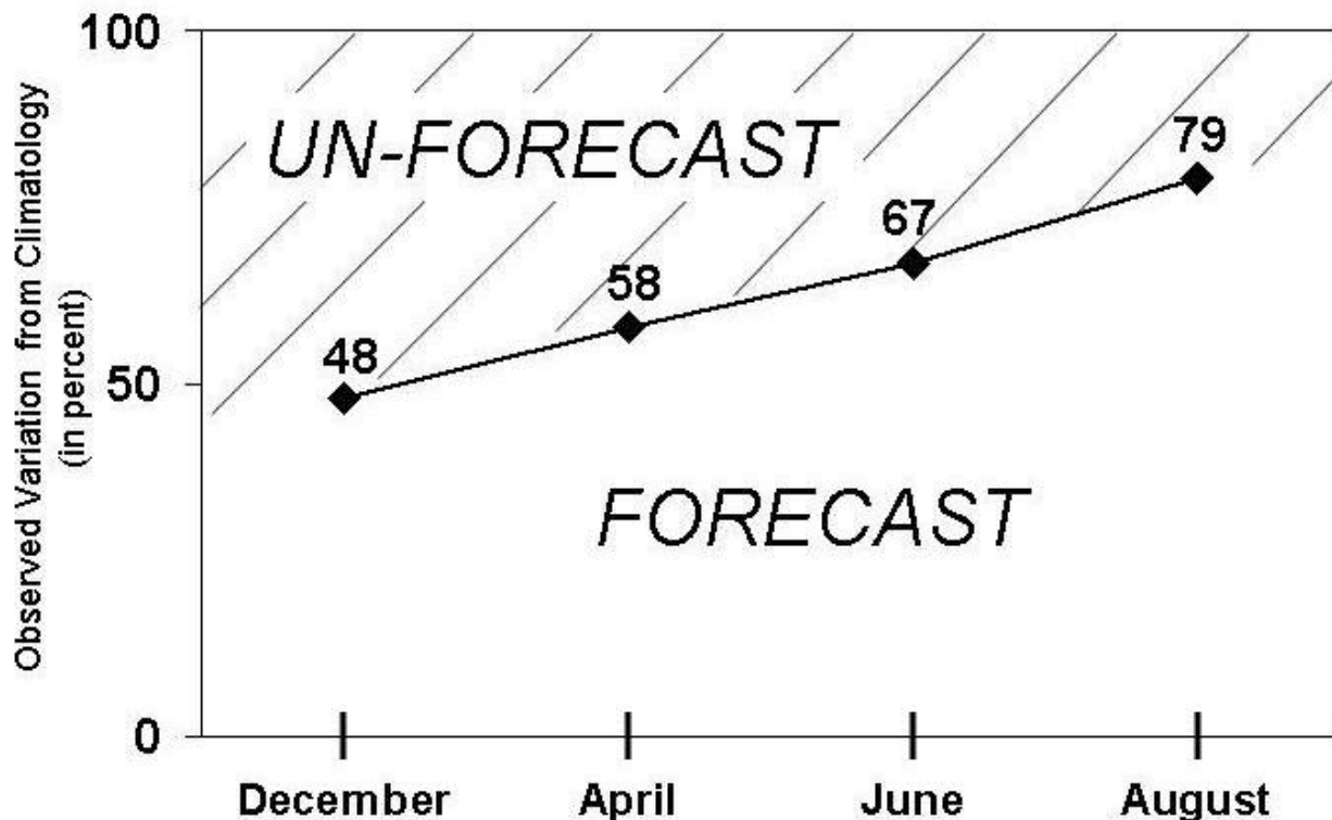
Figure 6: Last four-year average percent of Net Tropical Cyclone (NTC) activity which was forecast at the four individual lead times of early December, early April, early June and early August.
