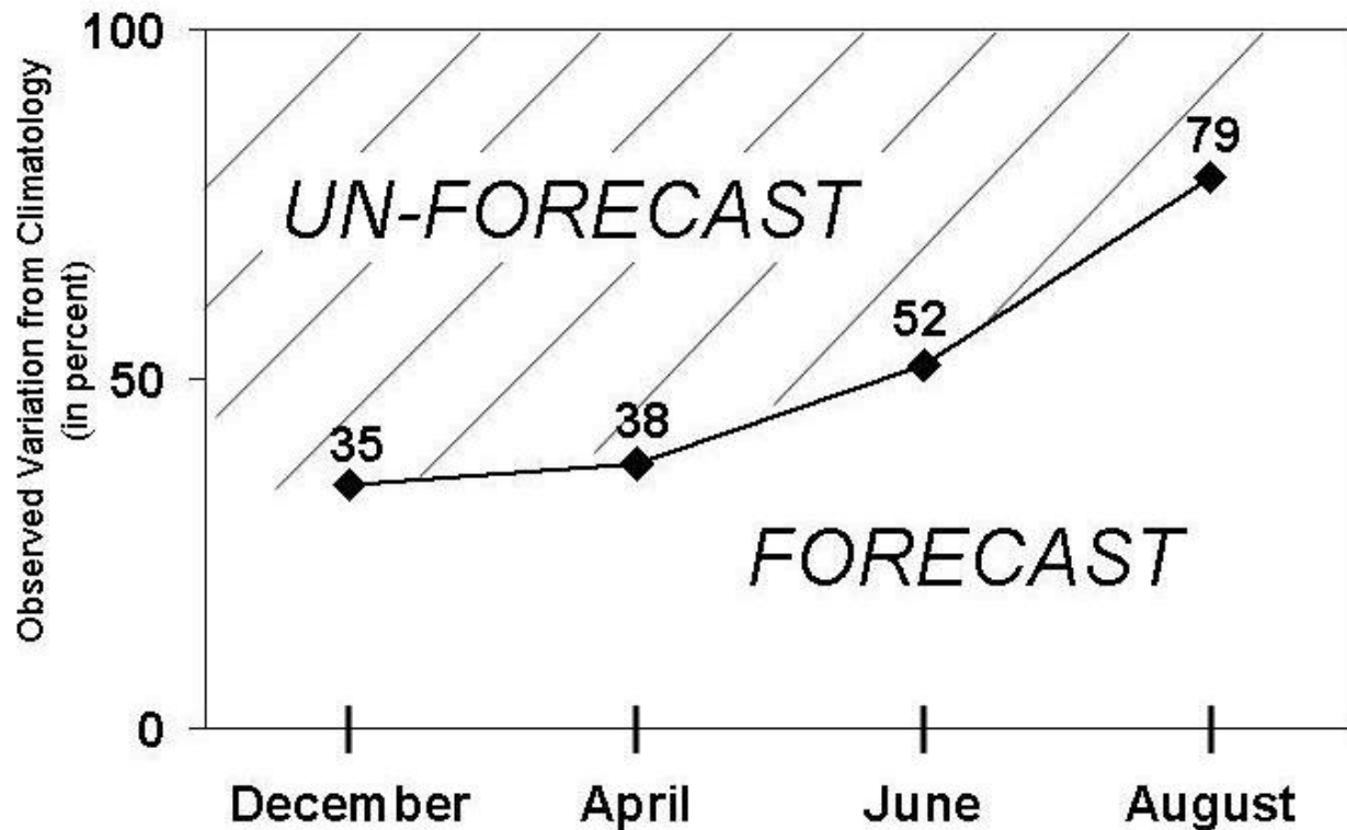
Figure 7: Last four-year average percent of Hurricane Destruction Potential (HDP) which was forecast at the four individual lead times of early December, early April, early June and early August.
