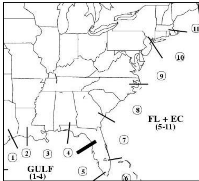
Figure 10: Location of the 11 coastal regions for which separate hurricane landfall probability estimates are made.
