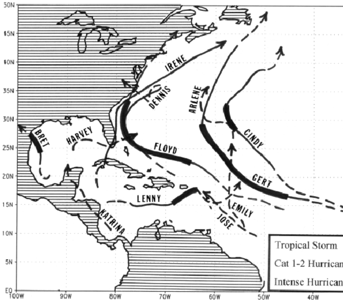
Figure 4: Tracks of the 12 named tropical cyclones of 1999. Dashed lines indicate the tropical storm intensity stage, thin solid lines indicate the Saffir/Simpson hurricane category 1-2 stage, and the thick lines show the intense (or major) hurricane category 3-4-5 hurricane stage.
