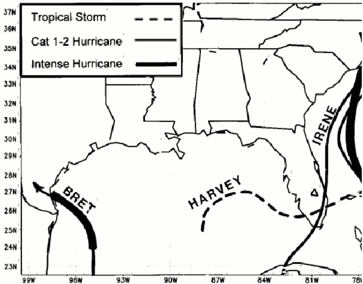
Figure 5: All 1999 U.S. landfalling tropical cyclones by intensity class.
