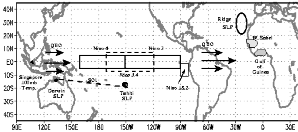
Figure 1: Meteorological parameters used in our various seasonal forecasts.
