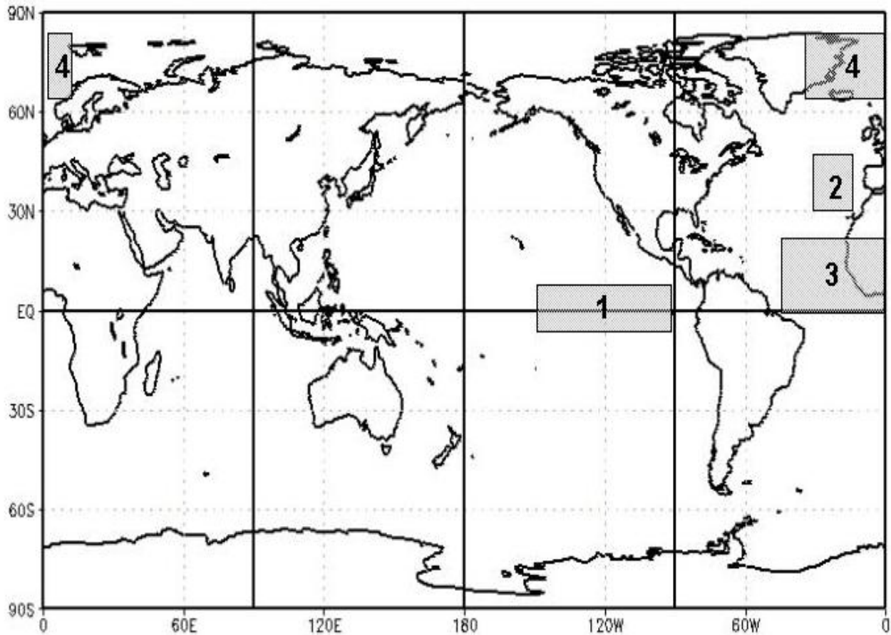
Figure 1: Location of predictors for our new 1 June forecast for the 2005 hurricane season.
