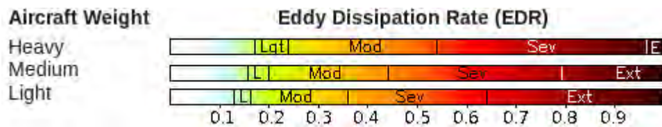
Figure 7. EDR thresholds by aircraft weight class.
