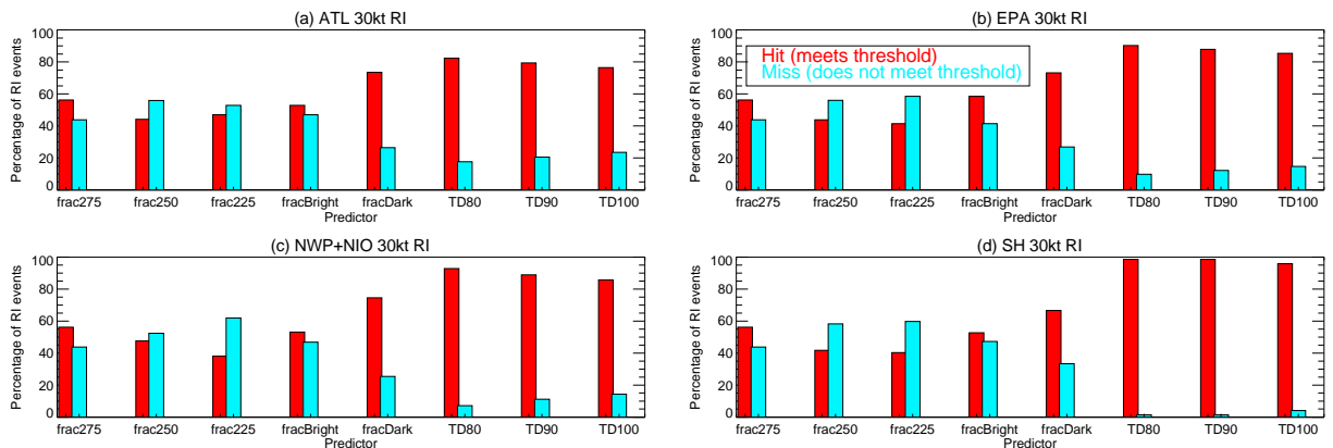
Figure 3b: Same as Figure 2b, except for the SSMIS developmental dataset
