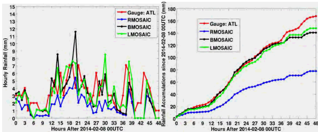
Figure 3. Sample rainfall observations at gauge ATL. (left) time series of hourly rainfall (right) rainfall accumulations.
