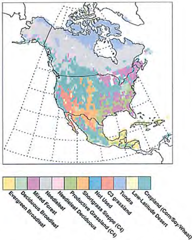
Figure 1: Model domain, showing vegetation type
