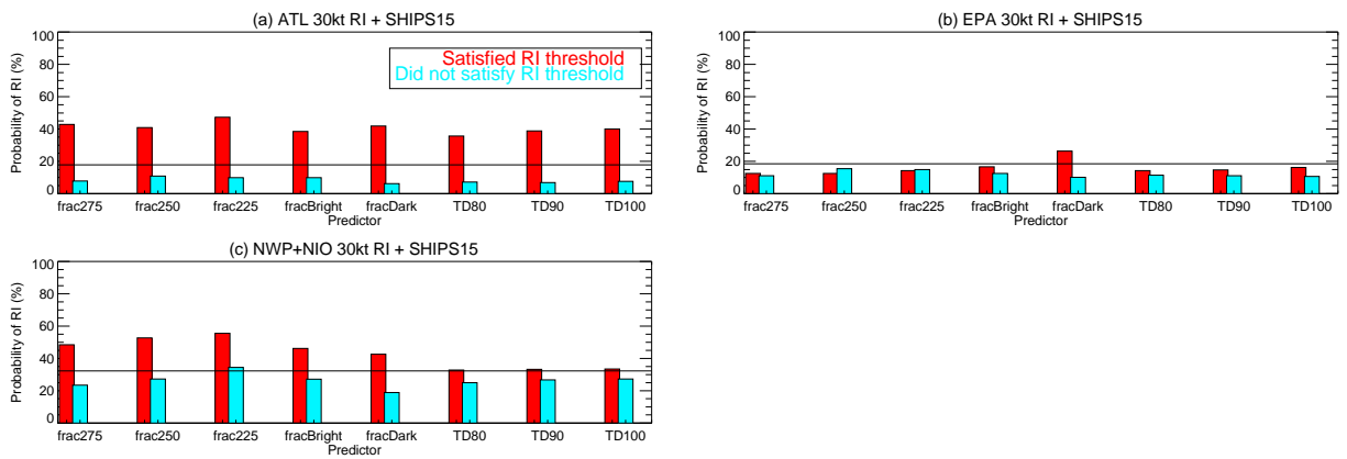
Figure 3c: Same as Figure 2c, except for the SSMIS developmental dataset
