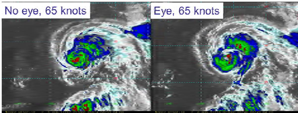
Figure 4. West Pacific case showing an eye/no-eye example, WP122011 MERBOK (65 knots). The image on the left shows a no-eye case 6 hours prior to the image on the right which was subjectively determined to have an eye.
