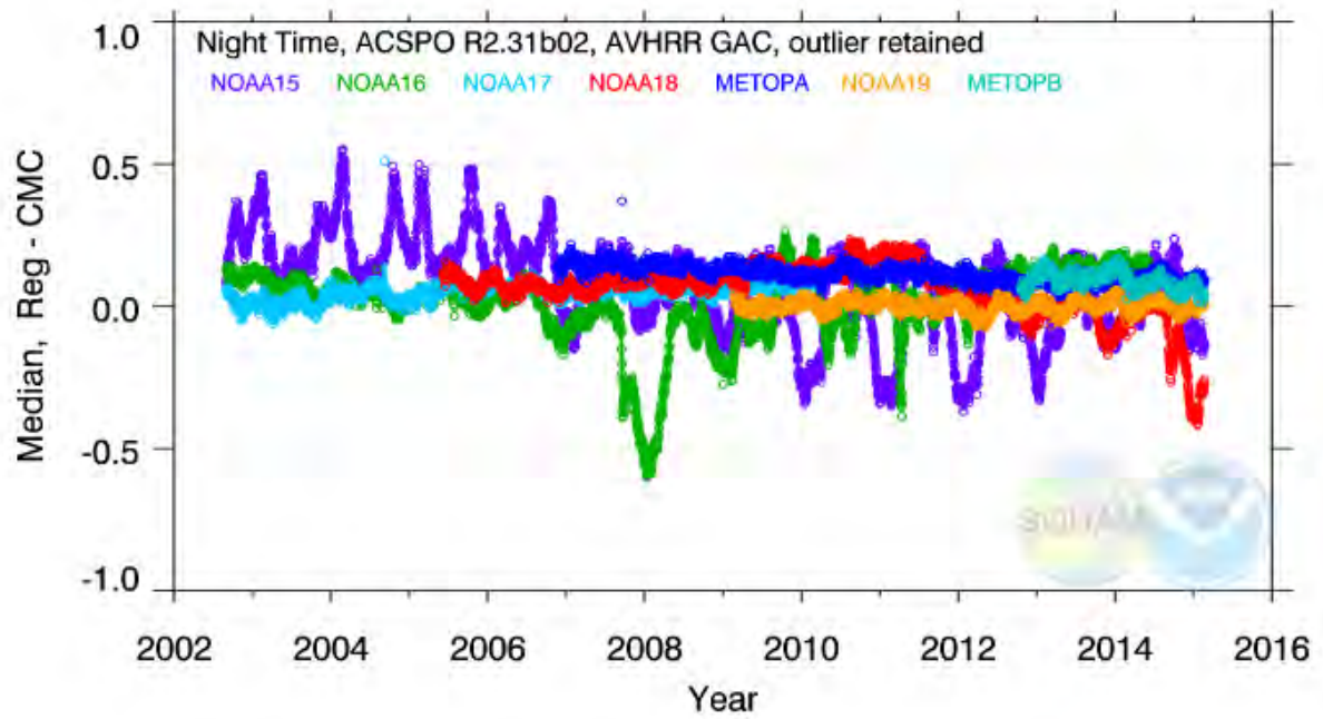
Figure 3. Time series of night time ACSP0 RAN2 AVHRR GAC L2 SST minus CMC L4 SST. Each symbol is one day average bias.
