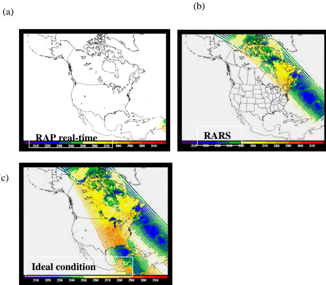
Figure 2. AMSU-A channel 3 brightness temperature from NOAA-19 at 18Z May 29 2012 with \pm 1.5 hour time window for (a) RAP real-time data file (used operationally), (b) RAP RARS file (not used operationally yet), and (c) the ideal condition (no data latency and no cut-off issue).
