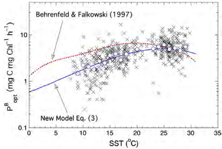
Figure 9. Optimal photosynthetic carbon fixation rate ( P_{opt}^B ) as a function of SST for the Chesapeake Bay.
