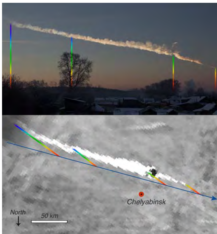
Figure 5. Comparison and triangulation of the Chelyabinsk meteor trail as seen from the ground (top) and from space (bottom) as detailed by CIRA researcher Steve Miller. (Image courtesy of Steve Miller and Maureen Murray.)
