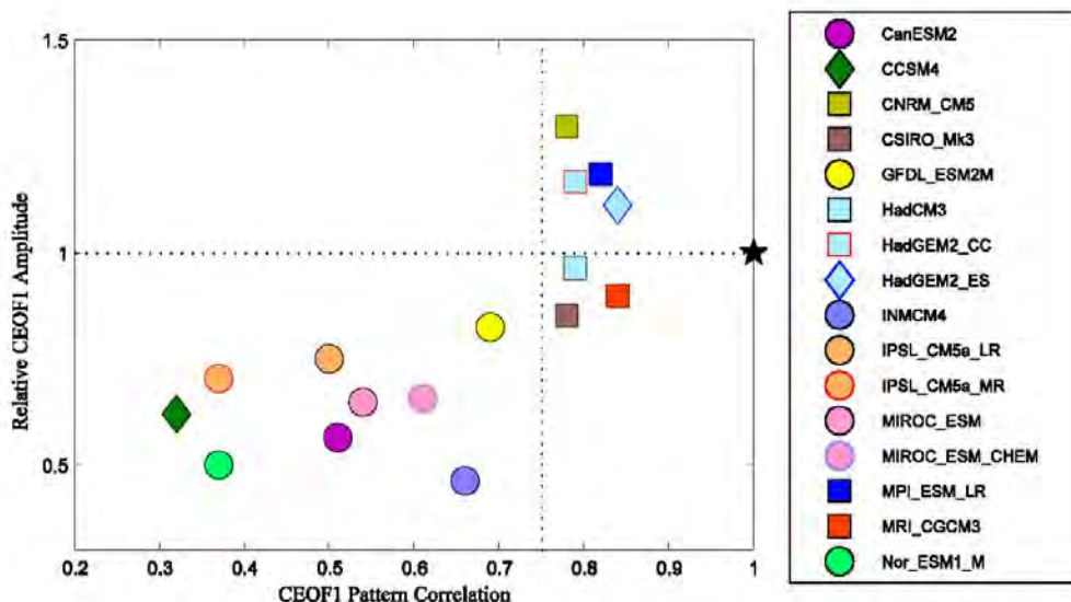
Figure 1. Pattern correlation coefficients of the CEOF1 mode between TRMM observations and CMIP5 GCM simulations. Y-axis: Relative amplitudes of CEOF1 in model simulations to the observed counterpart. Both pattern correlations and amplitudes are derived by averaging over the area of 5°N-25°N, 140°W-80°W where the active ISV is observed. The black “star” mark represents the TRMM observations. Models with “square” marks display westerly or weak easterly (<1.5 m s -1 ) summer mean wind at 850hPa, while strong easterly winds (> 4 m s -1 ) are noted in models with “circle” marks. Wind fields are not available in the data portal at the time of this analysis from the two GCMs with “diamond” marks.
