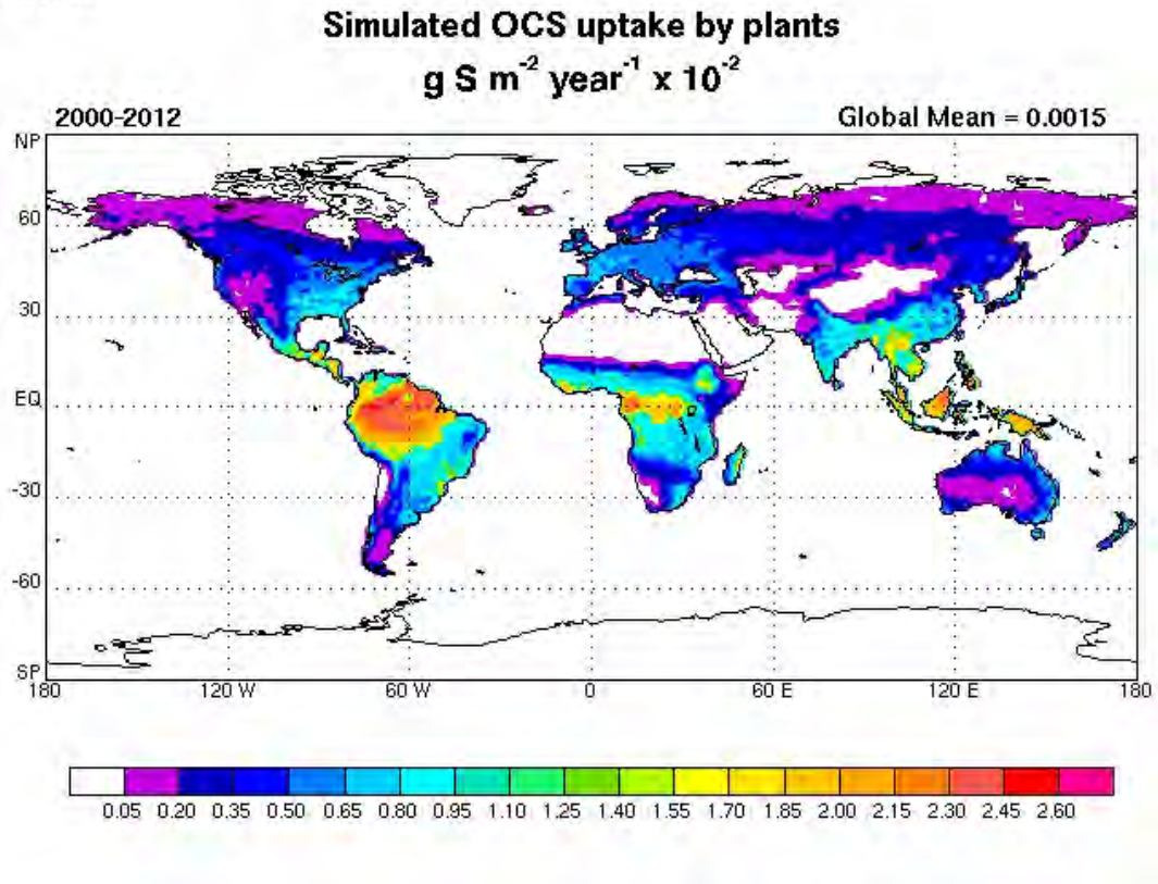
Figure 2. Global mean uptake of OCS by plants ( \text{g S m}^{-2} \text{ year}^{-1} ).
