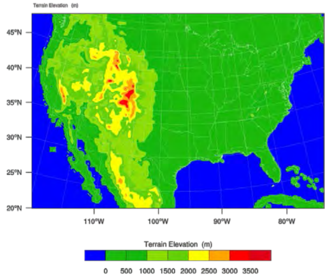
Figure 2. Modeling Domain.
