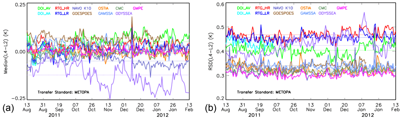
Figure 3. (a) The time series of global median ( \mu_{\Delta\epsilon} ) for \Delta T_{L4L2} , with L2 SST derived from Metop-A GAC data; (b) The time series of global robust standard deviation ( \sigma_{\Delta\epsilon} ) for \Delta T_{L4L2}
