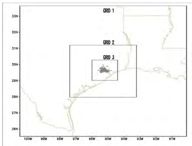
Figure 1. Grid configuration. The center of all grids coincides with the location of the city. The shaded area represents the city of Houston
