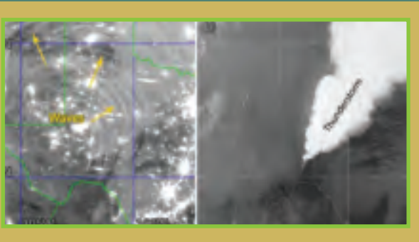
Figure 3. DNB (left) and infrared (right) images of Texas thunderstorm from VIIRS. (credit CIRA)
