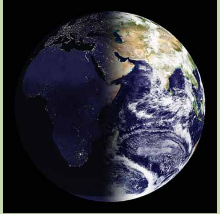
Figure 4. A new animation of the NASA "Blue Marble" image with nighttime lights.
