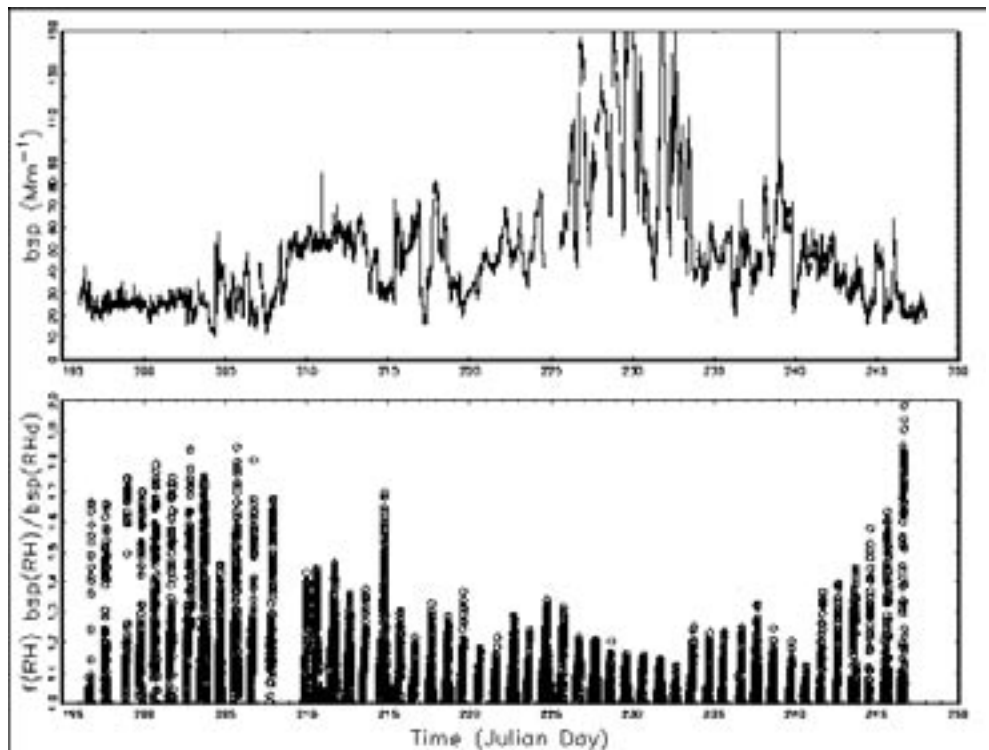
Figure 5, showing the light scattering coefficient (top) and f(RH) functions in time.
