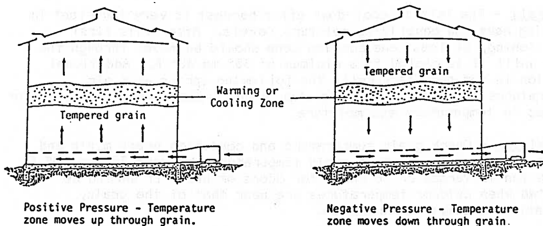
Figure 3. Air Flow Direction Showing Positive and Negative Pressure
