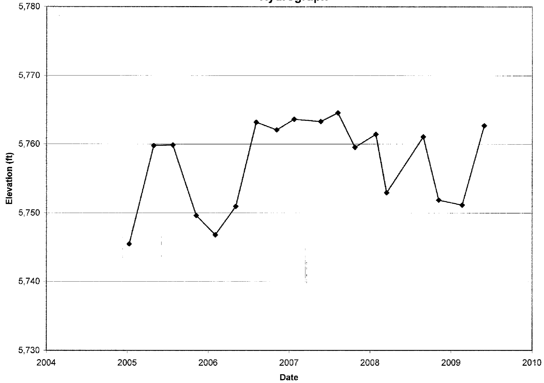
Figure 3 CSRMI-2 Hydrograph
