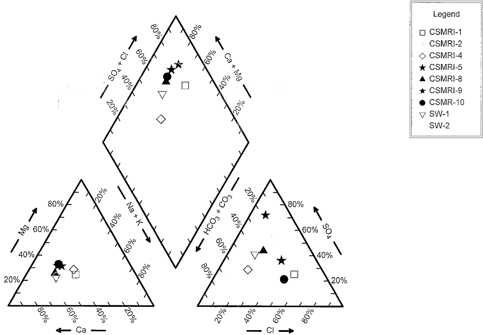
Piper Diagram CSMRI 2009 Quarter 2
