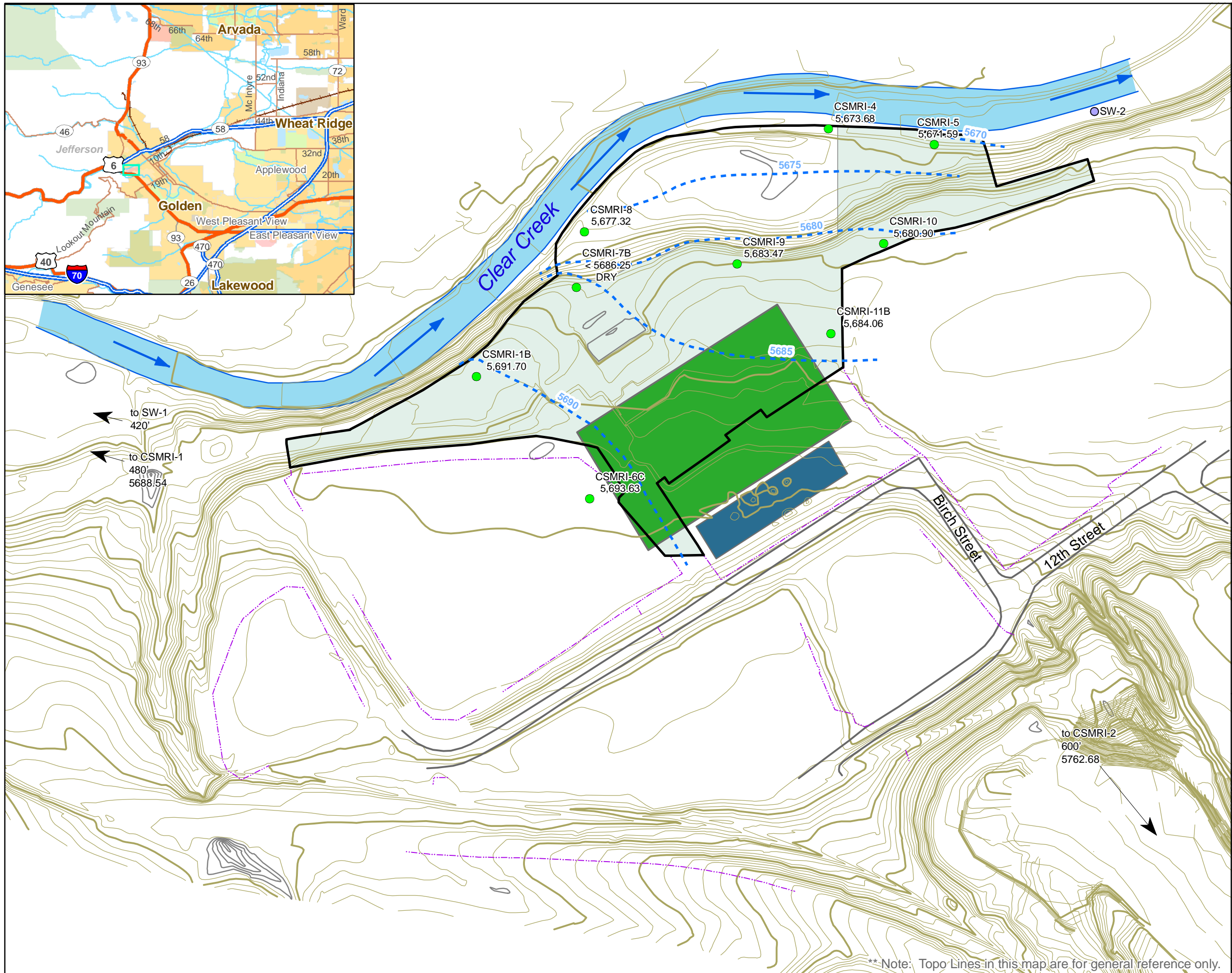
Figure 1 Groundwater Potentiometric Elevation Map - June 2009
