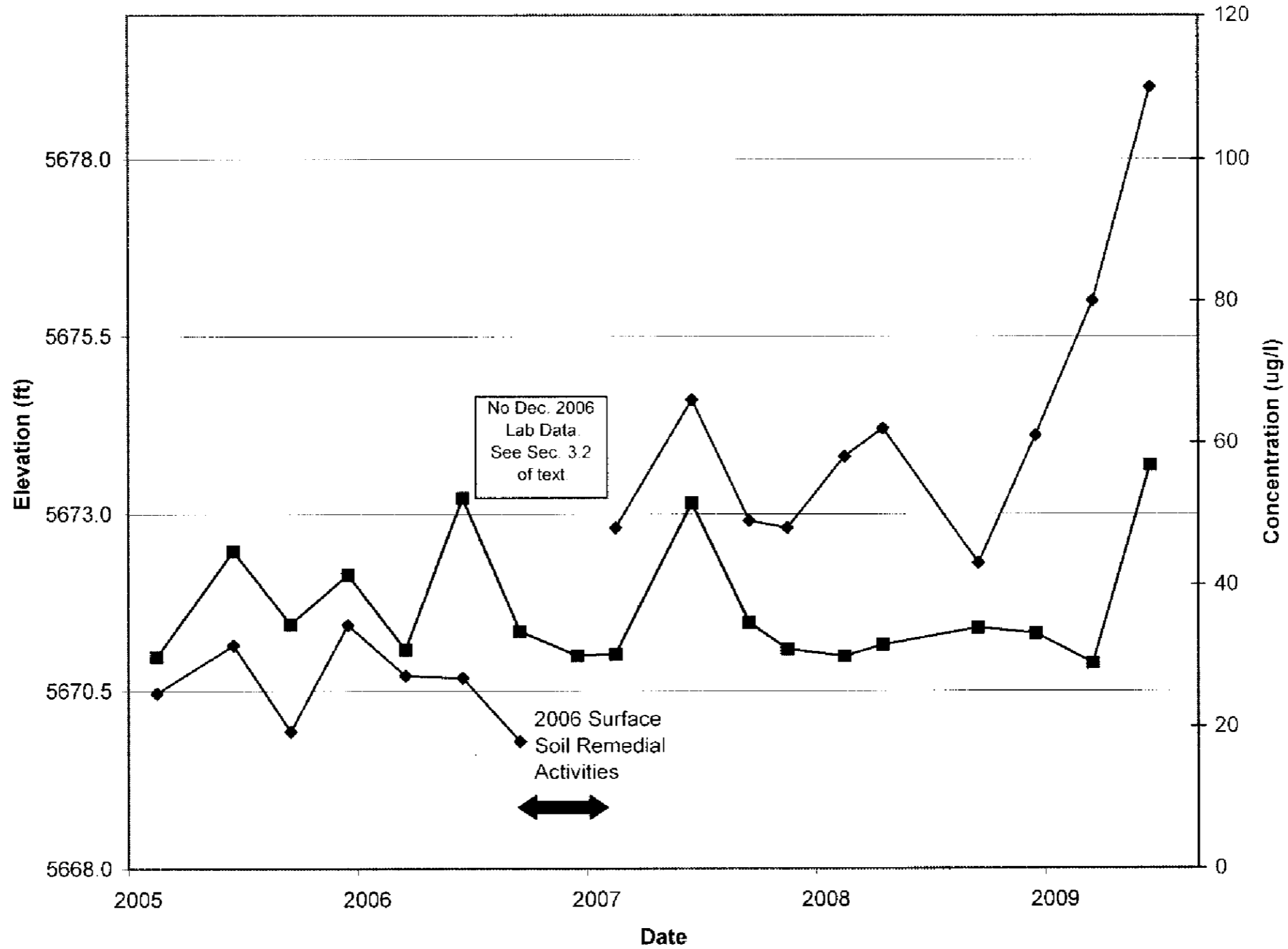
Figure 6 CSMRI-4 Total Uranium Concentration and Potentiometric Elevation
