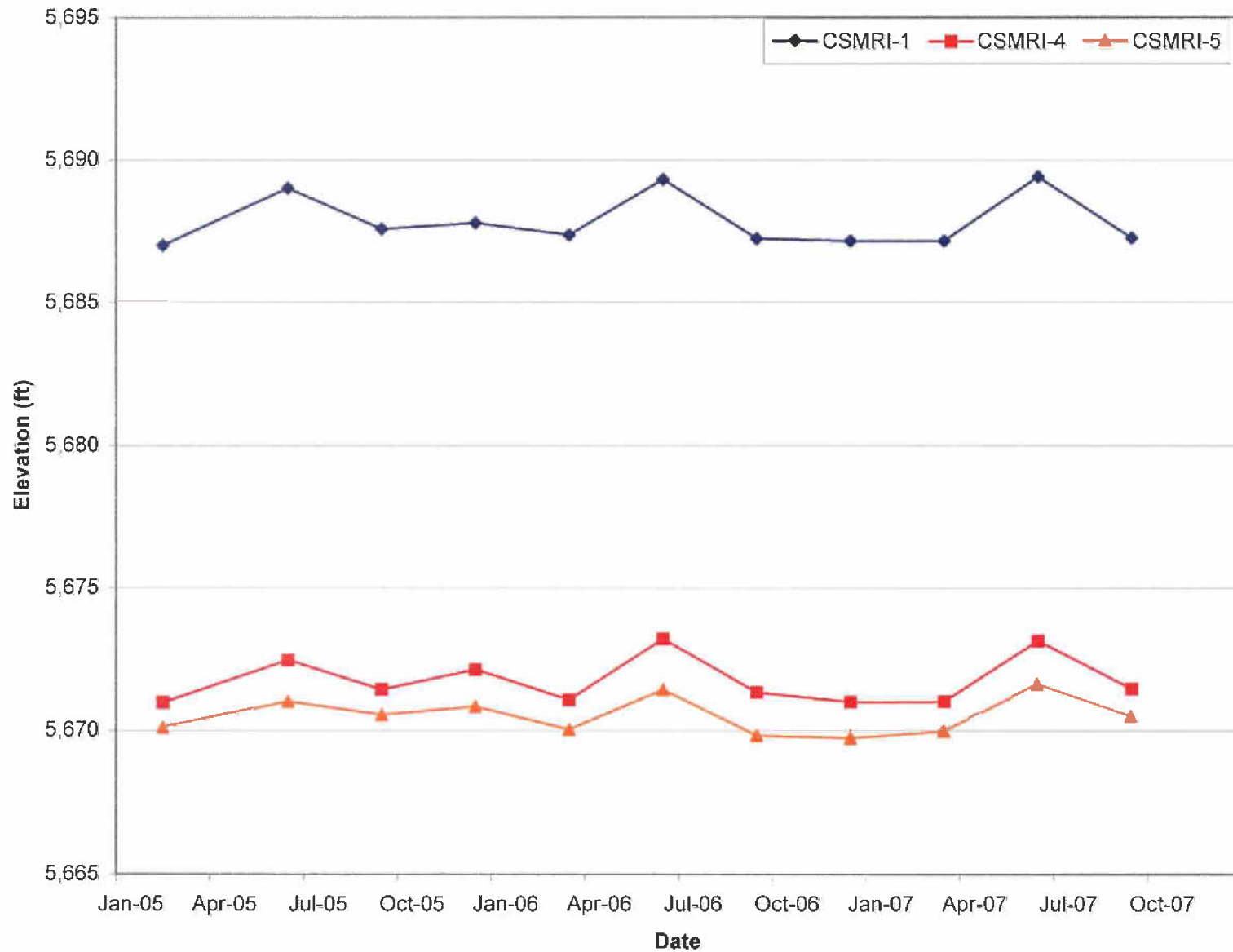
Figure 2 Hydrographs CSMRI-1, CSMRI-4 and CSMRI-5
