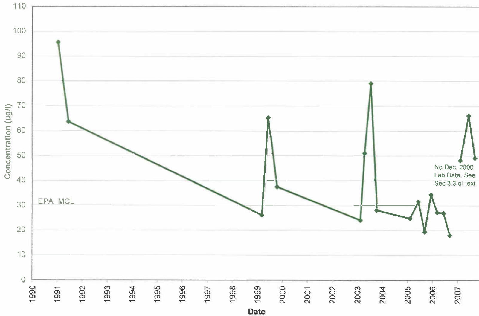
Figure 5 CSMRI-4 Historical Total Uranium Concentration
