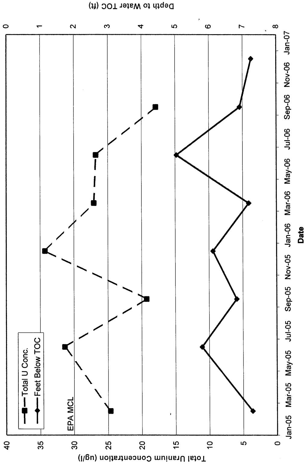
Figure 6 CSMRI-4 Total Uranium Concentration
