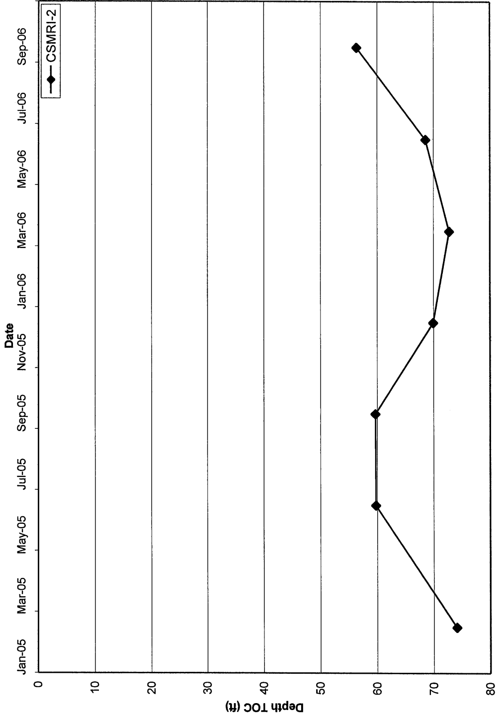
Figure 3 Hydrograph CSMRI-2
