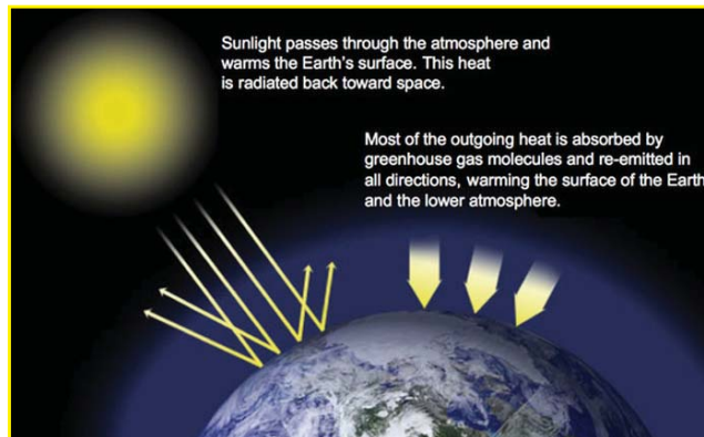
Figure 1: A simple demonstration showing how excess CO 2 can cause global warming. (www.nasa.gov)
