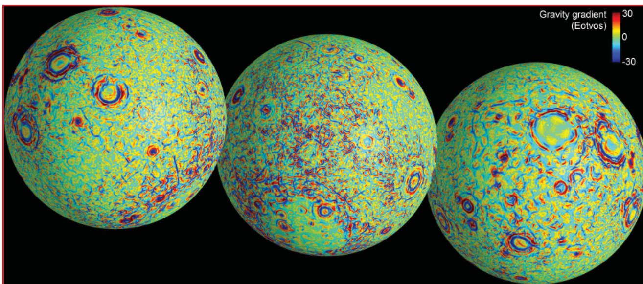
Globes of different orientations showing the Bouguer gravity gradient data [Andrews-Hanna et al., Science, 2013].
