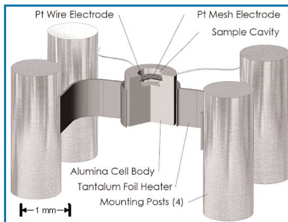
Figure 4.4 (5). Preliminary design for the miniaturized electrochemical cell for use in the TIMS (courtesy of Don David, CIRES). Mounting posts are the filament posts currently used in the mass spectrometer.
