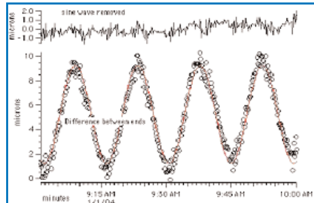
Figure 4.4 (1). 2\text{-}\mu\text{m} peak-to-peak signal caused by the dynamics of the piston/stepper drive system
