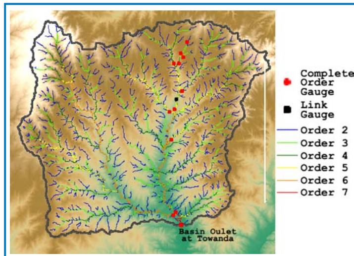
Figure 4.1 (8). Locations of the planned stream flow gauges.
