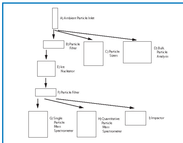
Figure 3.6.3 (1). Schematic diagram of the experimental apparatus used in the INSPECT2 study. Particles are sampled through the inlet system (A) followed by a filter that removes any large (supermicron) particles so that large ambient particles will not be confused with nucleated ice particles. Commercial particle sizing instruments (C) and bulk particle samplers (D) are used to put the measurements in context with previous data sets. The Continuous Flow Diffusion Chamber (CFDC, item E) nucleates ice particles on a fraction of the ambient aerosols, depending on operating conditions. The Laboratory Counterflow Virtual Impactor (LCVI, item F) acts as another particle filter, removing all the un-nucleated small particles, allowing analysis of just those particles that nucleated ice. Analysis of the ice nuclei is performed in real time with the Particle Analysis by Laser Mass Spectrometry (PALMS) instrument (G) and the Aerosol Mass Spectrometer (AMS, item H). Collection on an impactor (item I) allows ice nuclei to also be analyzed later using standard laboratory methods.
