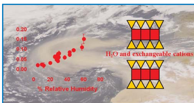
Figure 4.1 (21). Schematic of montmorillonite clay and water content of clay vs. RH overlaid on a photo of atmospheric dust off of the African coast.
