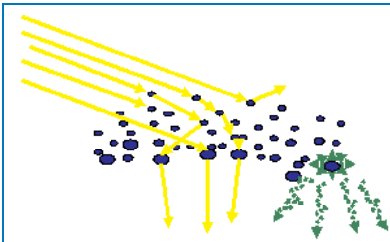
Figure 4.5 (8). Schematic displaying the radiative properties of liquid within a cloud. Yellow lines show the near-infrared absorption photon path, and the green is illustrative of the microwave emission of all of the liquid water molecules. The microwave emission signal is dependent upon the amount of water in the column and essentially independent of size of the particles. The near-infrared absorption signal is dependent upon the amount of water in the column and the photon path length. The photon path length depends on the size of the particles; a higher number of small particles increases the path length.
