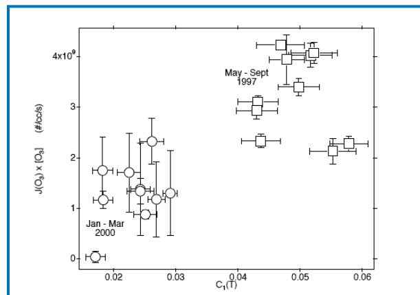
Figure 3.2.4 (1). Scatter plot showing the correlation between photodissociation of ozone and intermittency of temperature in the lower stratosphere. The data are from the POLARIS and SOLVE campaigns.
