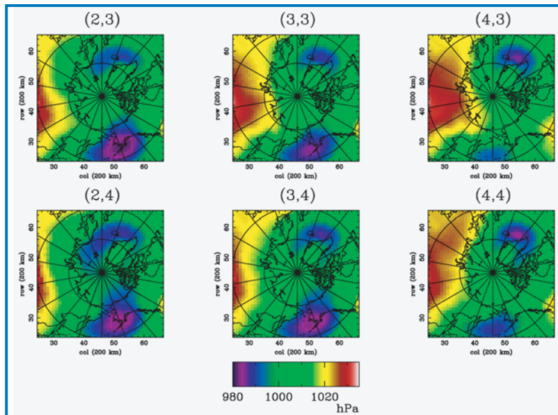
Figure 4.1 (4). Six of the 35 synoptic weather patterns identified using the SOM algorithm. Color shading indicates sea level pressure.
