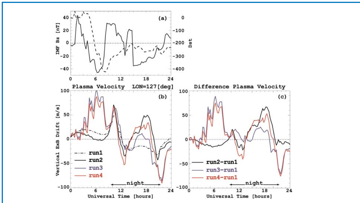
Figure 3.1.16 (3). (a) GSM z-component of the interplanetary magnetic field (IMF) measured by SWEPAM and MAG instruments on board the ACE spacecraft (time-shifted to the sub-solar magnetopause location) shown by solid line, and the Dst (SYM-H) index plotted by dash line, for March 31, 2001. (b) An example of the vertical ExB drifts at the magnetic equator obtained from CTIPe, at 127 degree longitude. At this longitude sector, 00 UT corresponds to 8.47 LT. Four different CTIPe simulations are shown. The black dash line is the quiet time reference (run1). The black solid line is the simulation with DD effect only (run2). The blue solid line is the simulation with the DP electric field only (run3). The red solid line is the simulation including both effects of the DD and DP electric fields (run4). (c) Same as (b), but the changes in the drifts from the quiet time (run1).
