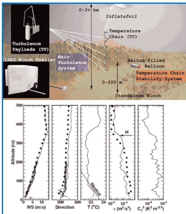
Figure 4.4 (6). Top: Diagram of proposed field deployment of the new CIRES TLS during the T-Rex experiment (proposed April-May 2006). Bottom: CIRES TLS in situ validation of doppler lidar remote-sensing turbulence data over the Pentagon in Washington, D.C. (May 2004). Solid lines represent TLS data, black circles are Lidar profiles, and open circles are sodar data.
