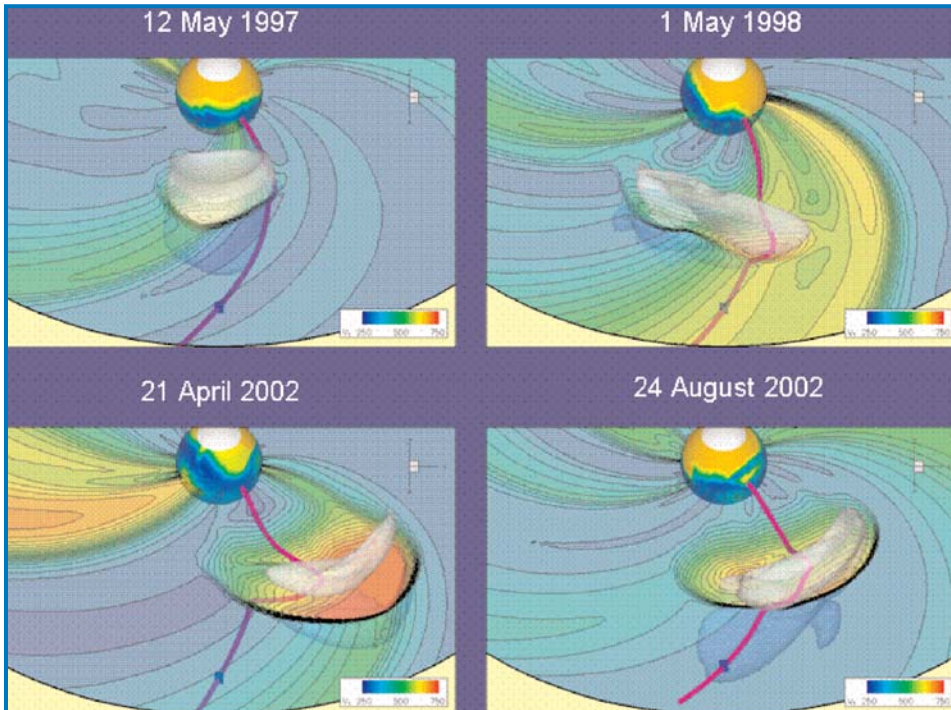
Figure 3.1.15 (5). Heliospheric disturbances during four solar events.
