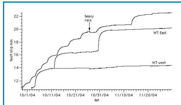
Figure 4.1 (3). Surface afterslip near the Parkfield epicenter, as recorded by creep meters.
