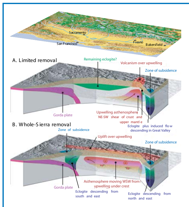
Fig. 4.1 (9). Competing explanations in the Sierra: localized lithospheric foundering with minimal implications (center) and widespread foundering with widespread consequences (bottom).
