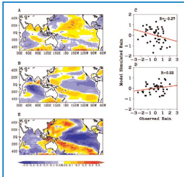
Figure 4.5 (2). Correlation maps of (a) observed SSTs and monsoon rainfall simulated from uncoupled NCAR-CCM3 (GOGA) model, (b) simulated SSTs and monsoon rainfall from the coupled (MLM) model. Scatter plots of standardized anomalies of observed and simulated monsoon rainfall for each year during 1950–1994 from GOGA and MLM are shown in (c) and (d), respectively. Correlation map of (e) observed SSTs and observed monsoon rainfall.
