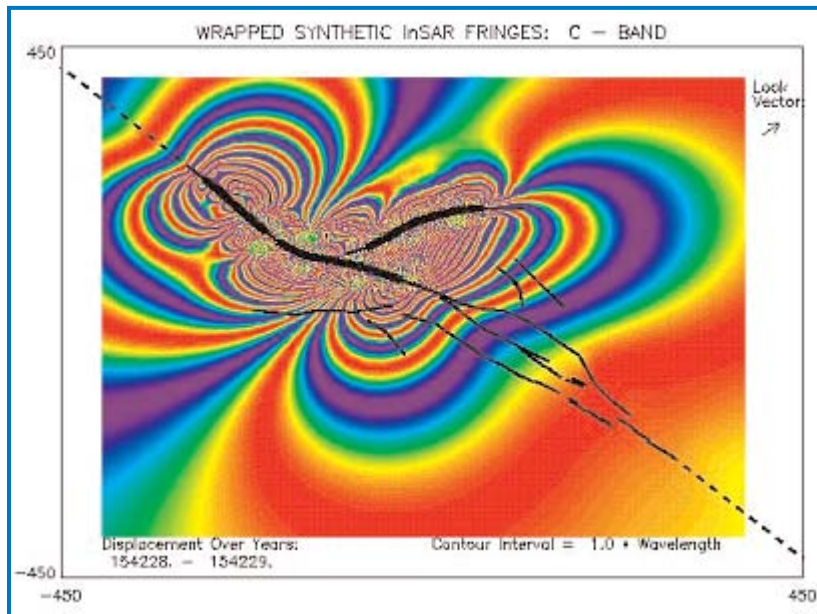
Figure 4.5 (6). Surface deformation as recorded by SAR Interferometry.
