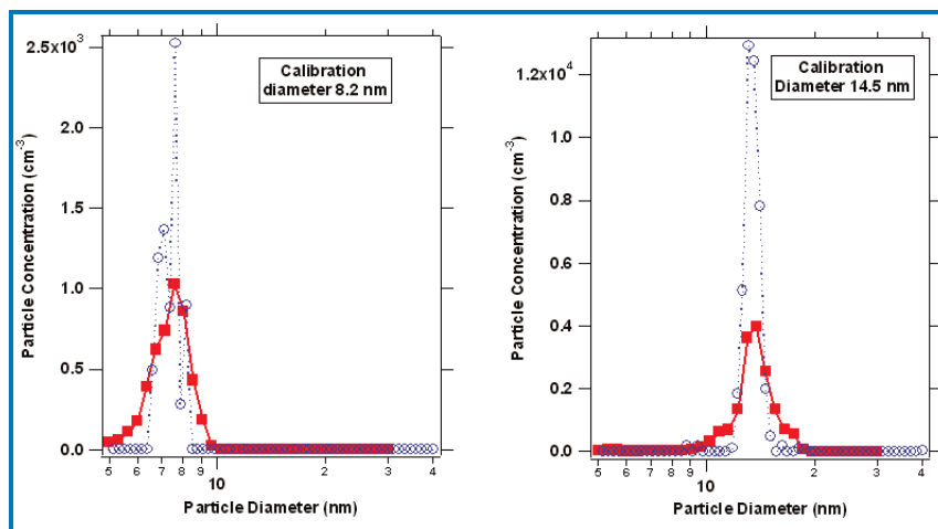
Figure 4.4 (4) Comparison of measurements of two monodisperse calibration aerosols measured simultaneously with the SCoPS (closed symbols) and with an existing technique, the scanning mobility particle sizer (open symbols). The SCoPS measured concentration more accurately and was faster, less expensive to construct, and simpler to operate.
