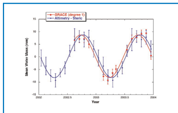
Figure 4.1 (14). GRACE ocean mass estimates compared with satellite altimetry measurements.
