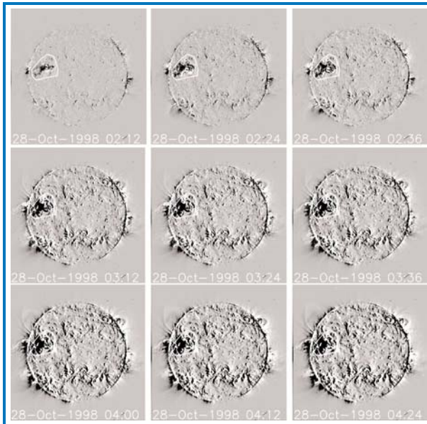
Figure 3.1.15 (4). EUV dimming (upper left quadrant) associated with solar eruption.
