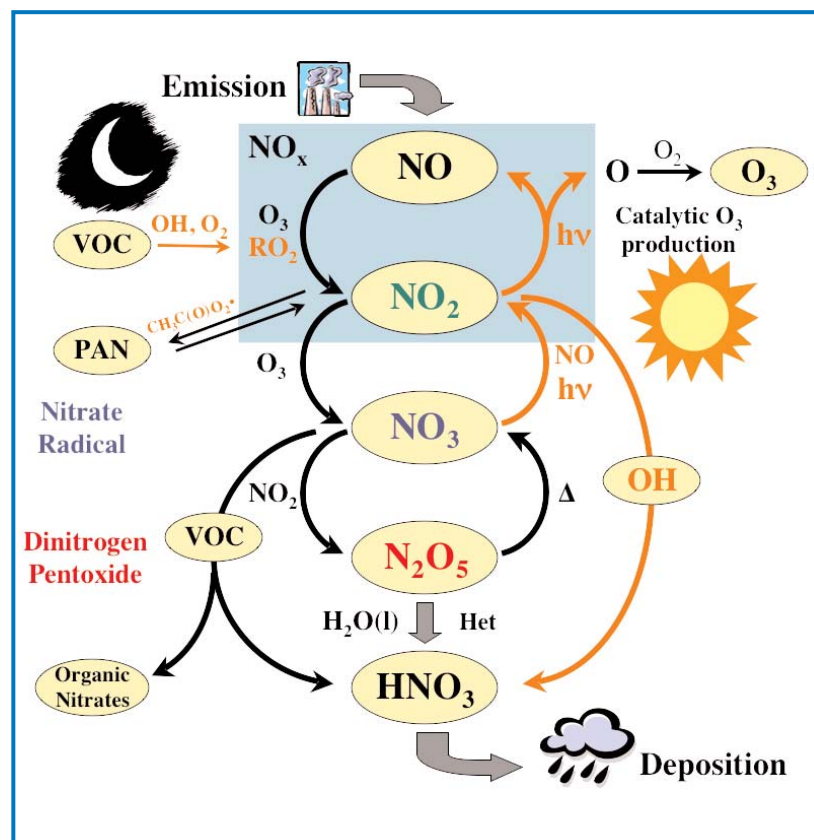
Figure 3.1.1 (1). Nitrogen oxide cycle in the lower atmosphere, showing “dark reactions.”
