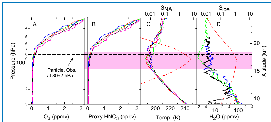
Figure 3.2.1 (1). Vertical profiles of ozone (A), proxy nitric acid (B), temperature (C), and water vapor (D) from balloon-sonde measurements in the deep tropics. The purple region represents the altitude range favorable for the growth of NAT particles ( SNAT > 1 ), calculated using the median values of nitric acid, temperature and water vapor.
