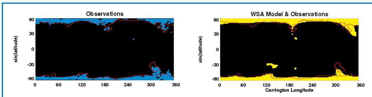
Fig. 3.1.15 (1) and d. Coronal Hole Synoptic Maps.
