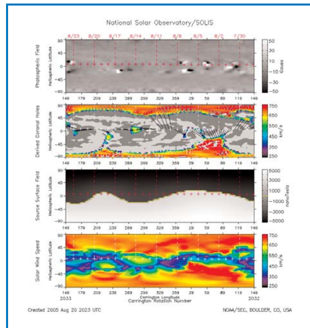
Figure 3.1.15 (3). Plots of output from newly improved and streamlined Wang-Sheeley-Arge model.
