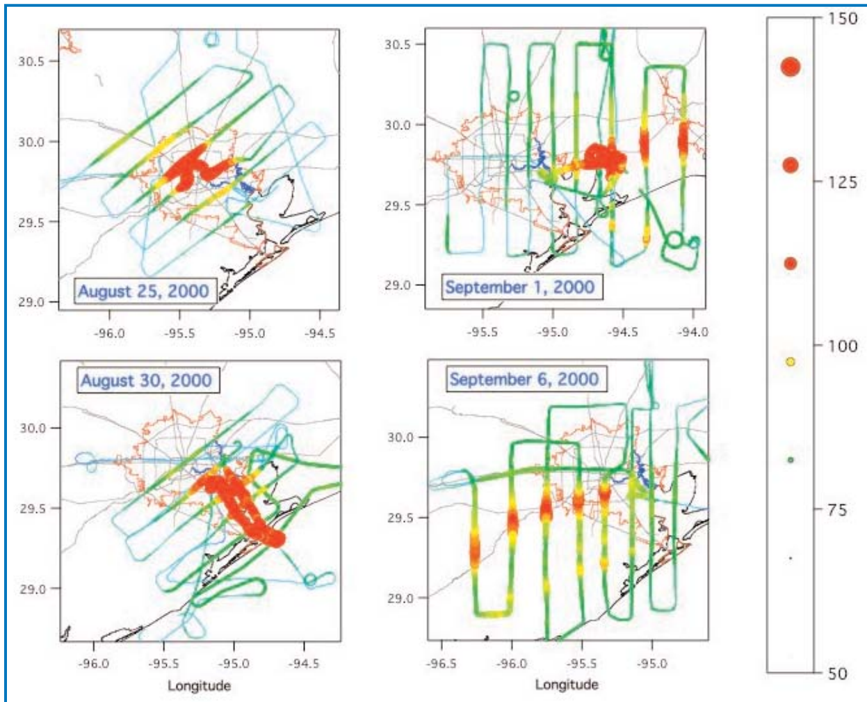
Figure 3.6.2 (2). Airborne measurements on four days characterized by substantially different meteorological conditions show the ability of petrochemical alkene emissions to routinely form extremely unhealthy amounts of ozone. Flight tracks are shown colored and sized by ozone. High ozone levels are only found downwind of the petrochemical source regions; in contrast, emissions from the urban center and the isolated power plant do not form nearly as much ozone.
