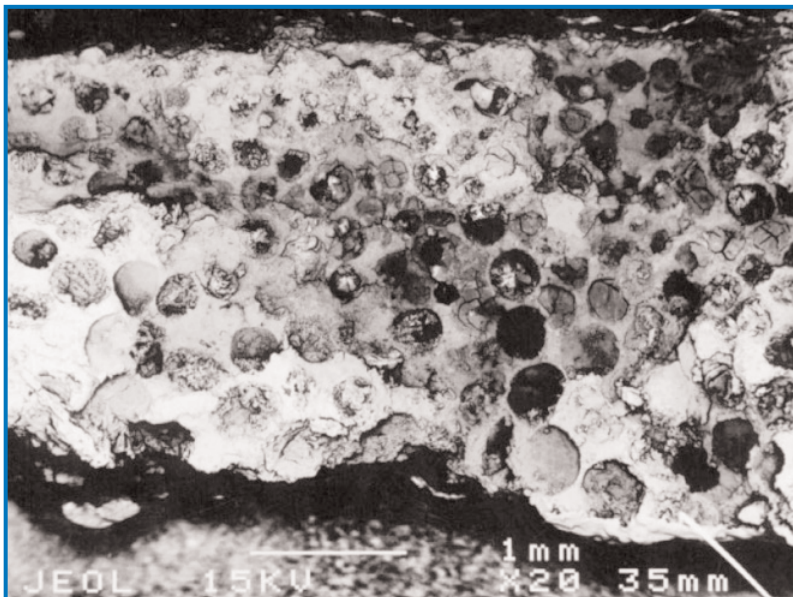
Figure 4.1 (17). Silicate spherules condensed from the vaporized rock of the Chicxulub impact found near Tbilisi, Georgia, on the far side of the planet. Similar deposits discovered worldwide have thus far been uniformly distributed in a 3 mm layer coincident with the iridium K-T boundary. This is evidence of an impact that impacted the entire planet in a single event. (Photo from Smit, J., 1999, Ann. Rev. of Earth and Plan. Sci. 27, p. 83.)
