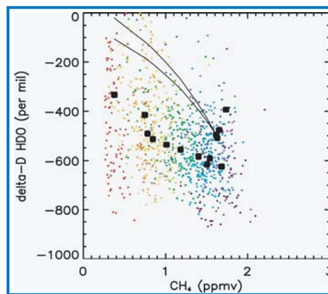
Figure 4.1 (16). Variation in HDO with methane shows the fraction of water coming from methane oxidation. The scatter is indicative of adiabatic mixing processes. Colors indicate altitude from blue near the tropopause to red in the mesosphere. Black curves are theoretical upper bounds on isotopic change in the absence of mixing.
