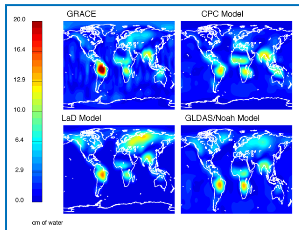
Figure 4.1 (24). GRACE monthly water storage variations compared against three predictive models.
