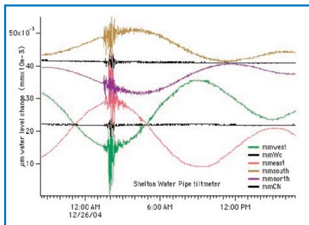
Figure 4.1 (2). The 26 Dec 2004 Sumatra earthquake recorded by a new CIRES 1-km-long tiltmeter. Height changes exceeded 50 \mu\text{m} at 20m minute periods.
