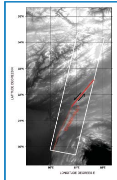
Figure 4.5 (7). A simulated SAR image of the area of study. The area covered by the interferograms is shown by the white box. The Chaman fault is indicated by the red line and the creeping segment by the thick red line. The black arrows indicate the direction of creep on the Chaman fault.
