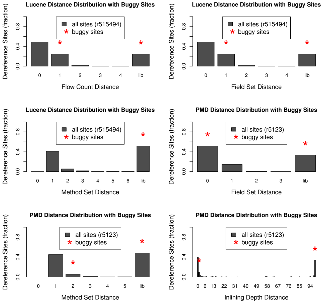
Figure 10: Distance distributions with buggy sites. Additional metrics.
