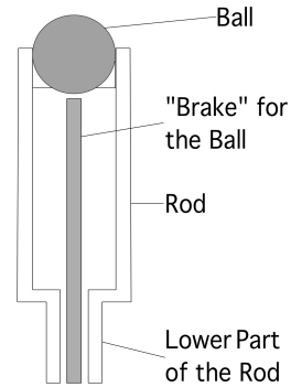
Figure 3. Each physical pixel consists of a rod whose height can be raised and lowered. The tip of each rod provides a mechanism for controlling the coefficient of friction, in this case a ball whose rotation can be adjusted or braked.
