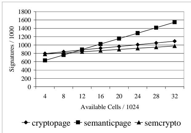
Figure 3a. Cells/Page=32
