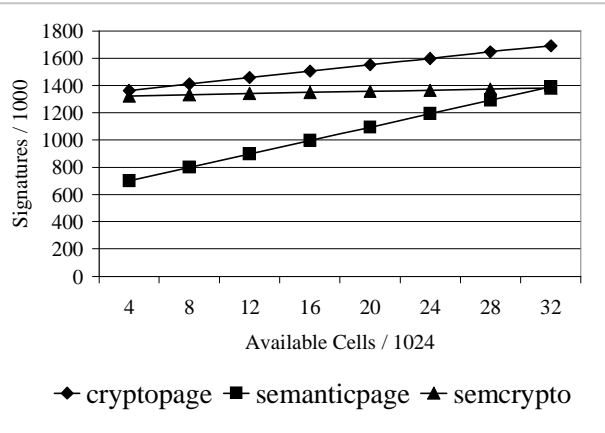
Figure 2b. Semispace
