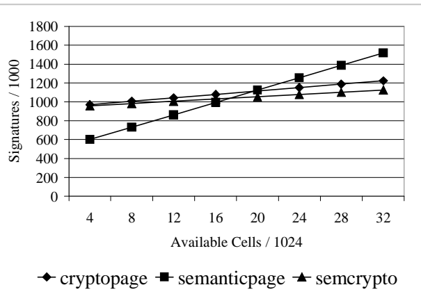
Figure 3b. Cells/Page=64
