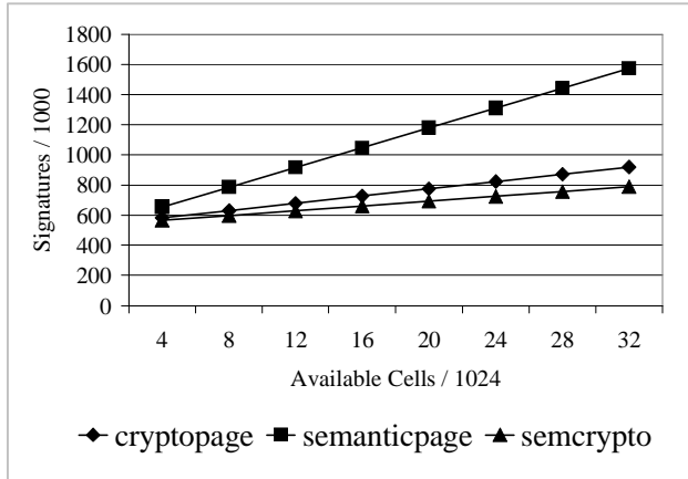
Figure 2a. MarkswEEP
