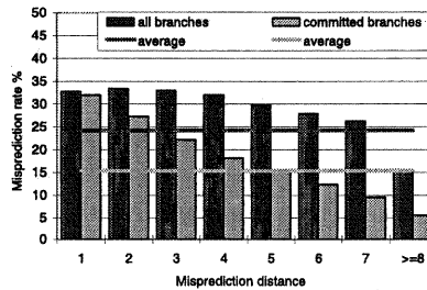
Figure 7: Misprediction distance using a McFarling branch predictor and precise misprediction information.
