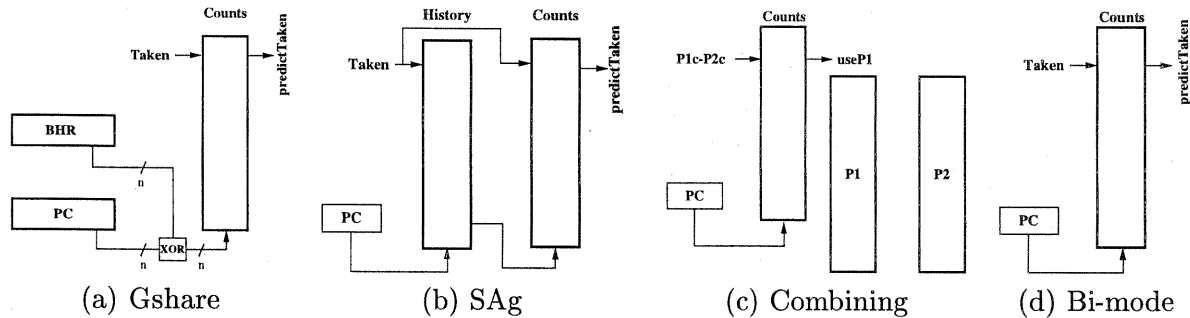
Figure 2: Schematic illustration of the different branch predictors used in this study
