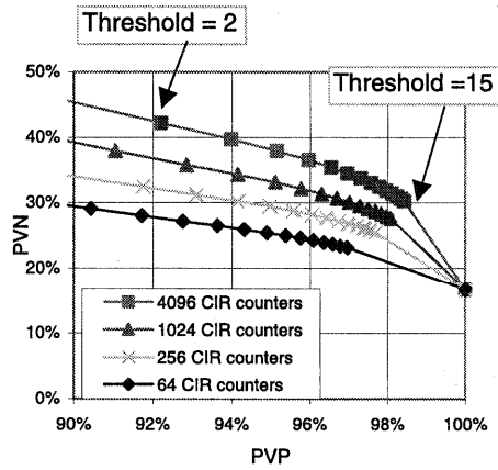
Figure 3: Performance of the JRS enhanced confidence estimator.
