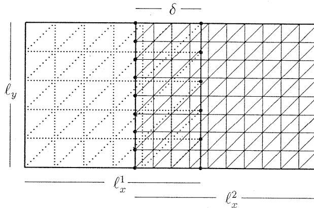
FIG. 1. The subregions \Omega_i, i = 1, 2 , are rectangles \Omega_i = \ell_x^i \times l_y . \ell_x^i, l_y are of O(1) . \delta is the size of the overlap.
