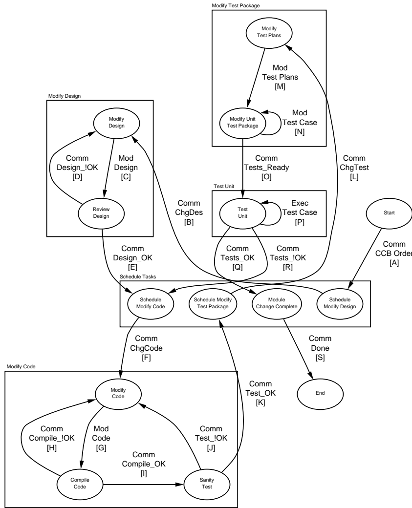
Figure 8: ISPW 6/7 Benchmark Process.
