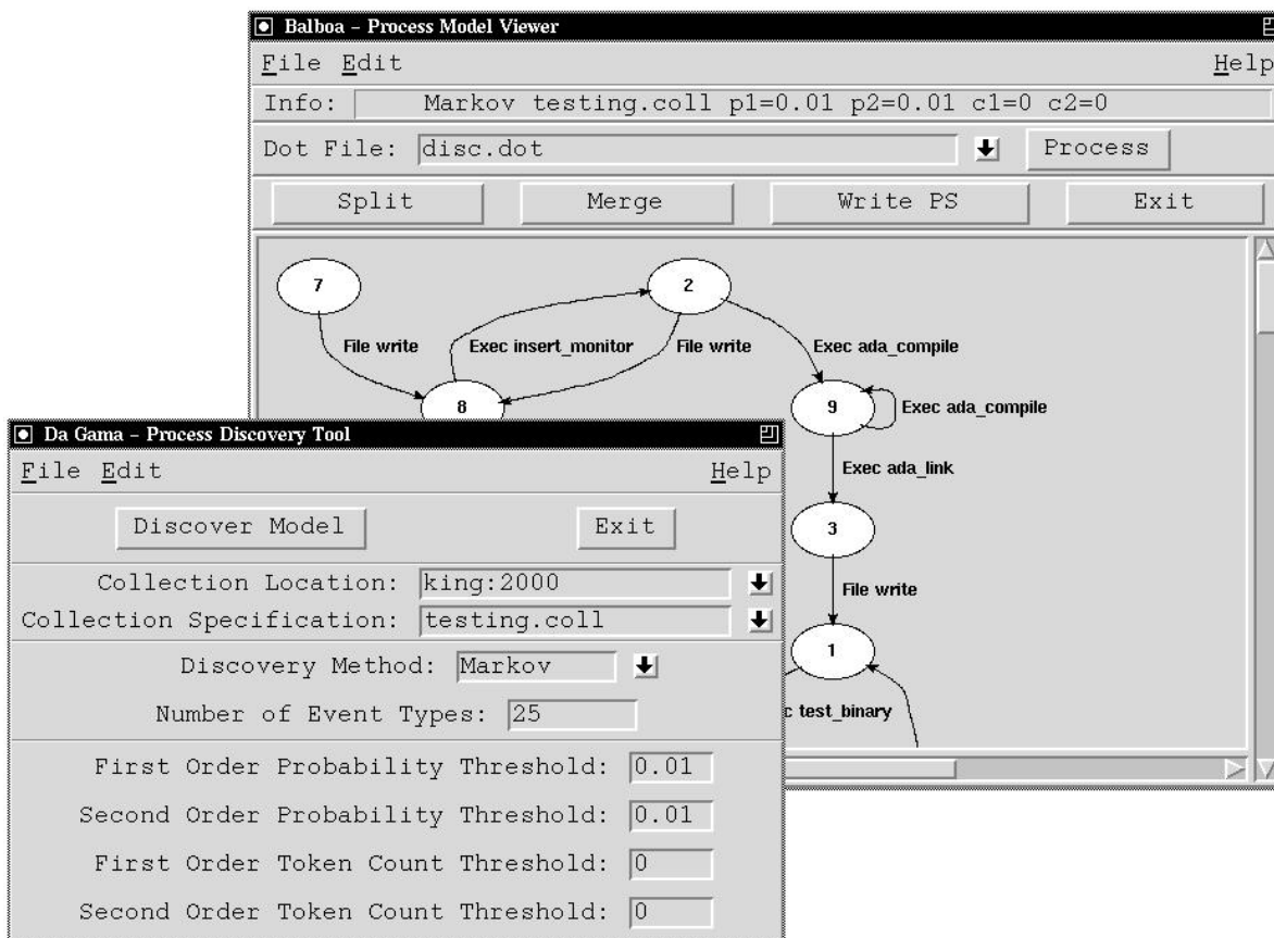
Figure 9: User Interface of DAGAMA.
