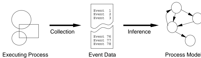
Figure 1: Process Model Discovery.
