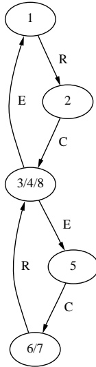
Figure 6: FSM Inferred by the KTAIL Method ( k = 2 ) for the Example Event Stream of Figure 2.
