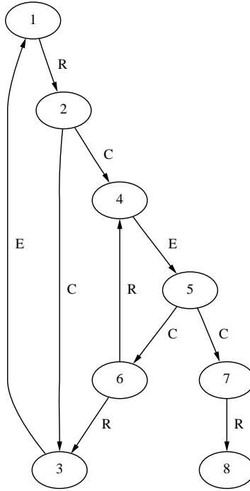
Figure 5: FSM Inferred by the Basic Biermann-Feldman Algorithm ( k = 2 ) for the Example Event Stream of Figure 2.
