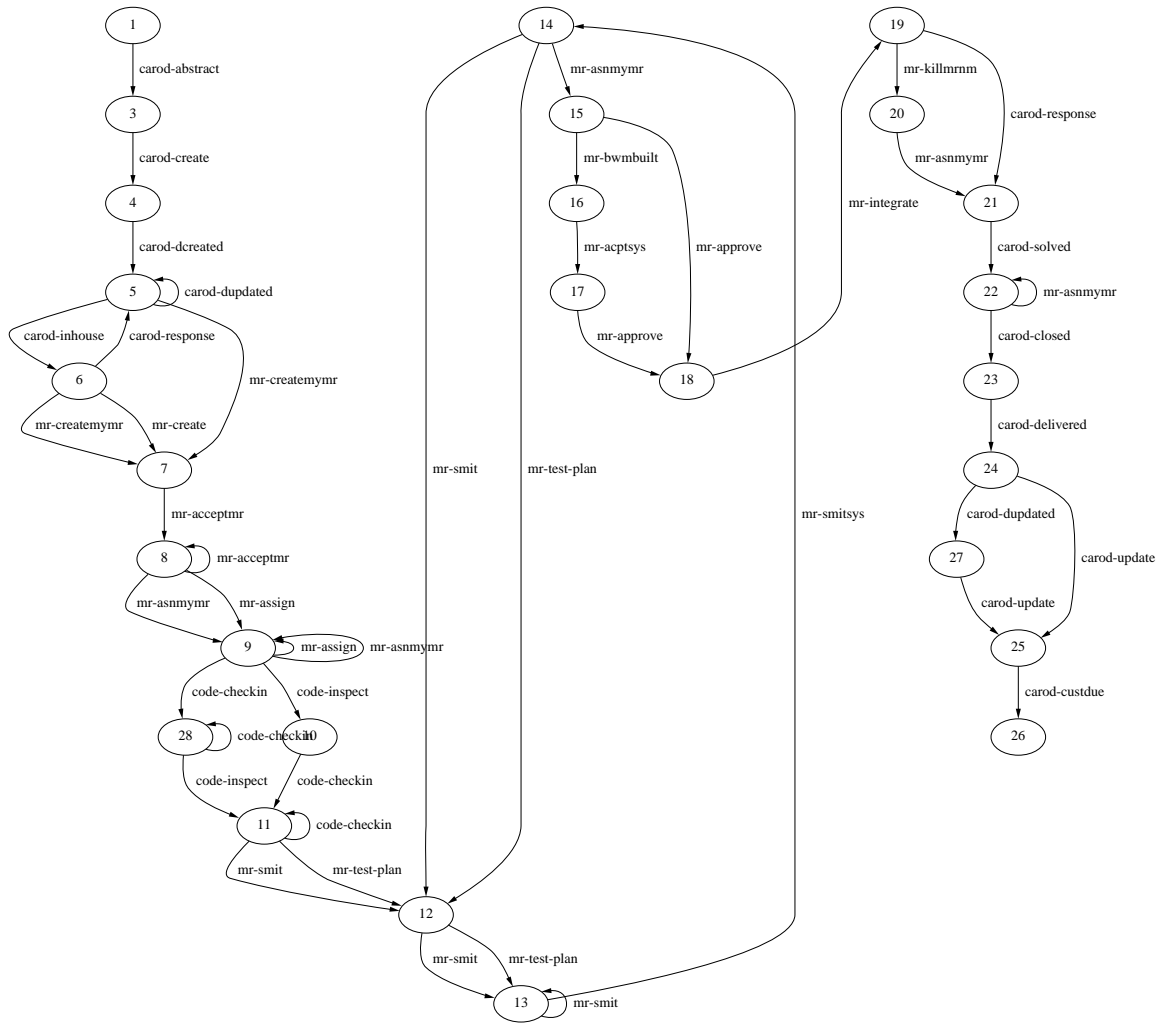
Figure 11: Final Process Model after Refinement.
