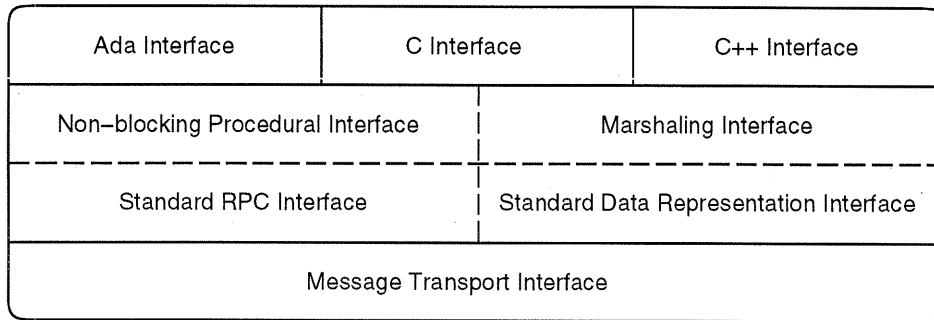
Figure 7: Q virtual machine layers
