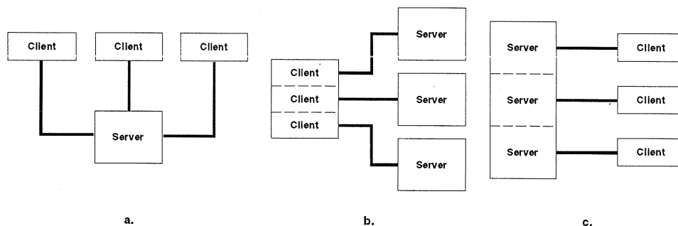
Figure 5: Logical client/server architectures
