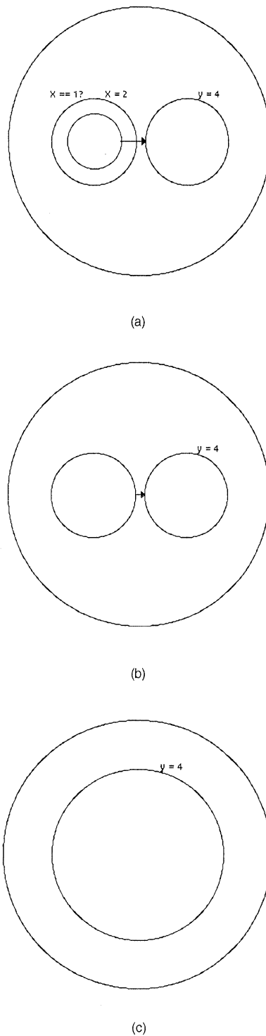
Figure 2. Execution of a VIPR program. (a) After application of selection rule. (b) After application of sequencing rule. (c) After application of substitution rule
