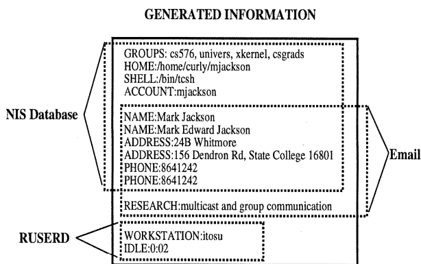
Figure 1: Example Mapping Algorithms for User Directory Information
