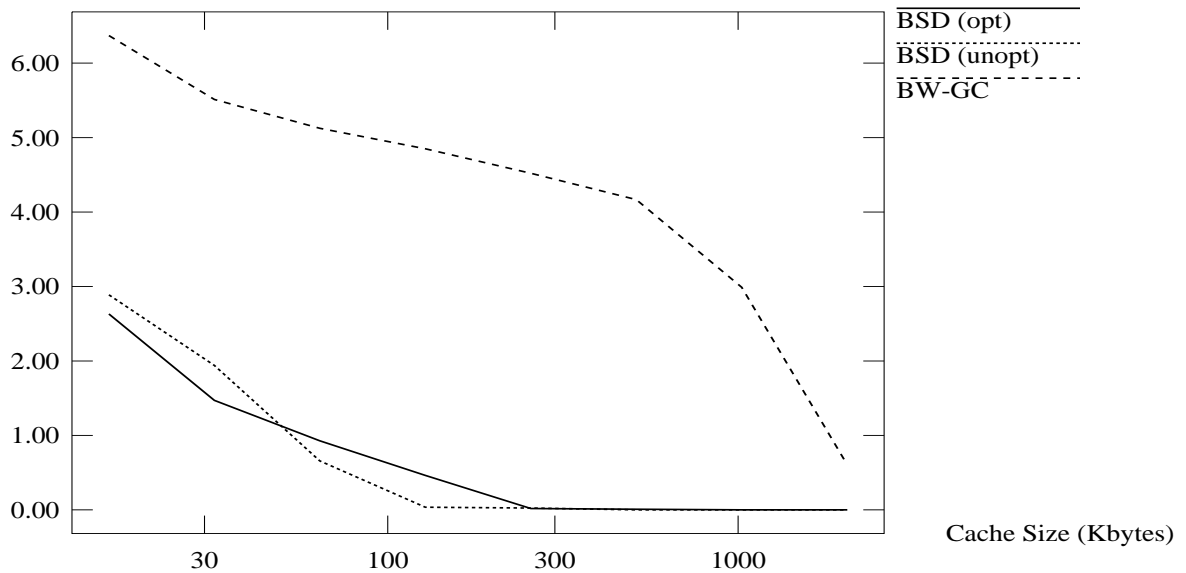
Figure 7: Cache miss rates for different direct-mapped cache sizes in the gawk application.
