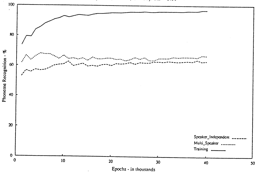
Figure 5.18: Comparative Performance for Two Learning Rates
