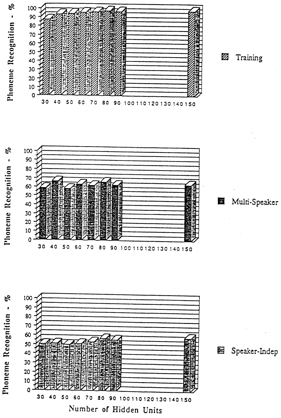
Figure 3.5: 1-frame Smoothed Data - Mimic Model
