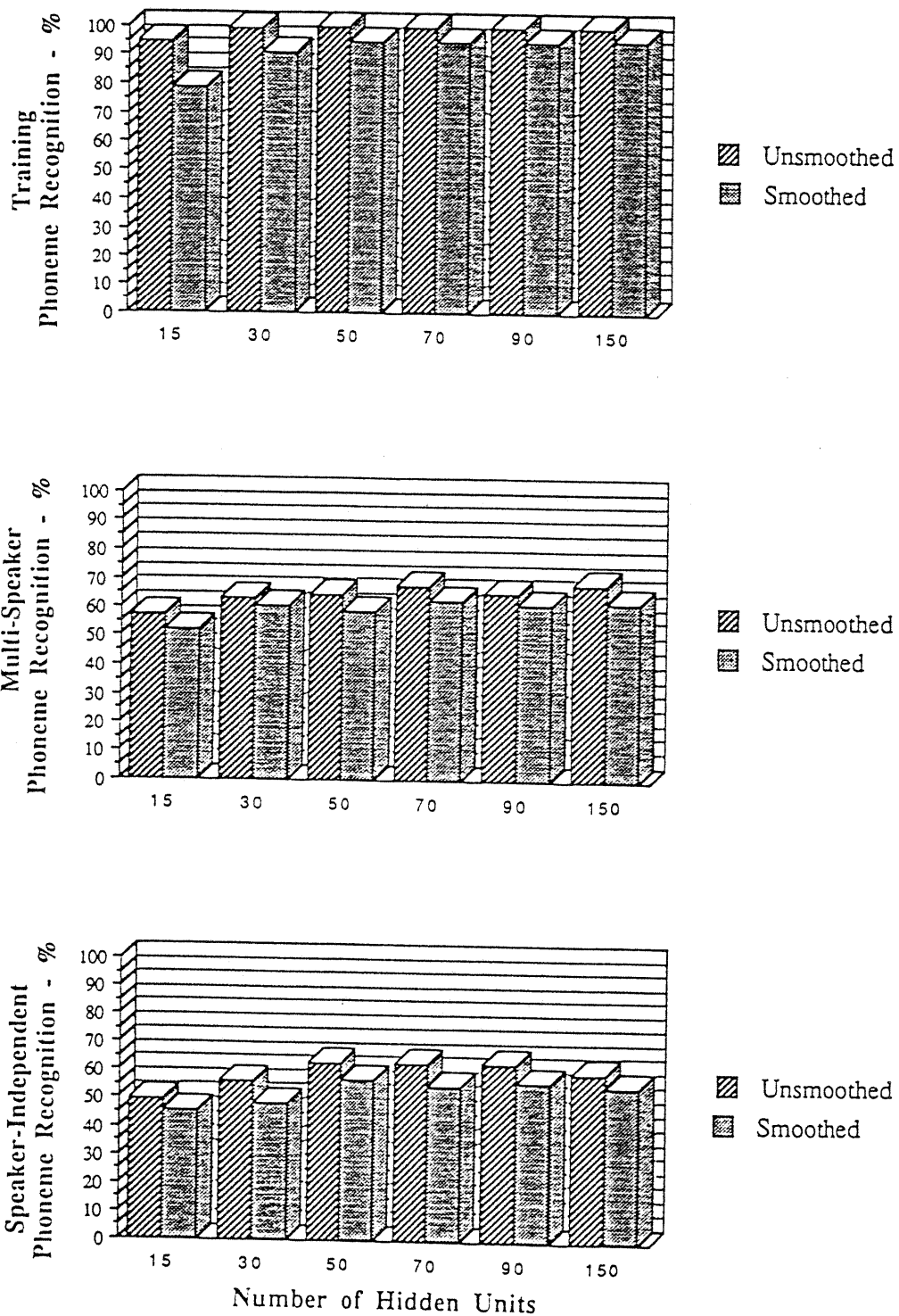
Figure 5.25: Smoothed vs. Unsmoothed Data - 1-frame Classifier
