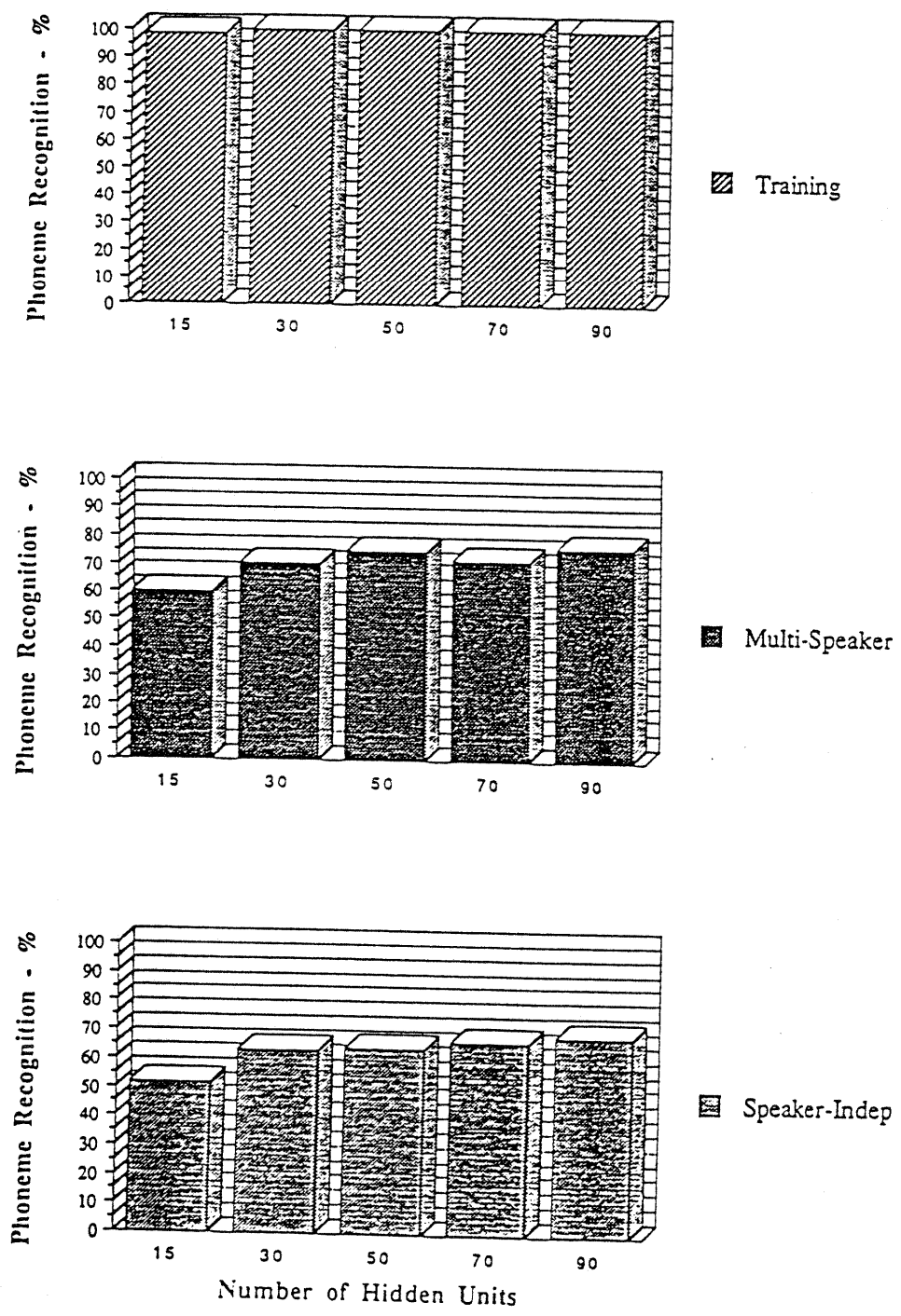
Figure 5.14: 3-frame Unsmoothed Data - Classifier Model
