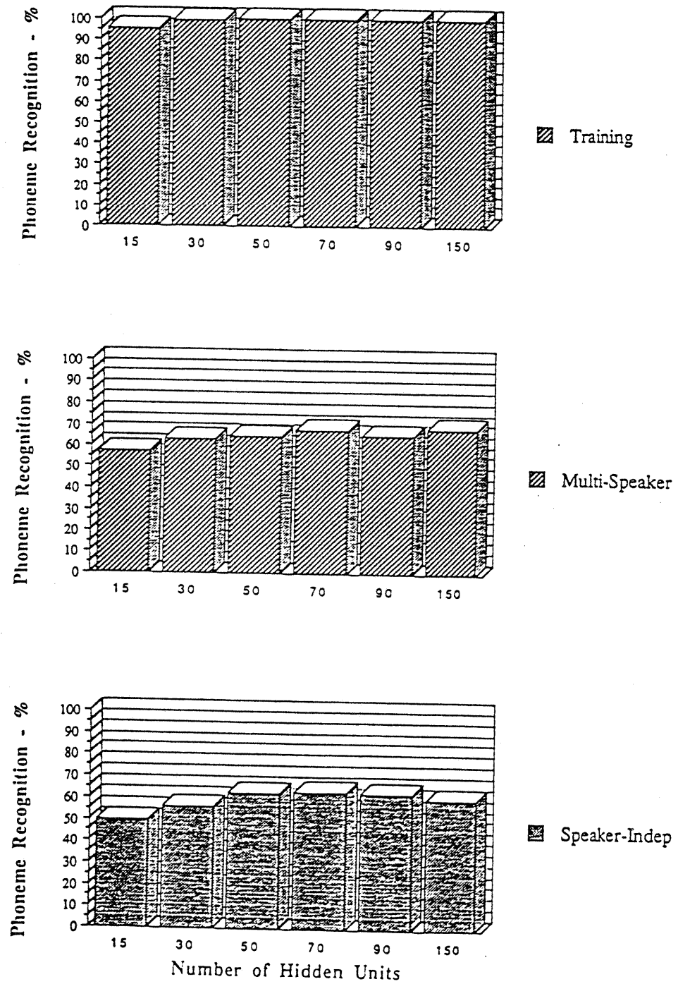
Figure 5.12: 1-frame Unsmoothed Data - Classifier Model
