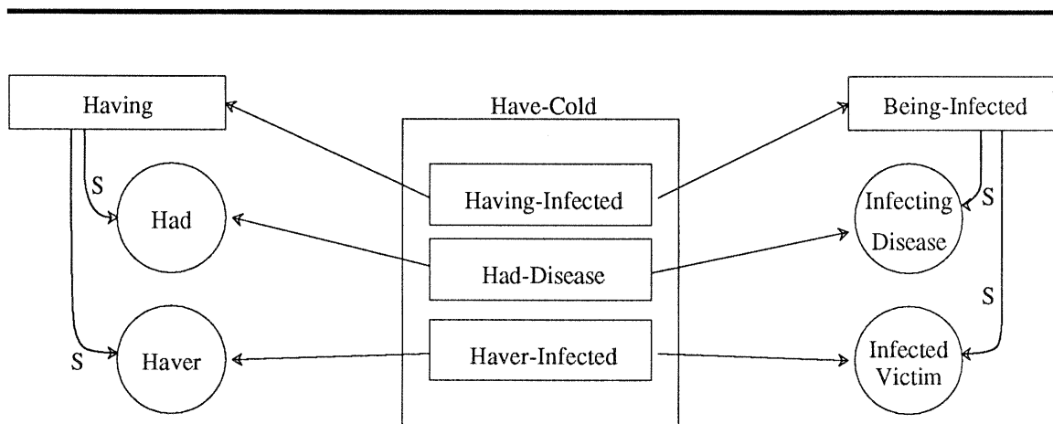
Figure 10: Have-Cold metaphor
