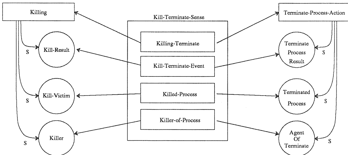
Figure 7: Kill-Terminate-Sense Abbreviated
