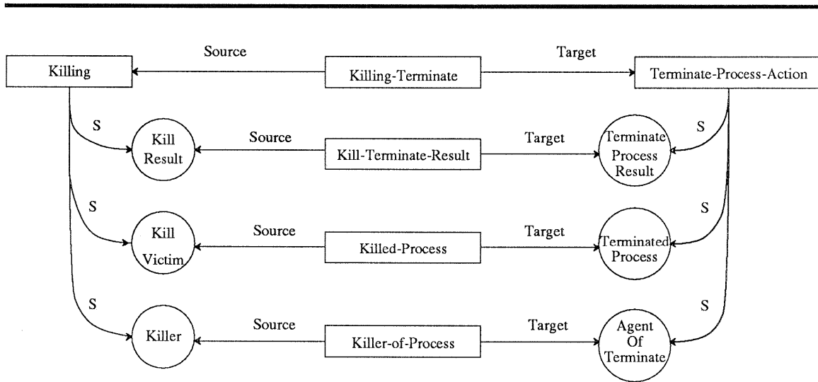
Figure 5: Kill-terminate-maps
