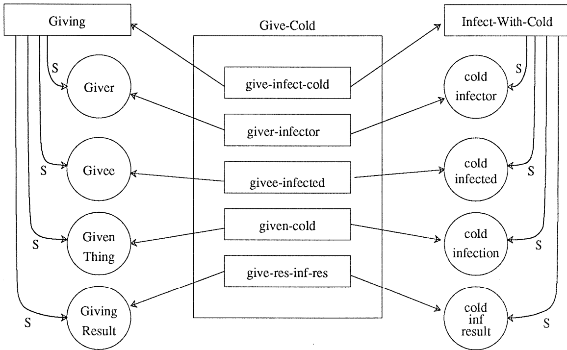
Figure 11: Give-Cold metaphor
