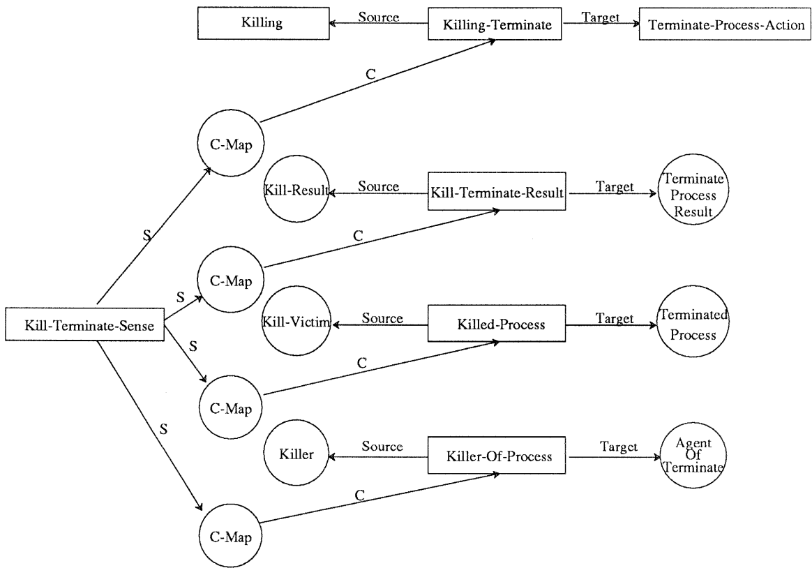
Figure 6: Kill-terminate-sense
