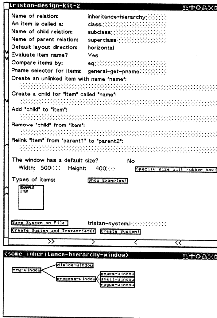
Figure 6-14: Initial state of the main form and an inheritance hierarchy window generated from it
