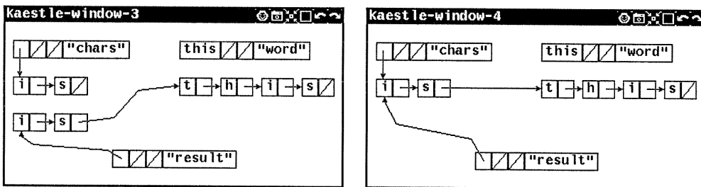
Figure 4-4: Illustration of the Validity of a Rule Using KAESTLE
