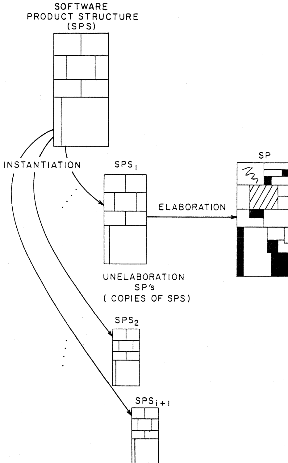
Figure 8: Software development, viewed as the process of instantiating an SPS and then elaborating the SPS instance into an SP.
