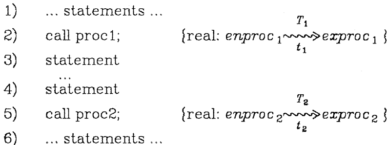
Figure 3 -- Code sequence containing interlevel calls
