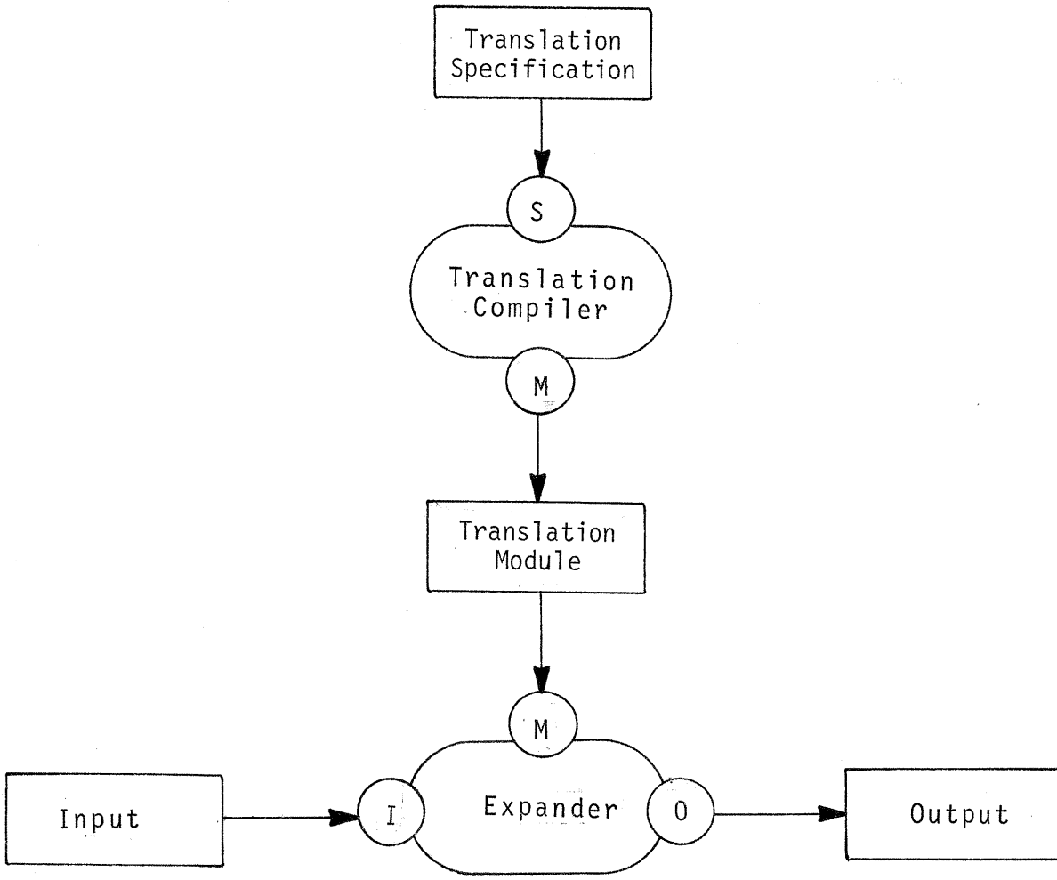
FIGURE 2: BIGMAC STRUCTURE
