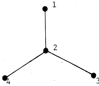
G(\bar{U}) for p = 2
