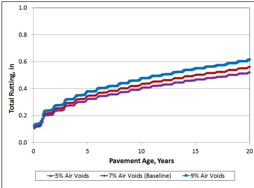
Figure 6.20 Sensitivity of Total Rutting to Air Voids
