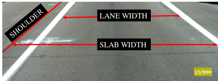
Figure 3.18 Schematic of Design Lane Width
