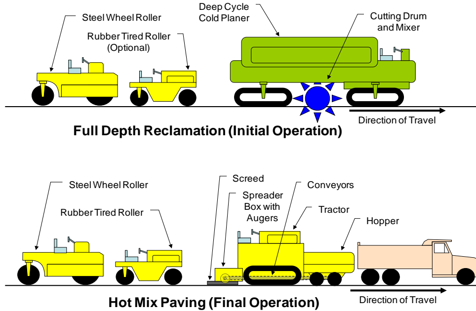
Figure 8.31 Schematic of FDR Equipment (sheeps foot not shown)
