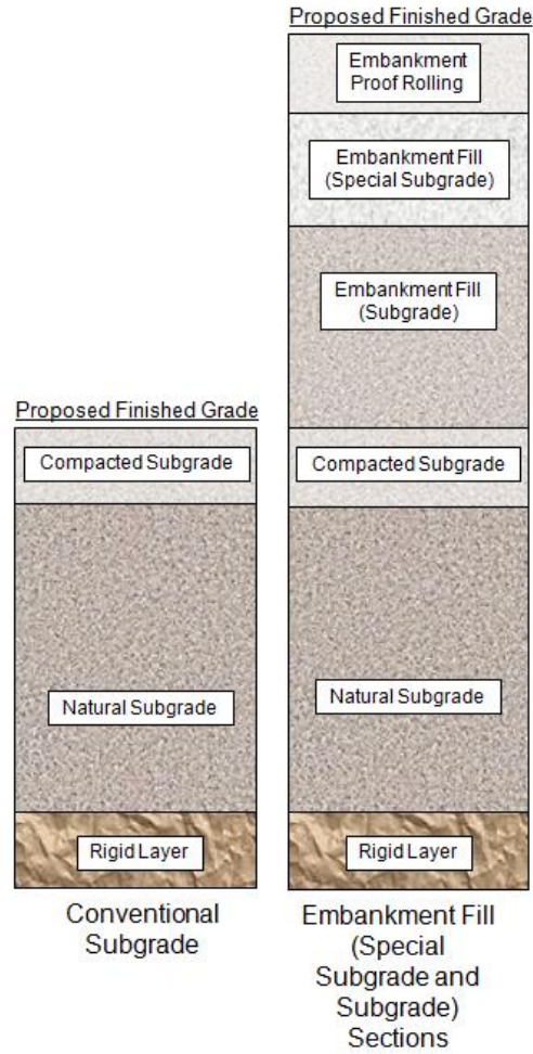
Figure 4.10 Special Cases of Embankment Fill
