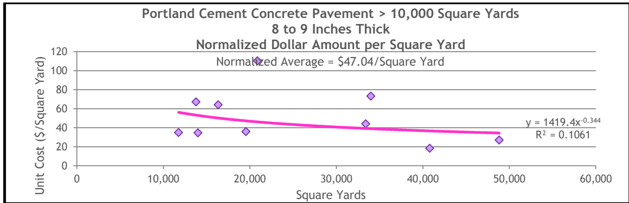
Figure 13.35 PCCP Normalized Dollar Amount for Projects of 8 to 9 Inches in Thickness and Greater Than 10,000 Square Yards in Size
