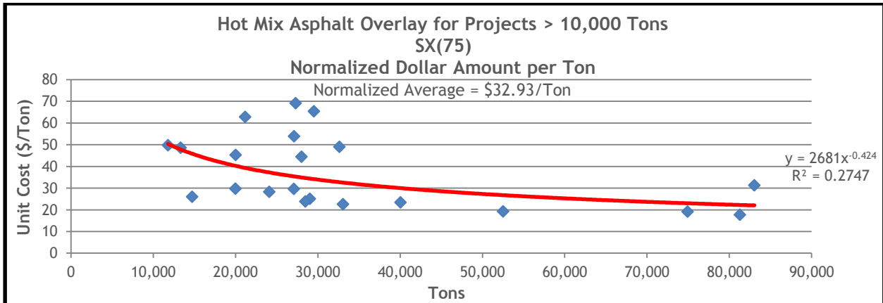
Figure 13.51 HMA Overlay Normalized Unit Costs for SX(75) on Projects Greater Than 10,000 Tons
