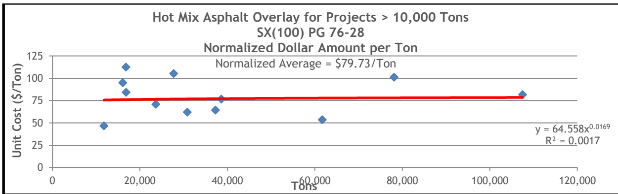
Figure 13.54 HMA Overlay Normalized Unit Costs for SX(100) PG 76-28 on Projects Greater Than 10,000 Tons
