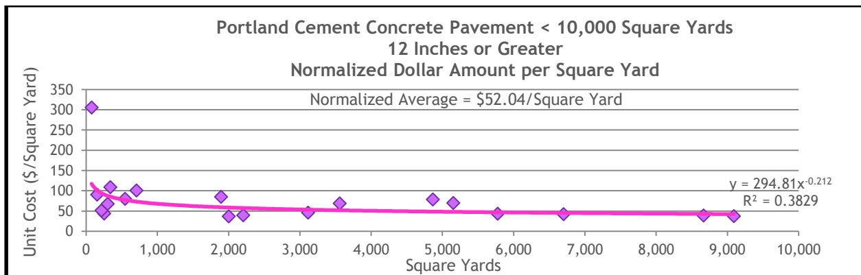
Figure 13.33 PCCP Normalized Dollar Amount for Projects of 12 Inches or Greater in Thickness and Less Than 10,000 Square Yards in Size
