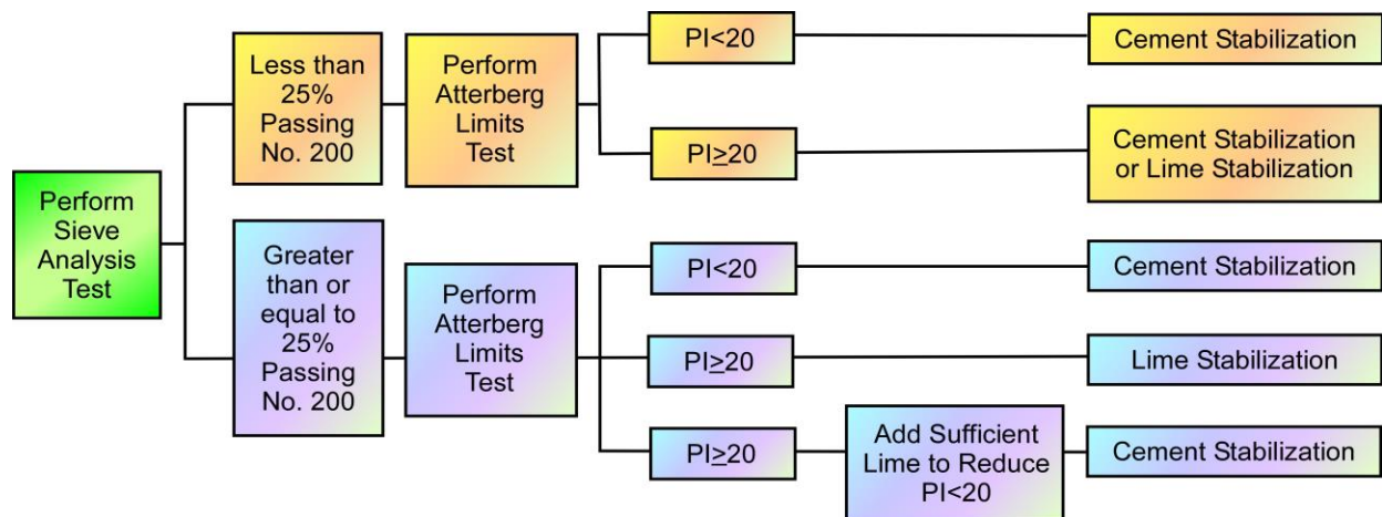
Figure 4.15 Lime/Cement-Stabilization Flow Chart
