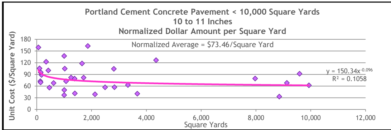
Figure 13.31 PCCP Normalized Dollar Amount for Projects of 10 to 11 Inches in Thickness and Less Than 10,000 Square Yards in Size
