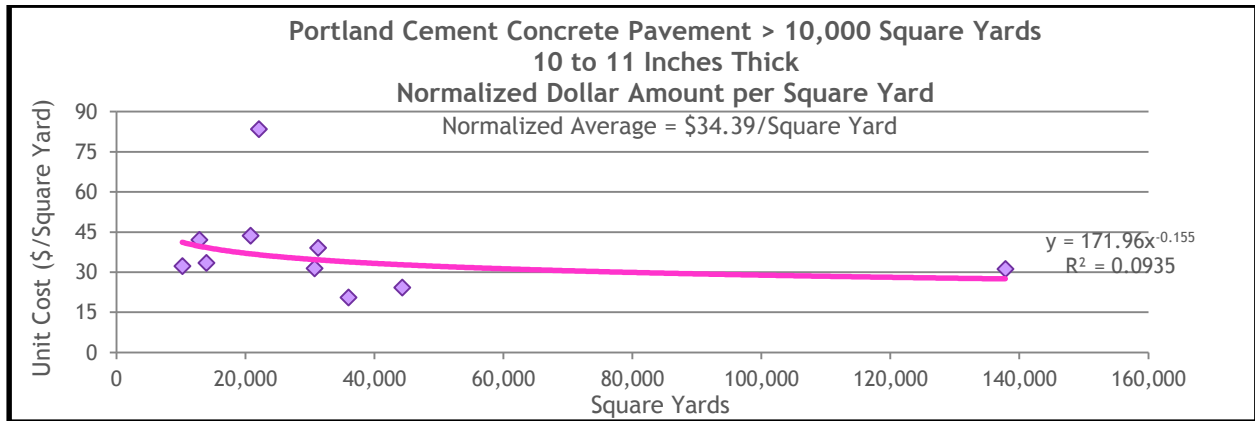
Figure 13.37 Normalized Dollar Amount for Projects of 10 to 11 Inches in Thickness and Greater Than 10,000 Square Yards in Size
