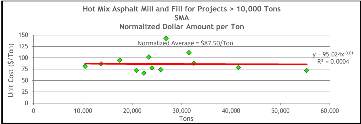
Figure 13.65 HMA Mill and Fill Normalized Unit Costs for SMA on Projects Greater Than 10,000 Tons
