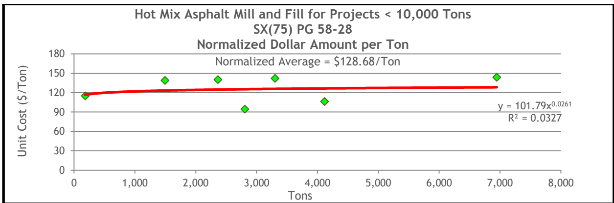
Figure 13.61 HMA Mill and Fill Normalized Unit Costs for SX(100) PG 58-28 on Projects Less Than 10,000 Tons
