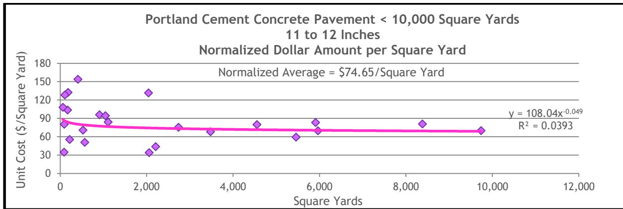
Figure 13.32 PCCP Normalized Dollar Amount for Projects of 11 to 12 Inches in Thickness and Less Than 10,000 Square Yards in Size
