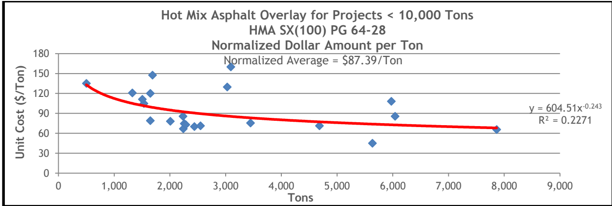
Figure 13.44 HMA Overlay Normalized Unit Costs for SX(100) PG 64-28 on Projects Less Than 10,000 Tons
