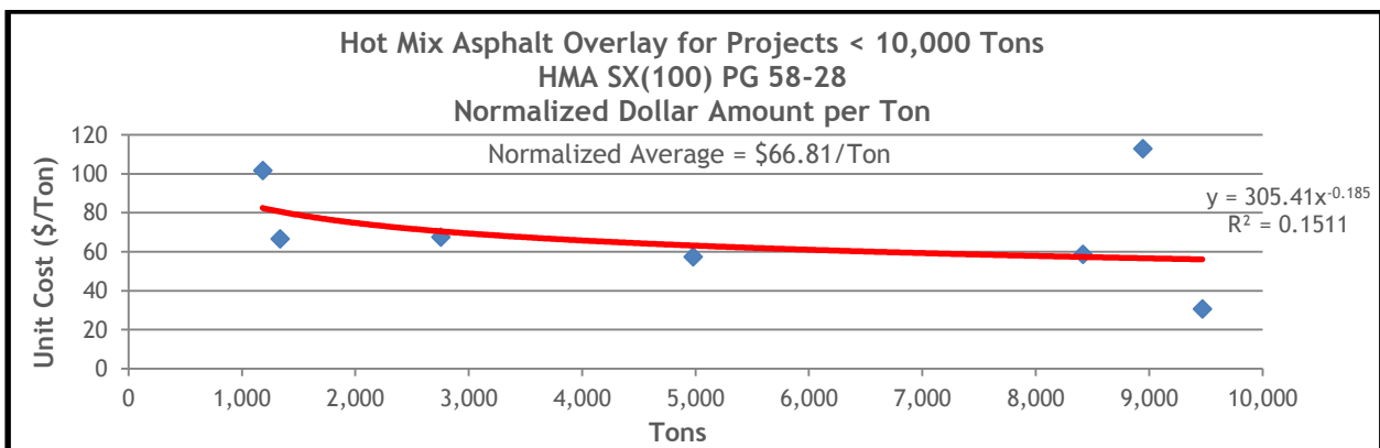
Figure 13.46 HMA Overlay Normalized Unit Costs for SX(100) PG 58-28 on Projects Less Than 10,000 Tons
