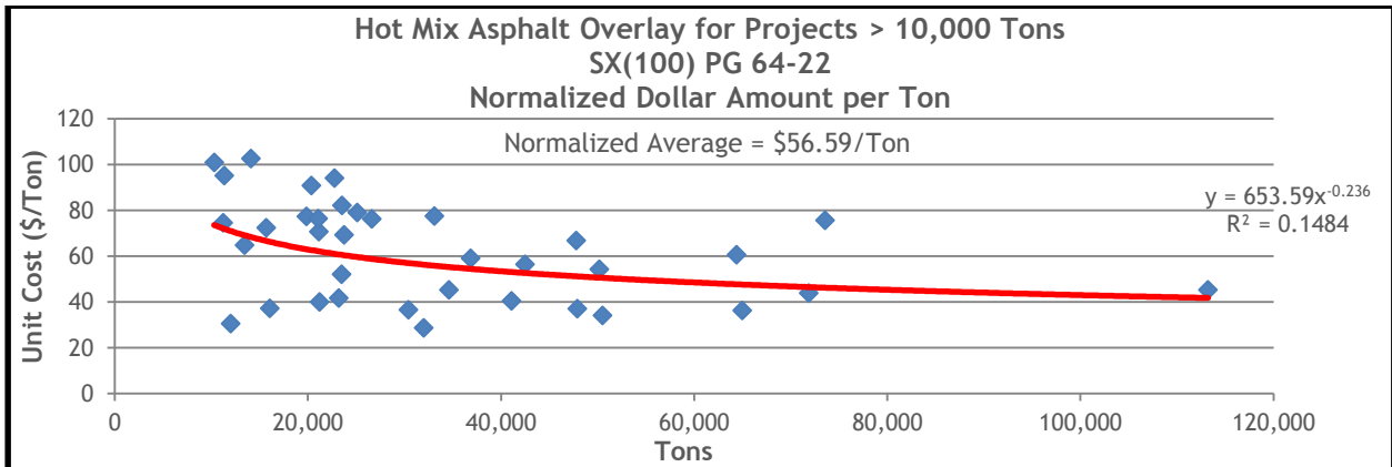
Figure 13.50 HMA Overlay Normalized Unit Costs for SX(100) PG 64-22 on Projects Greater Than 10,000 Tons
