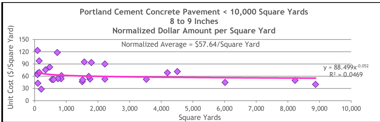
Figure 13.29 Normalized Dollar Amount for Projects of 8 to 9 Inches in Thickness and Less Than 10,000 Square Yards in Size
