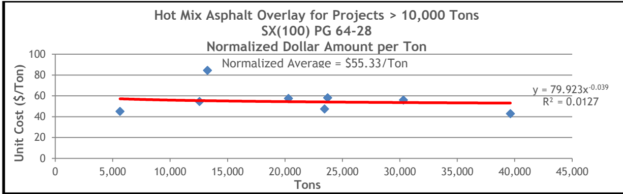
Figure 13.53 HMA Overlay Normalized Unit Costs for SX(100) PG 64-28 on Projects Greater Than 10,000 Tons
