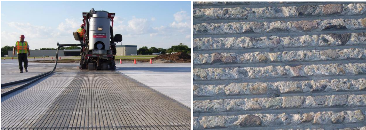
Figure 10.2 Photos of Diamond Grinding and Grooving
