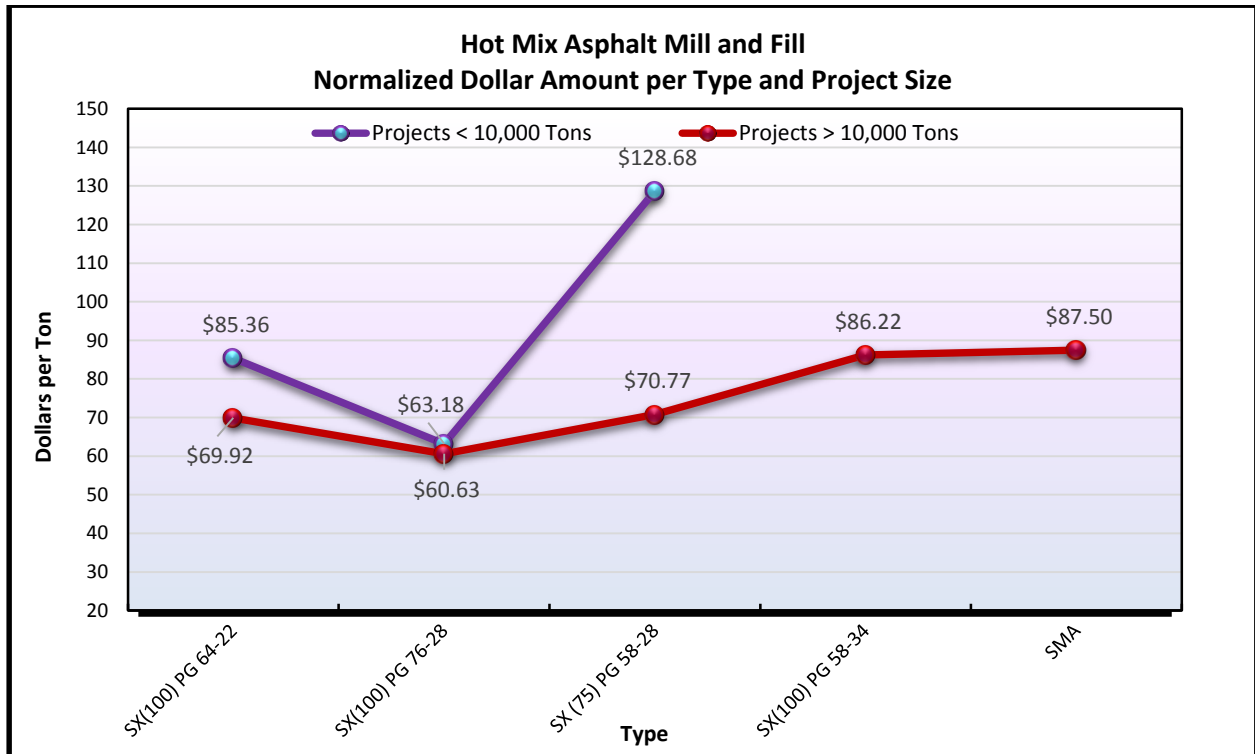
Figure 13.56 HMA Mill and Fill Normalized Dollar per Product Type
