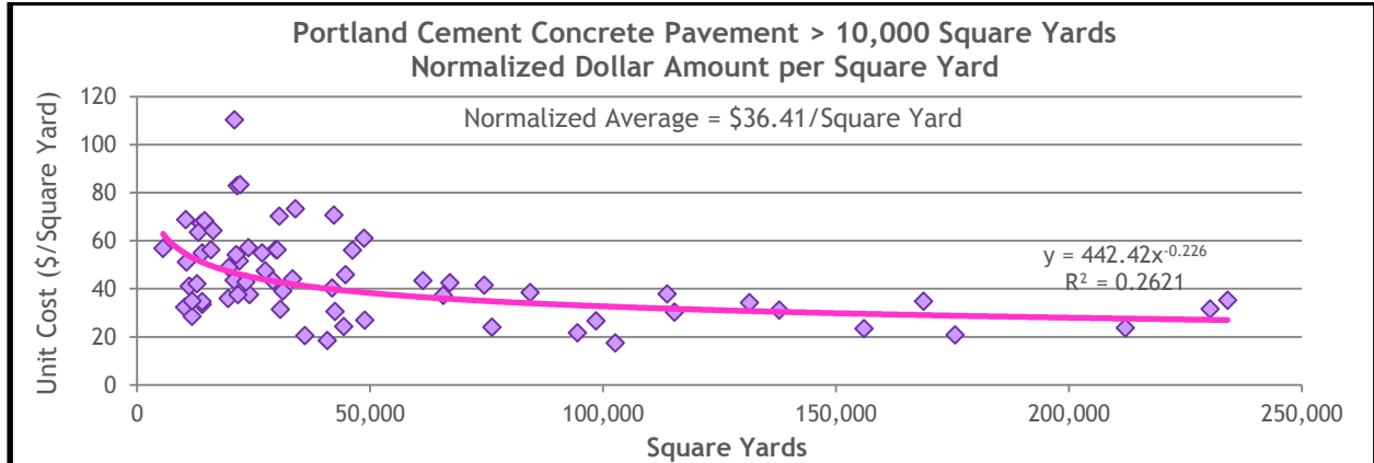
Figure 13.34 PCCP Normalized Dollar Amount per Total Square Yards for Projects Greater Than 10,000 Square Yards
