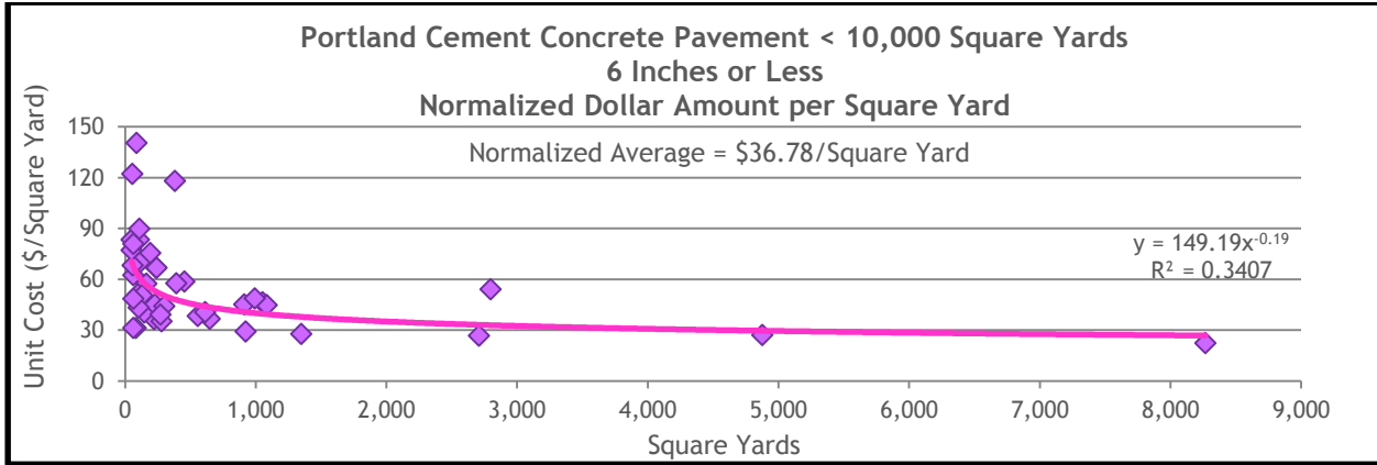
Figure 13.28 PCCP Normalized Dollar Amount for Projects of 6 Inches or Less in Thickness and Less Than 10,000 Square Yards in Size
