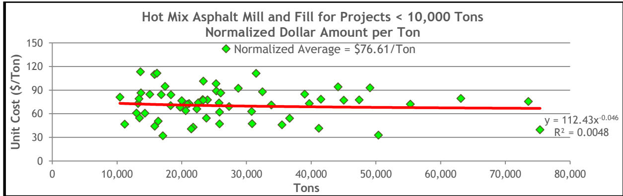
Figure 13.58 HMA Mill and Fill Normalized Unit Costs for Projects Less Than 10,000 Tons
