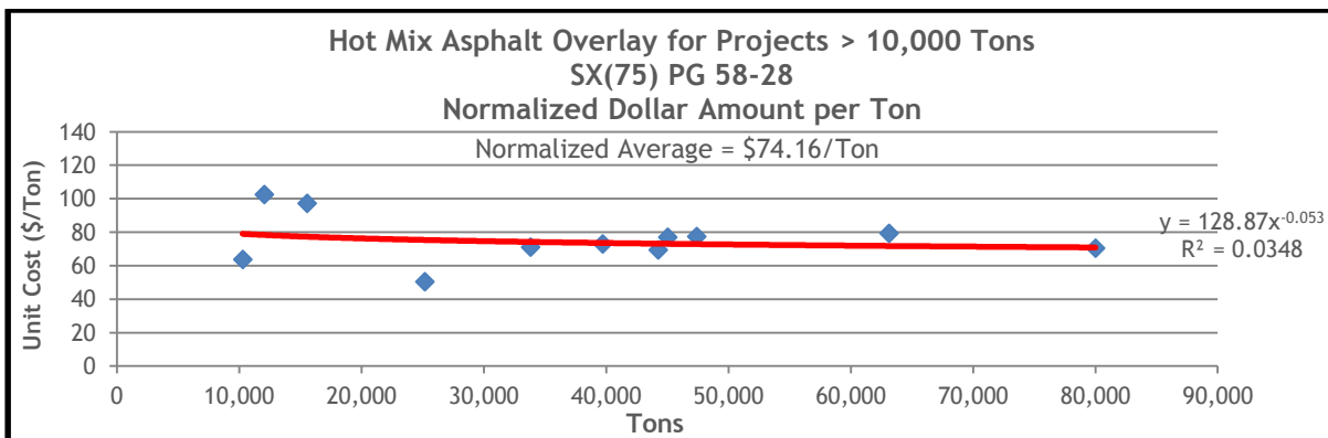
Figure 13.52 HMA Overlay Normalized Unit Costs for SX(100) PG 58-28 on Projects Greater Than 10,000 Tons
