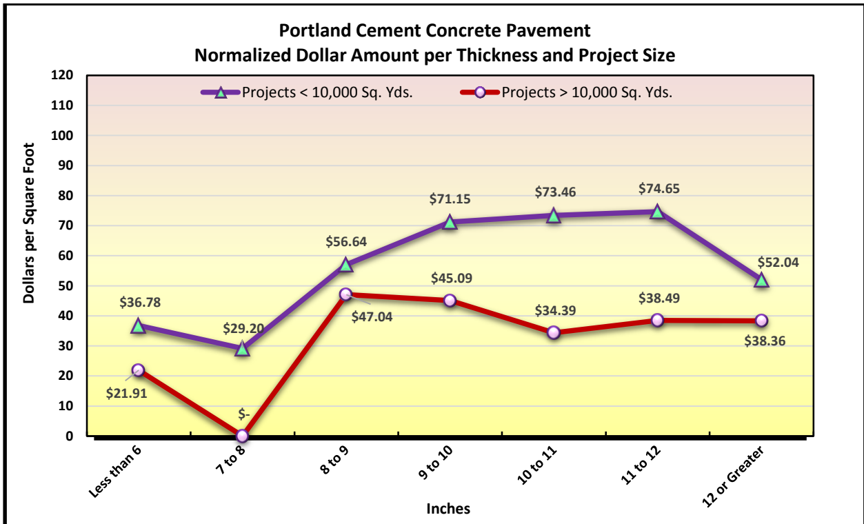
Figure 13.25 PCCP Normalized Dollar Amount per Thickness
