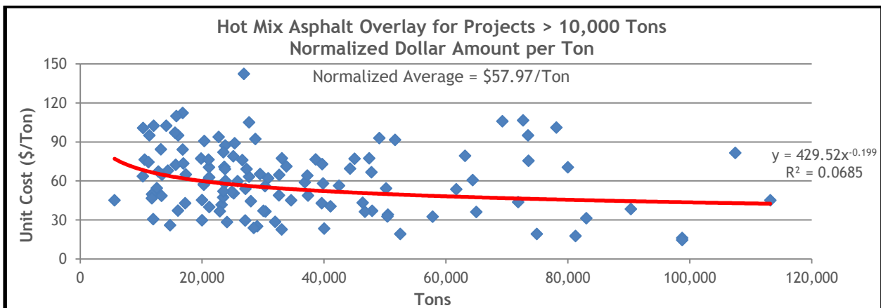
Figure 13.49 HMA Overlay Normalized Unit Costs for Projects with Greater Than 10,000 Tons
