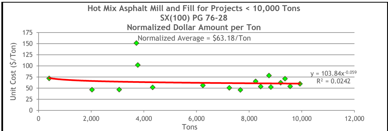
Figure 13.60 HMA Mill and Fill Normalized Unit Costs for SX(100) PG 76-28 on Projects Less Than 10,000 Tons
