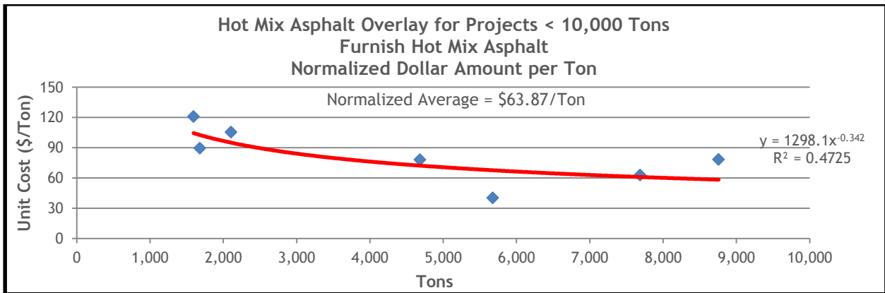
Figure 13.48 HMA Overlay Normalized Unit Costs for Furnish HMA on Projects Less Than 10,000 Tons
