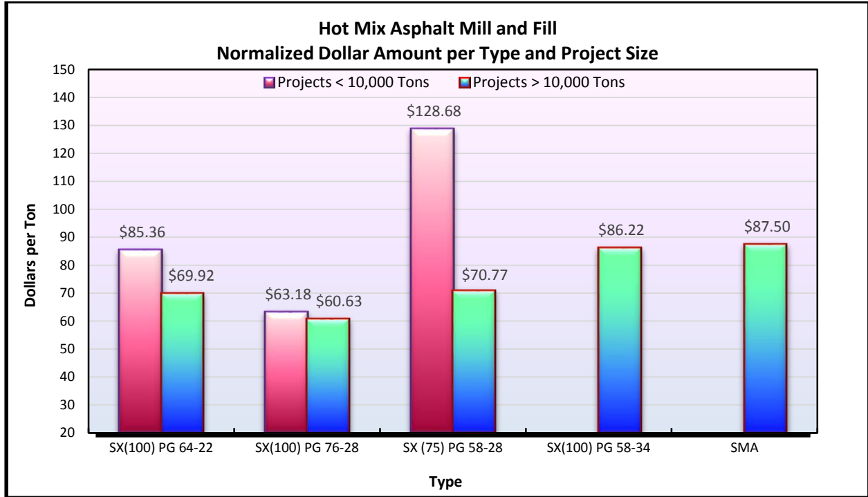
Figure 13.57 HMA Mill and Fill Normalized Dollar per Product Type
