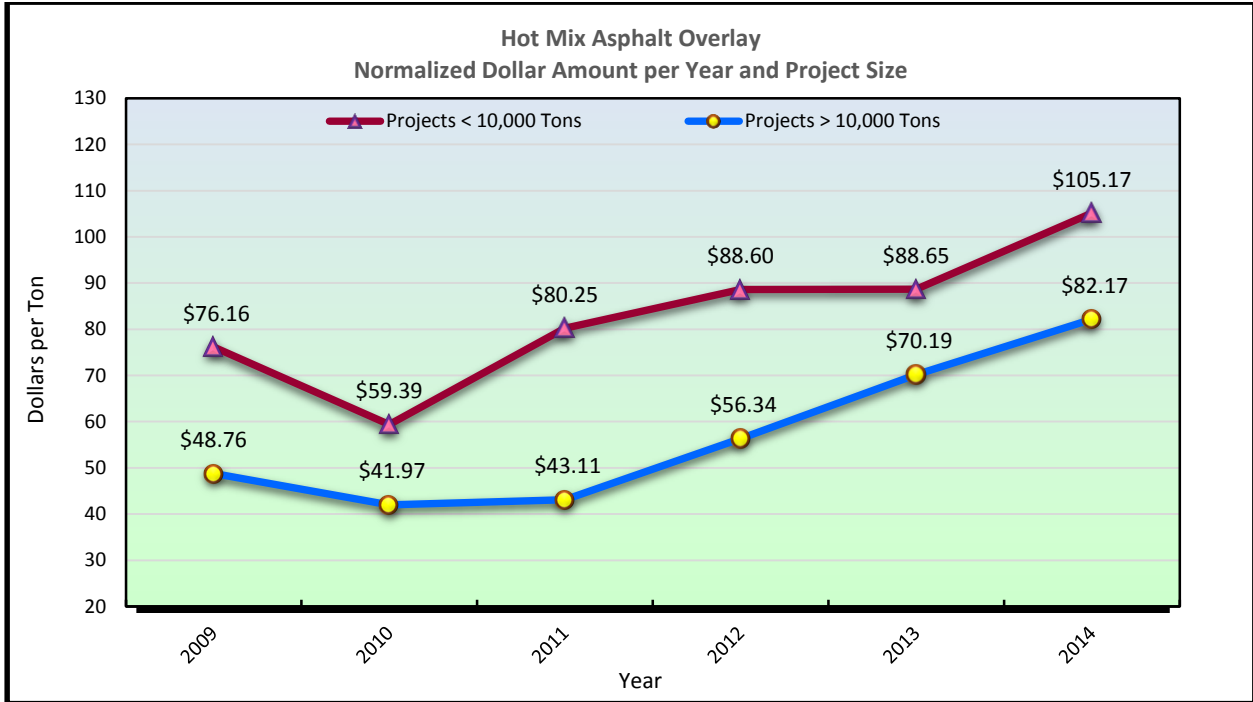
Figure 13.40 HMA Overlay Normalized Dollar per Year and Project Size
