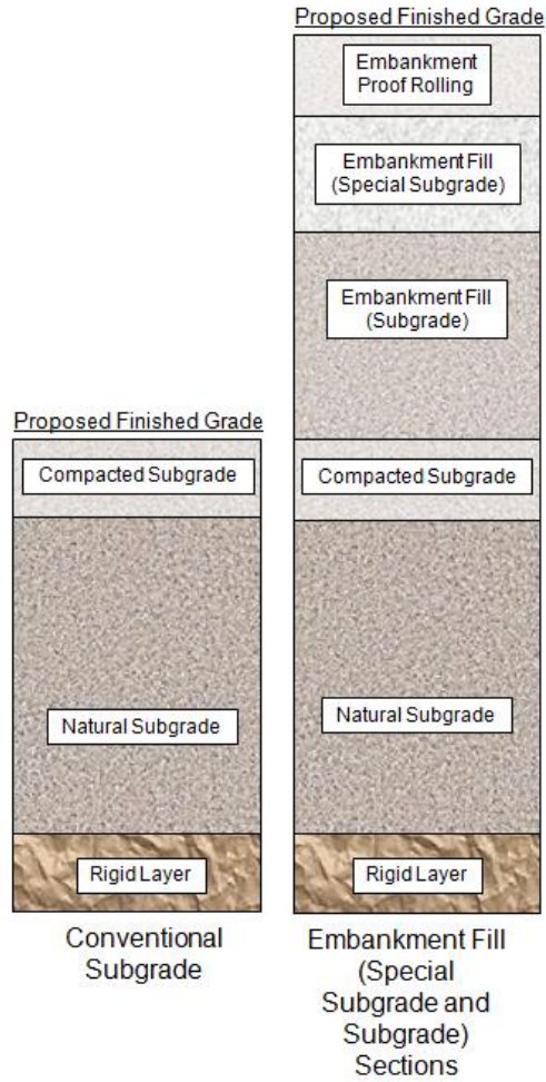
Figure 4.2 Special Cases of Embankment Fill
