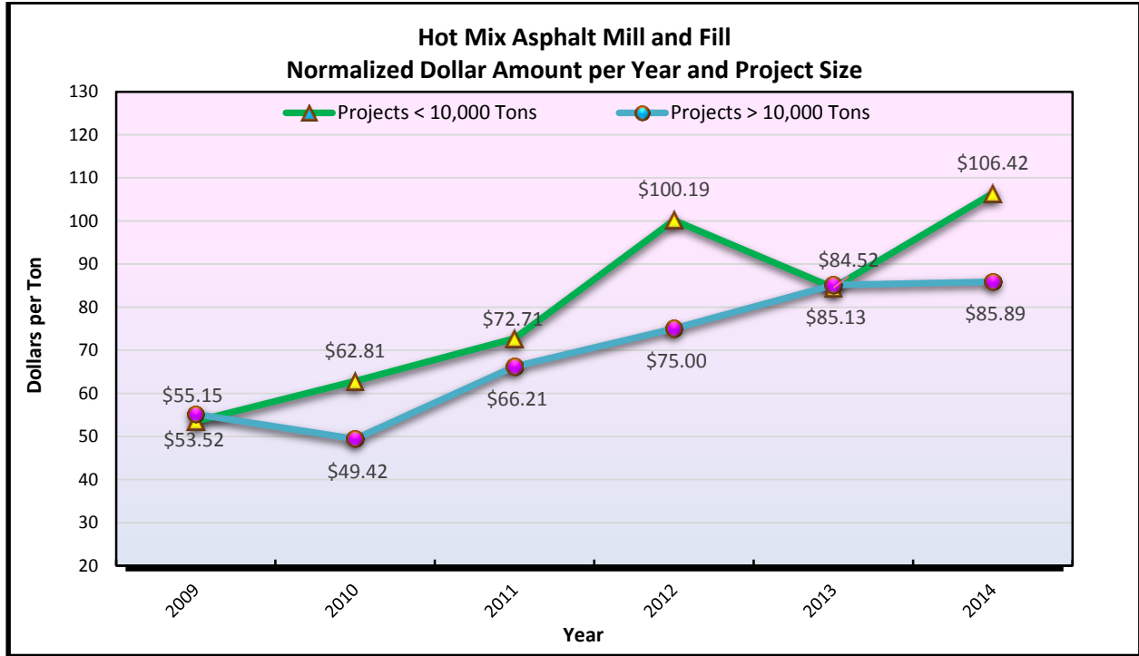
Figure 13.55 HMA Mill and Fill Normalized Dollar per Year and Project Size
