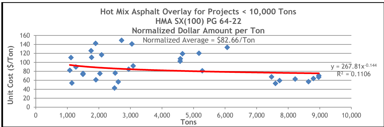
Figure 13.45 HMA Overlay Normalized Unit Costs for SX(100) PG 64-22 on Projects Less Than 10,000 Tons
