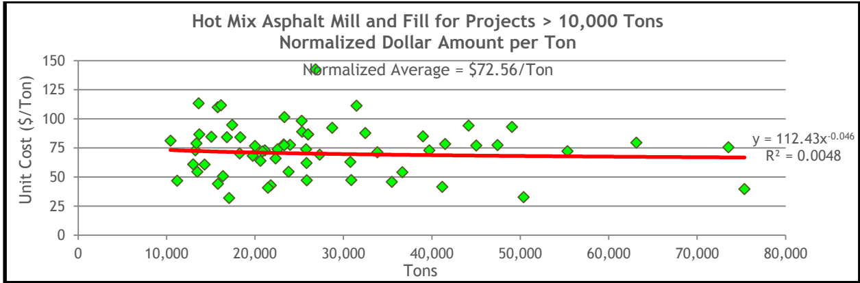
Figure 13.62 HMA Mill and Fill Normalized Unit Costs for Projects Greater Than 10,000 Tons
