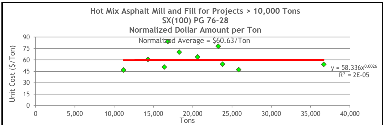
Figure 13.63 HMA Mill and Fill Normalized Unit Costs for SX(100) PG 76-28 on Projects Greater Than 10,000 Tons
