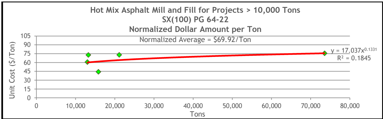
Figure 13.66 HMA Mill and Fill Normalized Unit Costs for SX(100) PG 64-22 on Projects Greater Than 10,000 Tons
