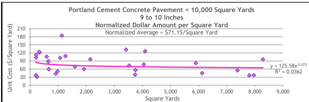
Figure 13.30 Normalized Dollar Amount for Projects of 9 to 10 Inches in Thickness and Less Than 10,000 Square Yards in Size
