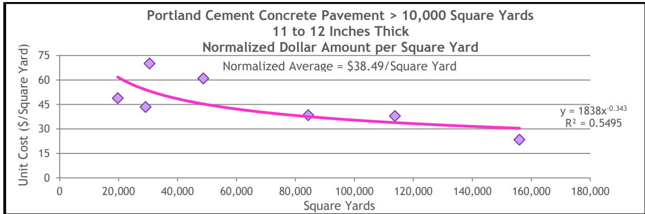
Figure 13.38 PCCP Normalized Dollar Amount for Projects of 11 to 12 Inches in Thickness and Greater Than 10,000 Square Yards in Size
