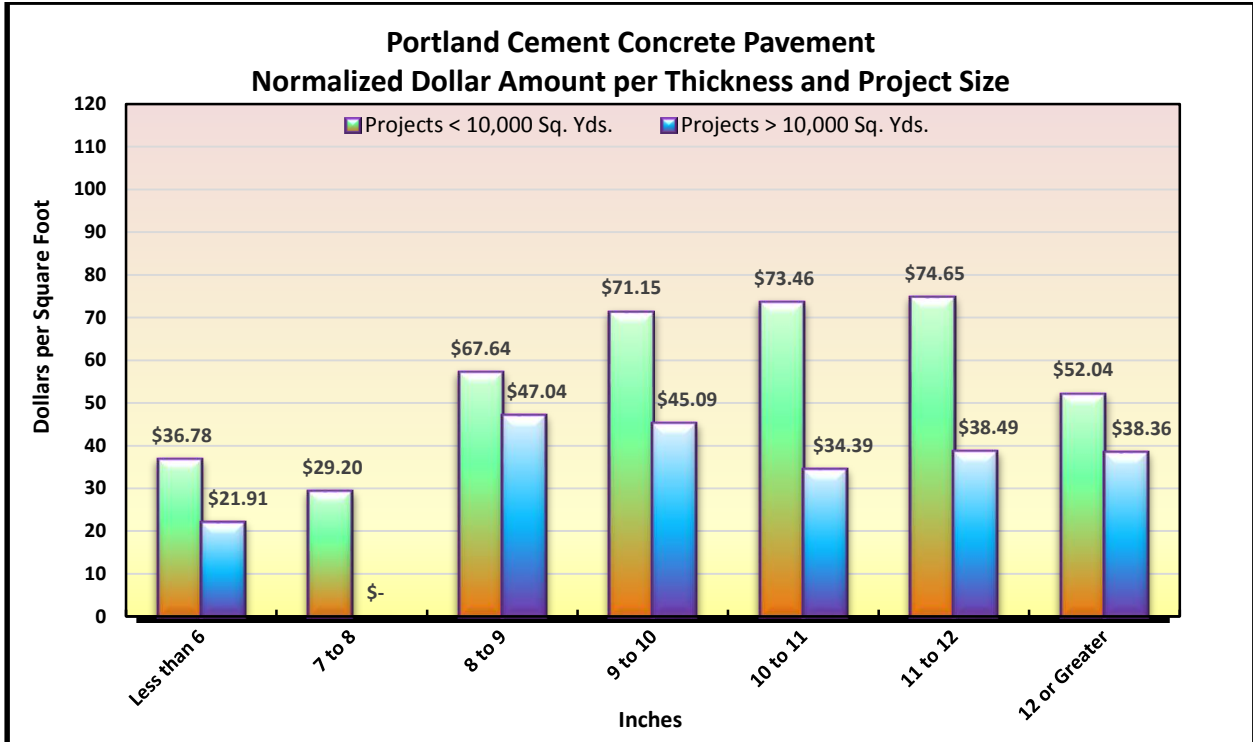
Figure 13.26 PCCP Normalized Dollar Amount per Thickness
