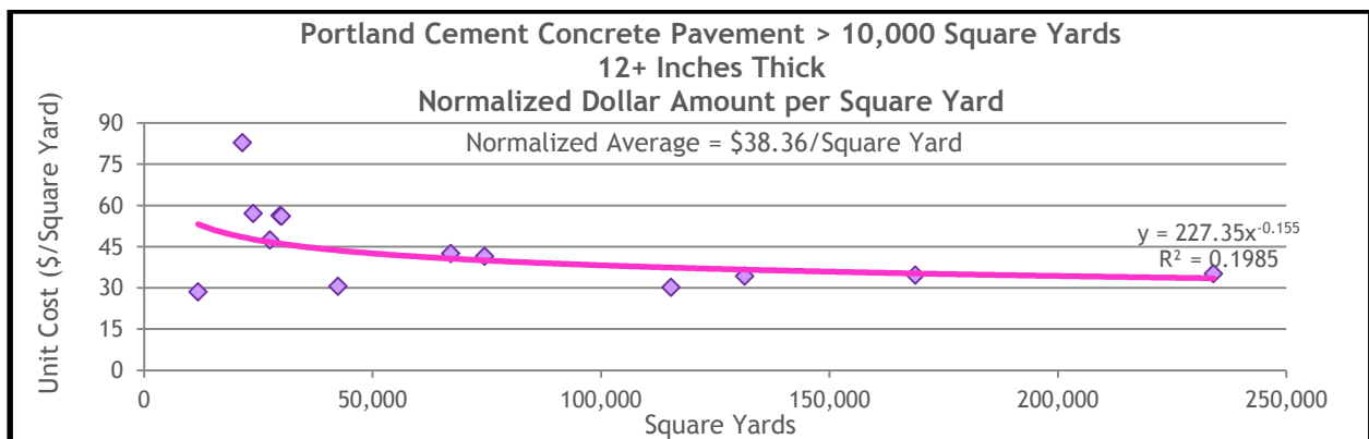
Figure 13.39 PCCP Normalized Dollar Amount for Projects of 12 Inches or Greater in Thickness and Greater Than 10,000 Square Yards in Size
