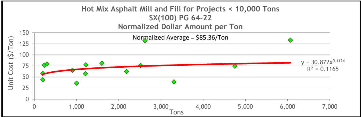
Figure 13.59 HMA Mill and Fill Normalized Unit Costs for SX(100) PG 64-22 on Projects Less Than 10,000 Tons
