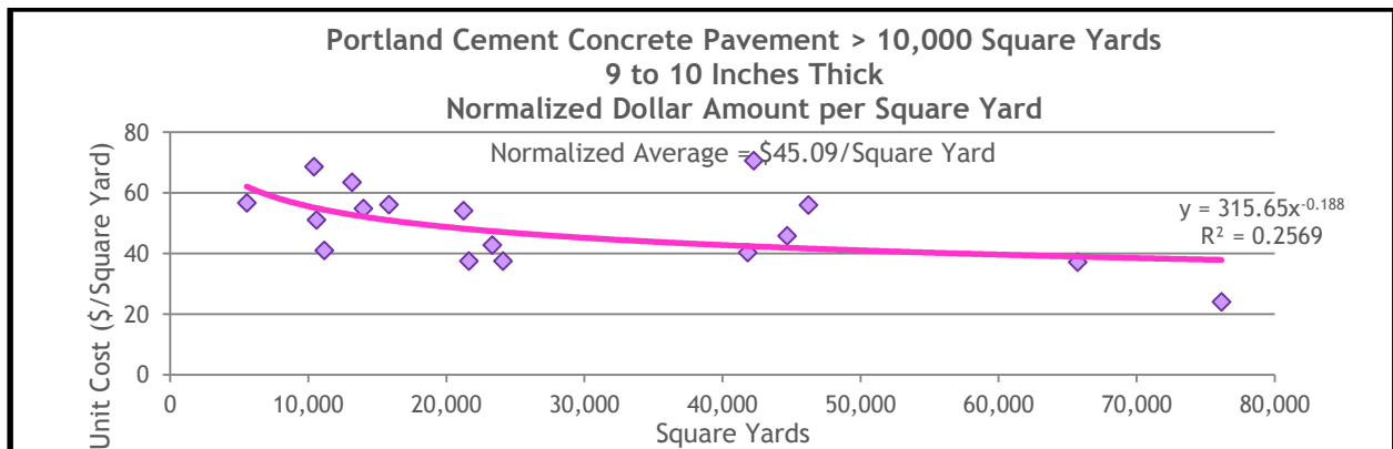
Figure 13.36 PCCP Normalized Dollar Amount for Projects of 9 to 10 Inches in Thickness and Greater Than 10,000 Square Yards in Size
