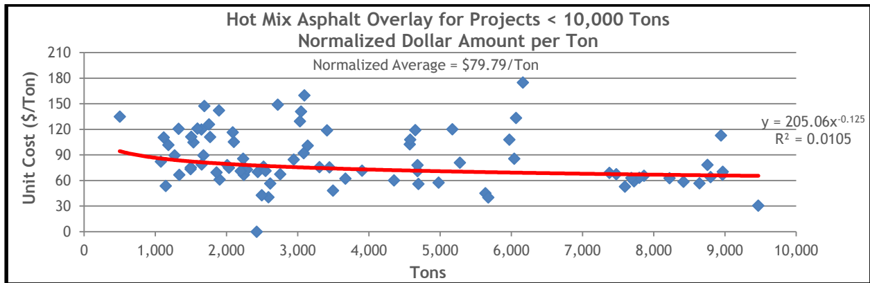
Figure 13.43 HMA Overlay Normalized Dollar Amount for Projects Less Than 10,000 Tons
