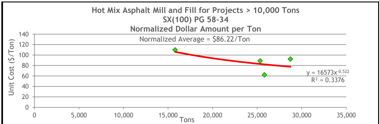
Figure 13.67 HMA Mill and Fill Normalized Unit Costs for SX(100) PG 58-34 on Projects Greater Than 10,000 Tons
