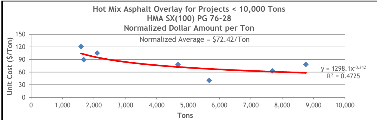
Figure 13.47 HMA Overlay Normalized Unit Costs for SX(100) PG 76-28 on Projects Less Than 10,000 Tons
