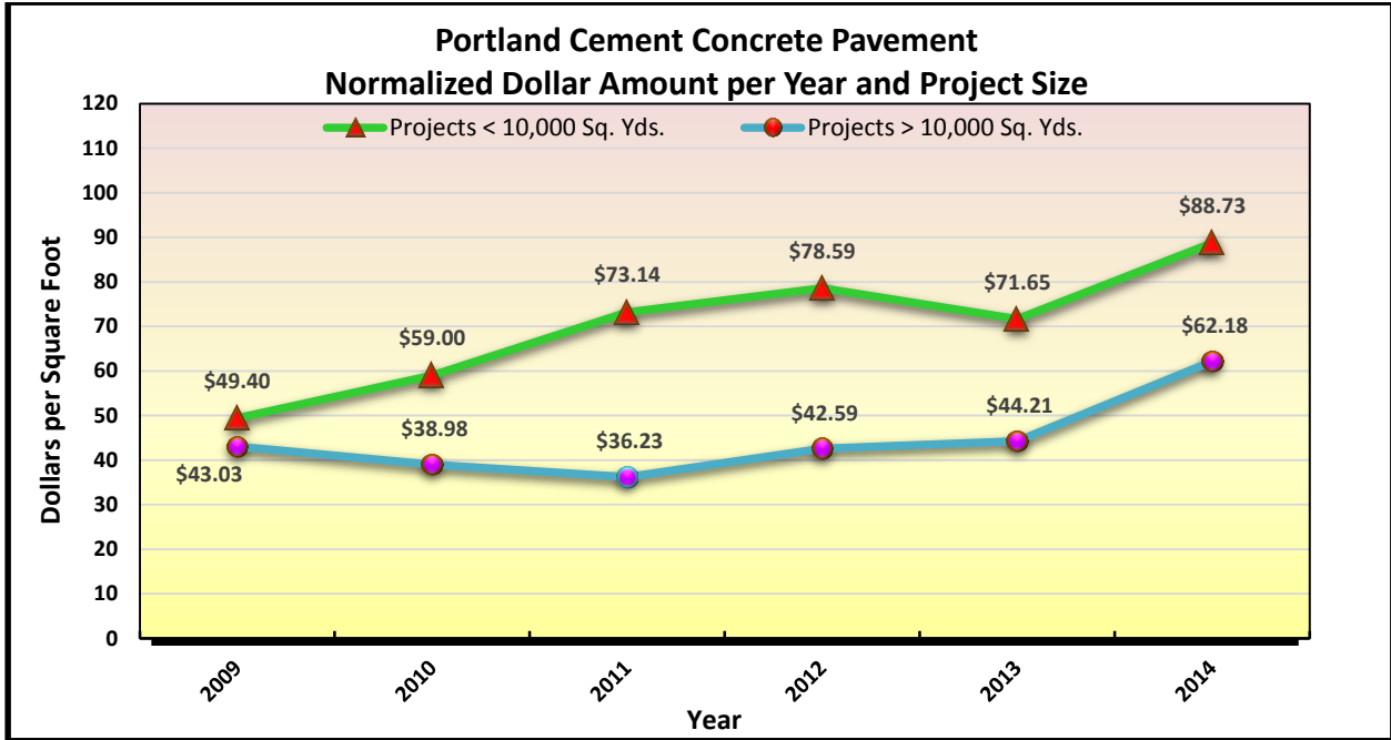
Figure 13.24 PCCP Normalized Dollar Amount per Year
