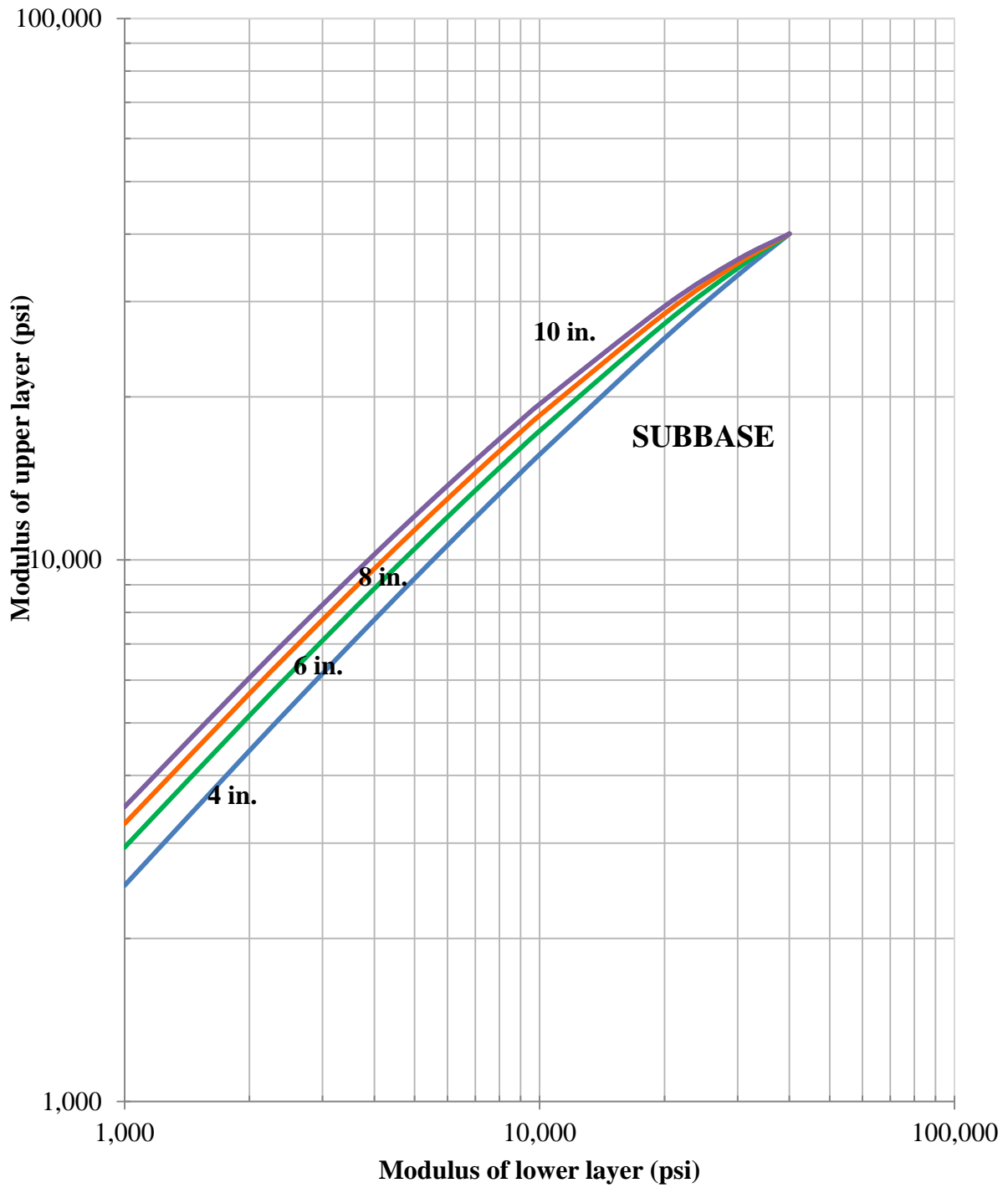
Figure 5.3 Limiting Modulus Criteria of Unbound Subbase Layers
