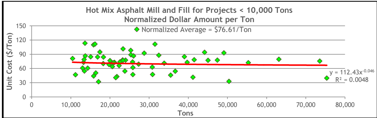
Figure 13.47 HMA Mill and Fill Normalized Unit Costs for Projects Less than 10,000 Tons
