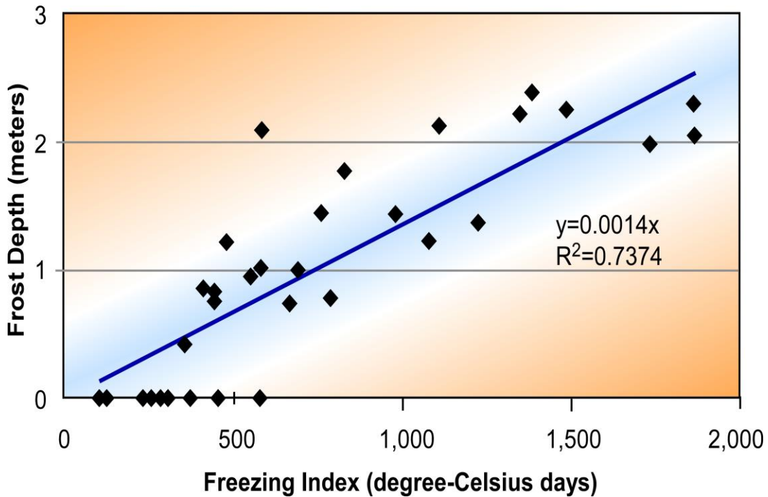
Figure 4.10 Frost Depth to FI
