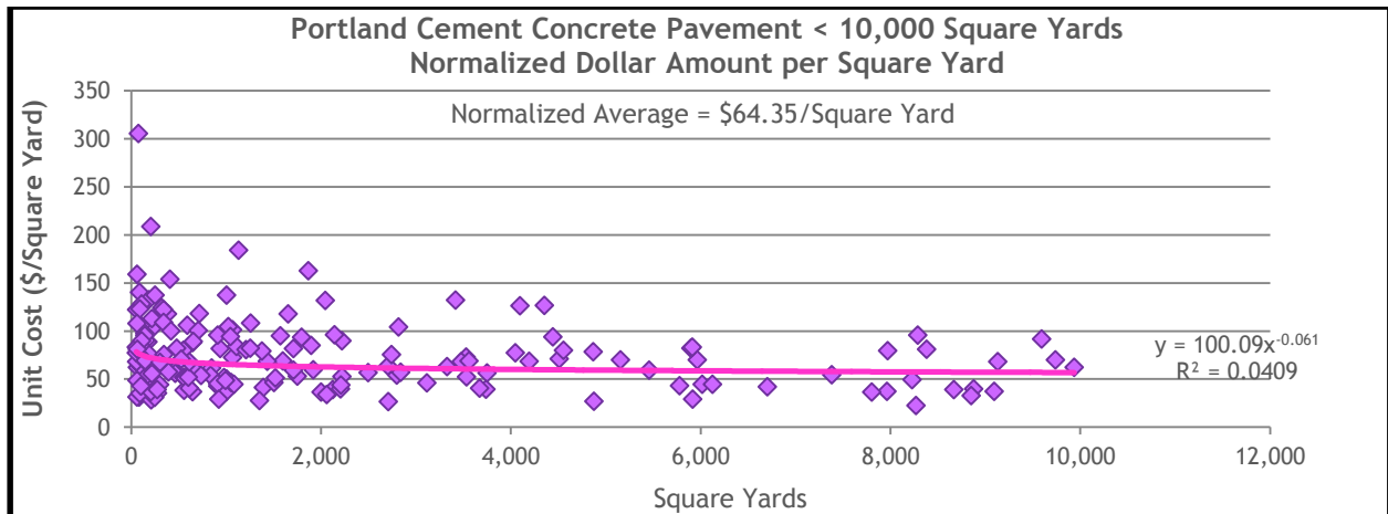
Figure 13.16 PCCP Normalized Dollar Amount per Total Square Yards for Projects Less Than 10,000 Square Yards
