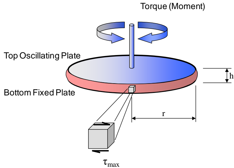
Figure S.14 Binder Complex Shear Modulus Specimen Loading
