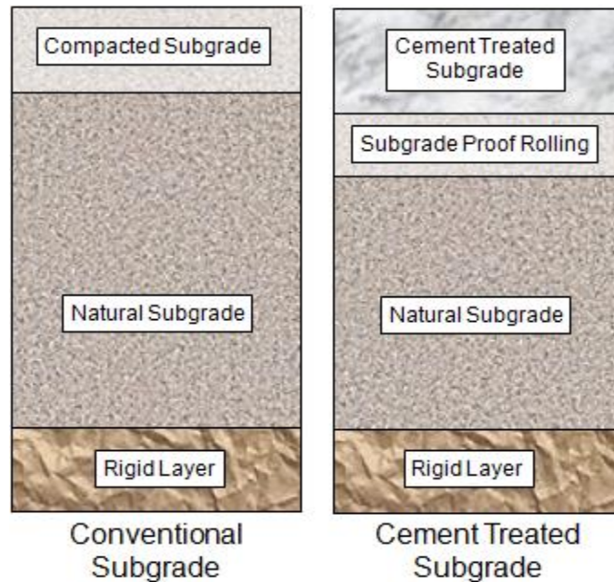
Figure 4.18 Cement Treated Structural Subgrade Layer
