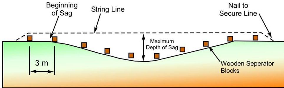
Figure 10.8 Typical Slab Raising in Slabjacking (From Figure 4-7.9 Stringline method of slab jacking Techniques for Pavement Rehabilitation 1998 (6))
