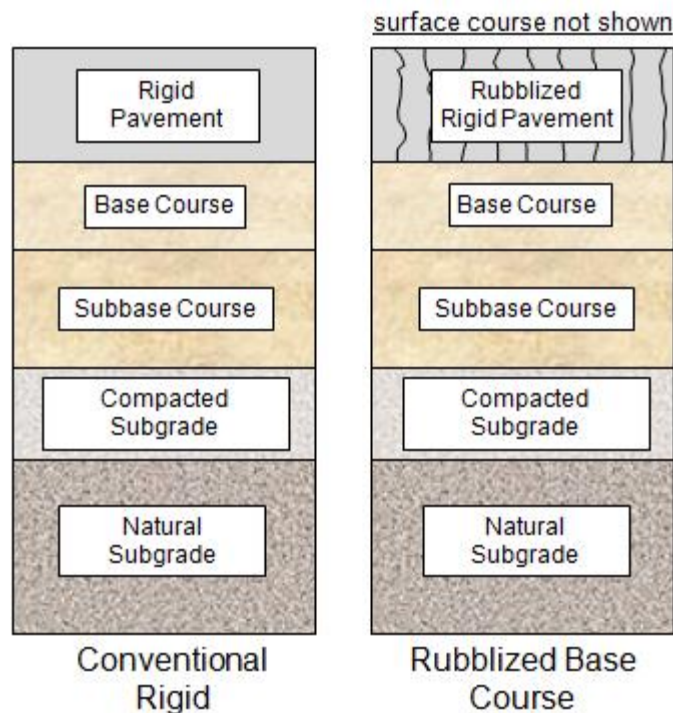
Figure 5.8 Rubblized Base Course
