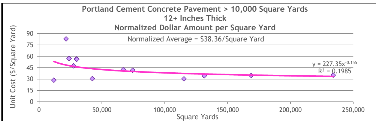
Figure 13.28 PCCP Normalized Dollar Amount for Projects of 12 Inches or Greater in Thickness and Greater Than 10,000 Square Yards in Size
