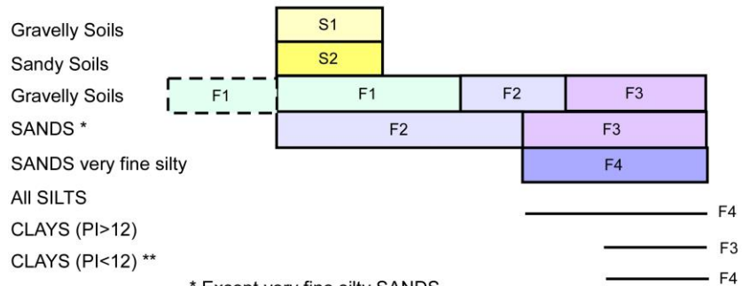
Figure 4.11 Frost Susceptible Soil Classifications
