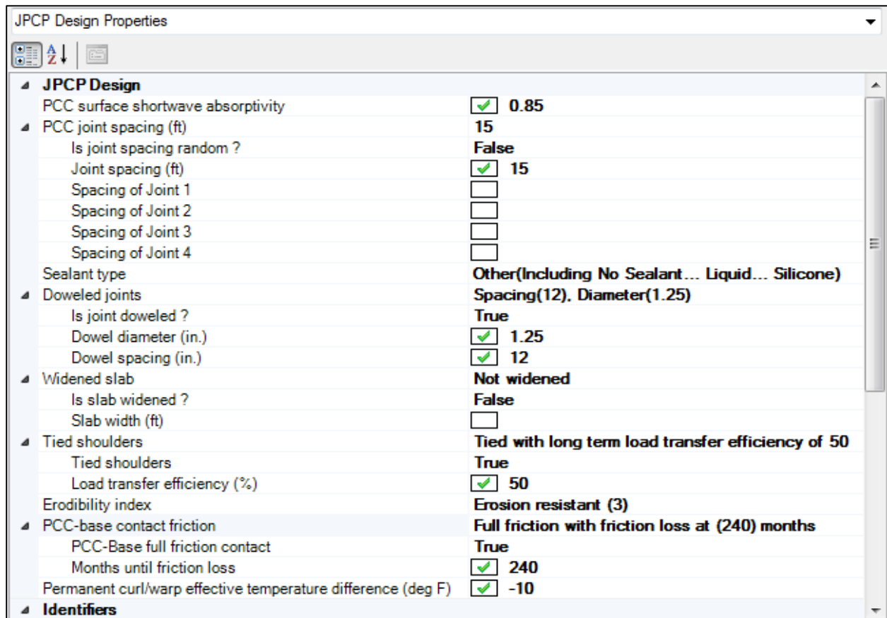
Figure 7.6 M-E Design Software Screenshot of JPCP Design Features
