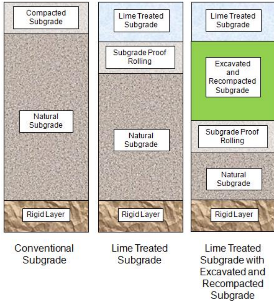
Figure 4.16 Lime Treated Structural Subgrade Layer
