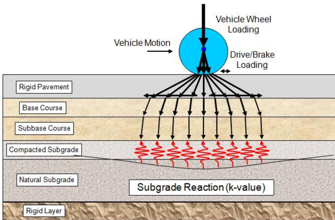
Conventional Rigid
