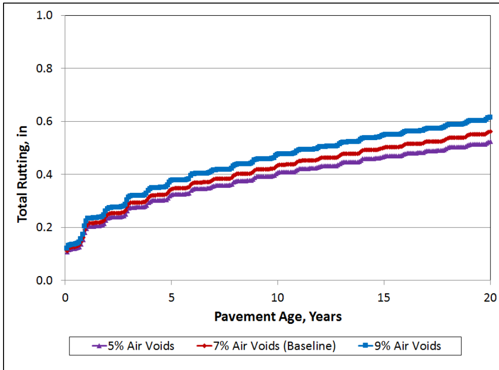
Figure 6.21 Sensitivity of Total Rutting to Air Voids
