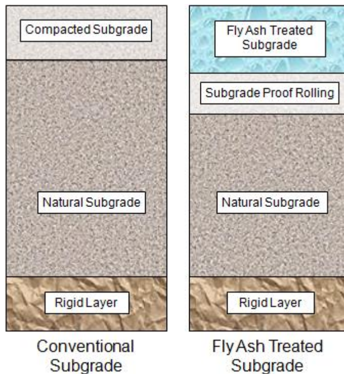
Figure 4.19 Fly Ash Treated Structural Subgrade Layer
