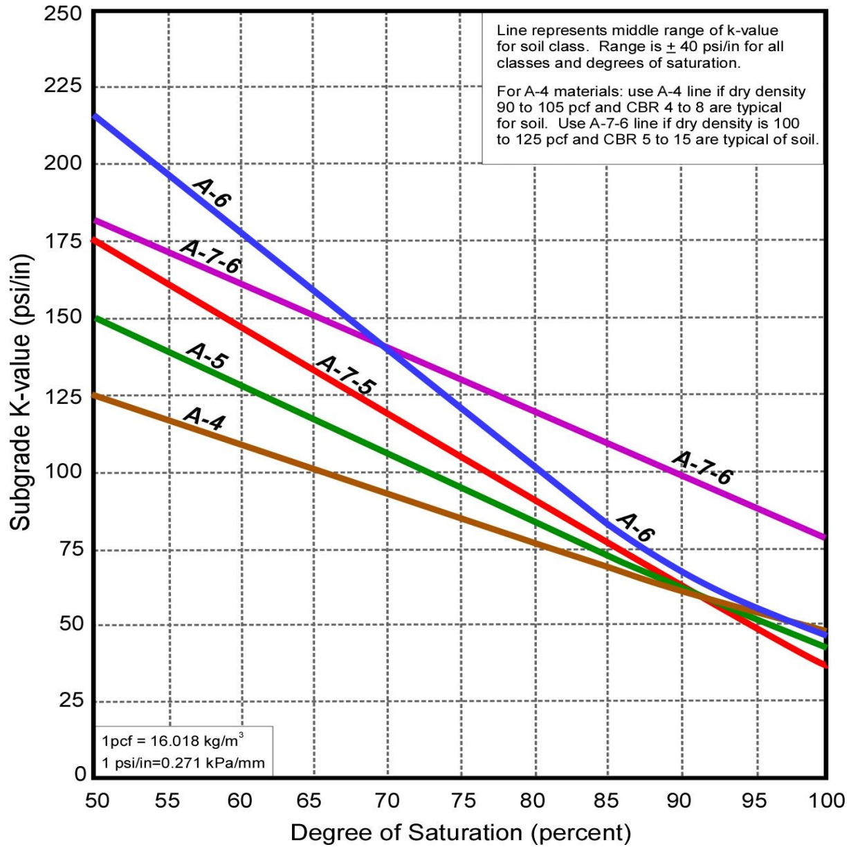
Figure 4.8 k-values vs. Degree of Saturation for A-4 Through A-7 Soils
