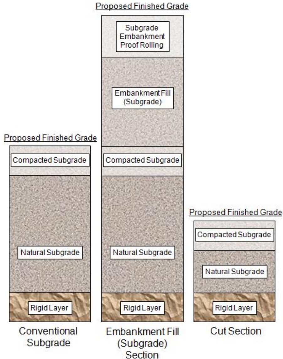
Figure 4.1 Subgrade Preparation
