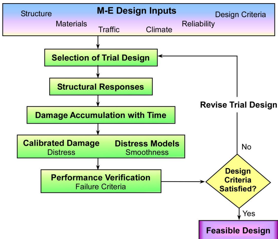
Figure 1.1 M-E Design Process
