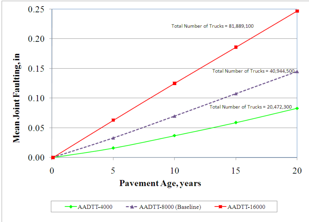
Figure 7.14 Sensitivity of JPCP Faulting to Traffic Volume
