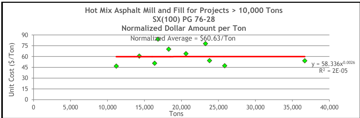
Figure 13.52 HMA Mill and Fill Normalized Unit Costs for SX(100) PG 76-28 on Projects Greater than 10,000 Tons
