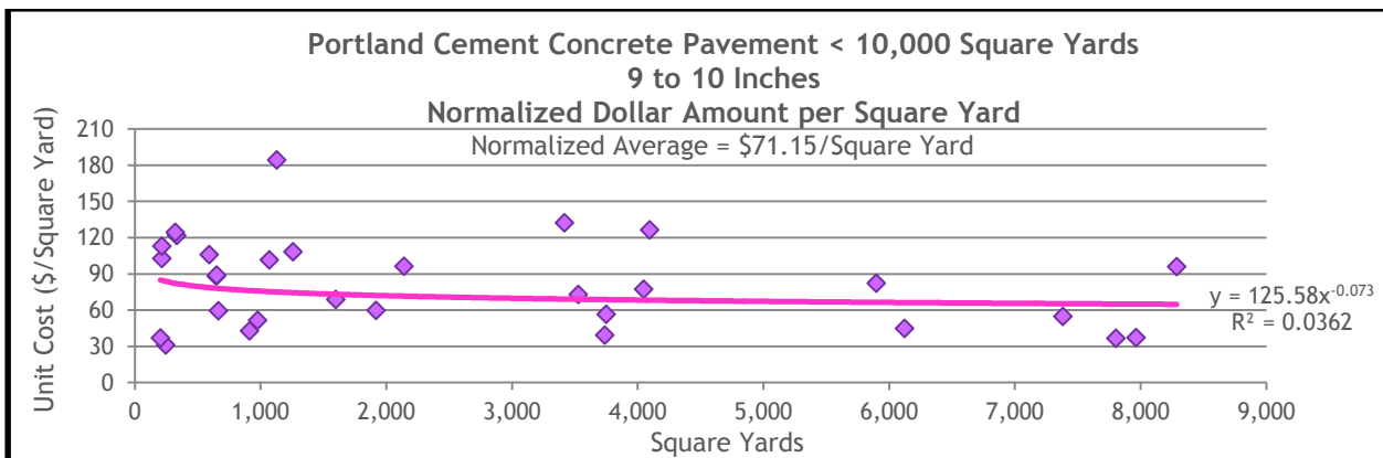
Figure 13.19 PCCP Normalized Dollar Amount for Projects of 9 to 10 Inches in Thickness and Less Than 10,000 Square Yards in Size
