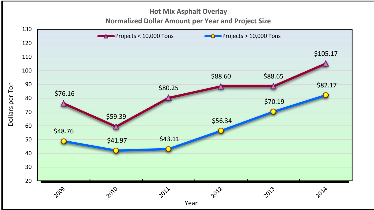
Figure 13.29 HMA Overlay Normalized Dollar per Year and Project Size
