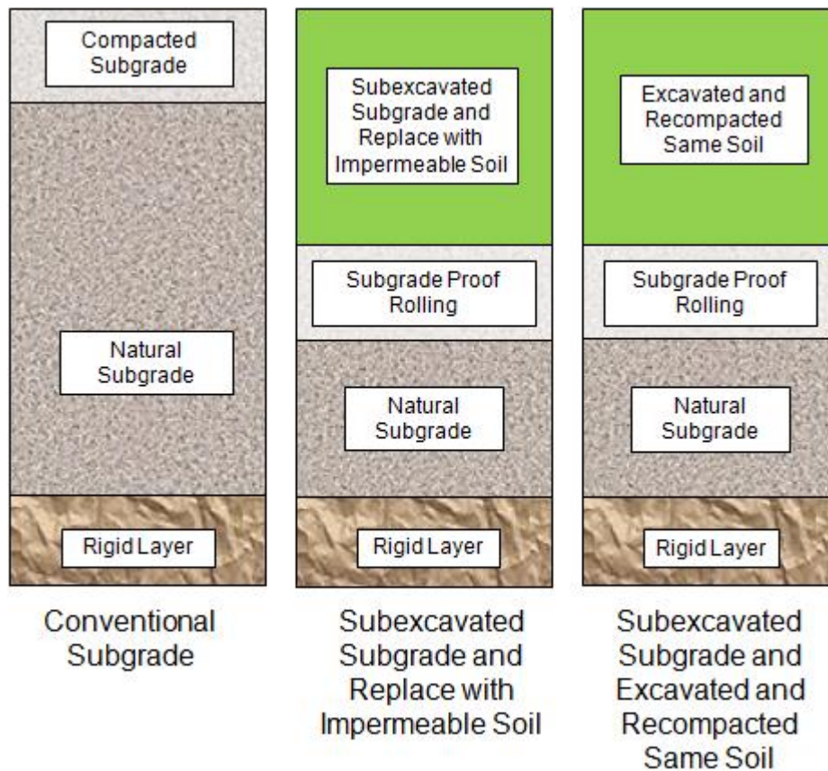
Figure 4.12 Subexcavated Subgrade Layers
