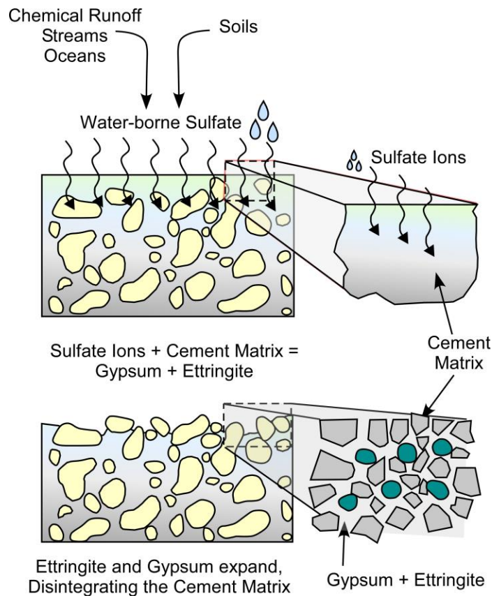
Figure 7.23 Sulfate Attack
