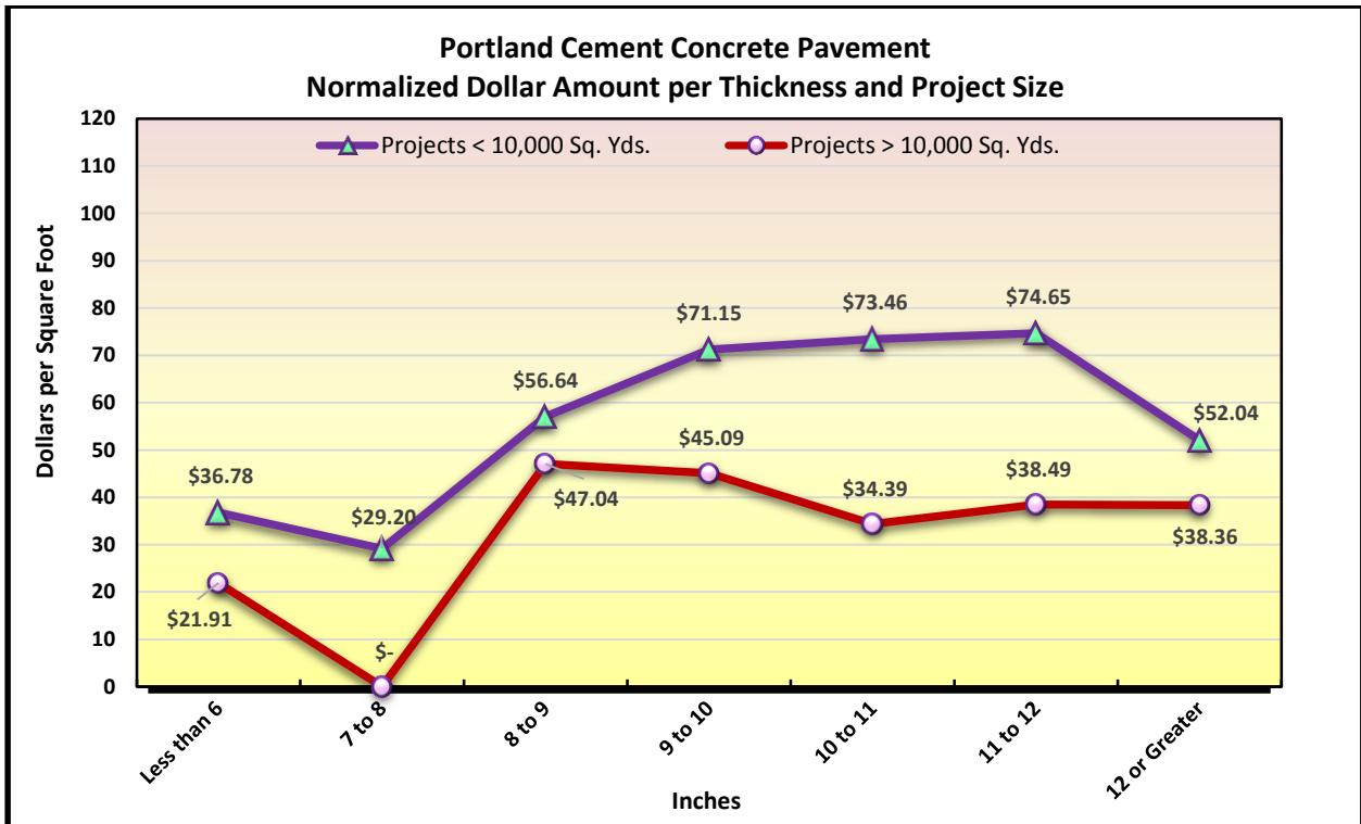
Figure 13.14 PCCP Normalized Dollar Amount per Thickness
