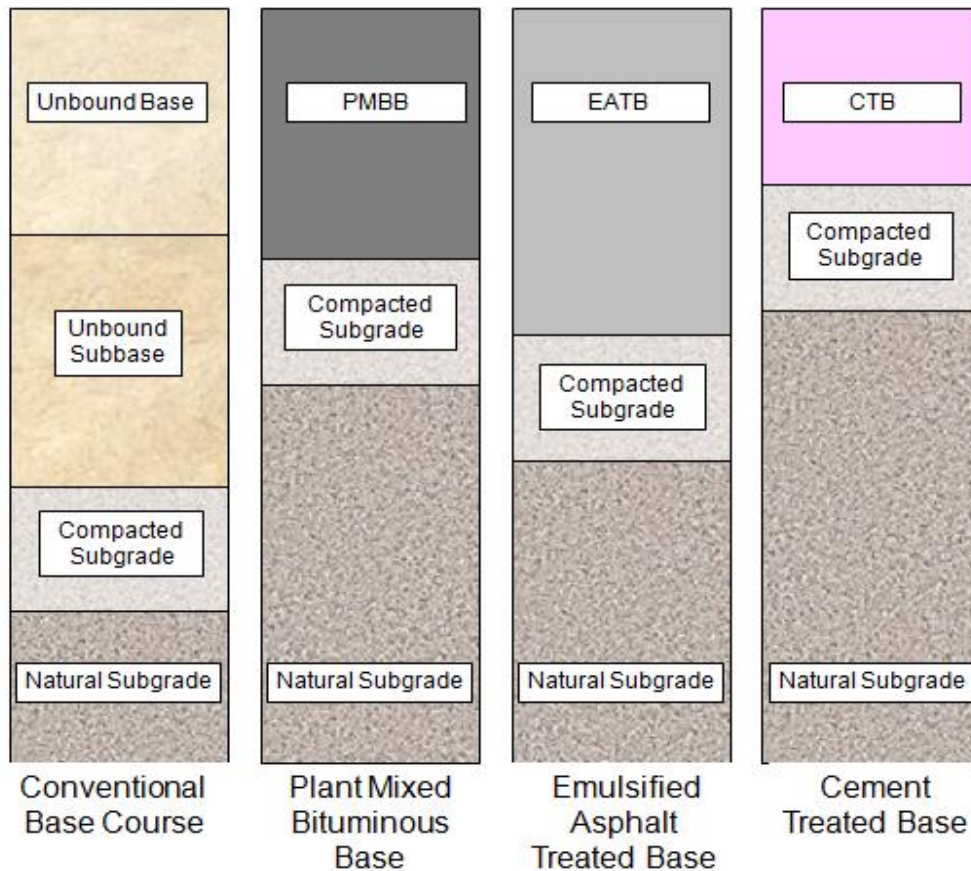
Figure 5.4 Stabilized Treated Structural Base Layers
