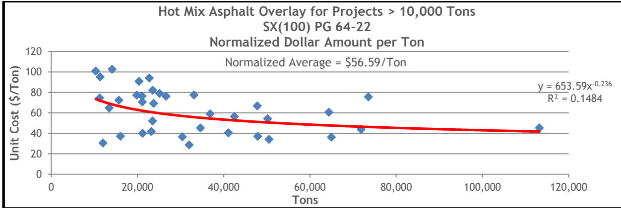
Figure 13.39 HMA Overlay Normalized Unit Costs for SX(100) PG 64-22 on Projects Greater than 10,000 Tons
