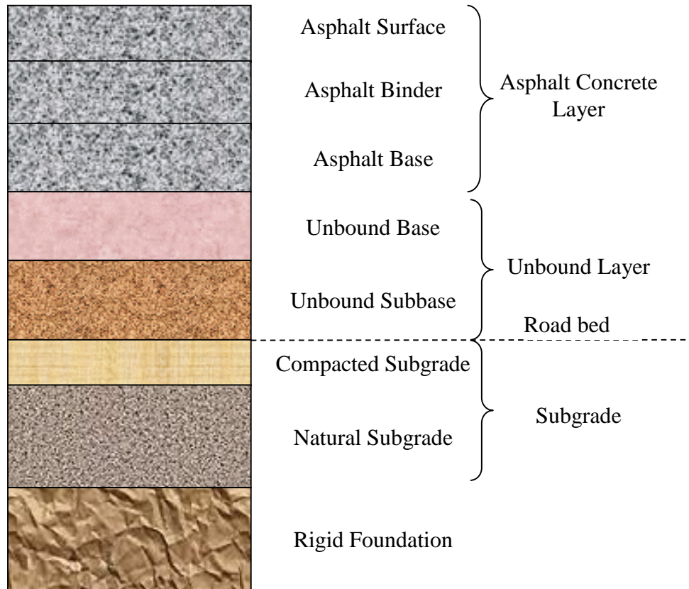
Figure 6.2 Structural Layers
