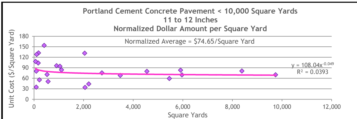
Figure 13.21 PCCP Normalized Dollar Amount for Projects of 11 to 12 Inches in Thickness and Less Than 10,000 Square Yards in Size
