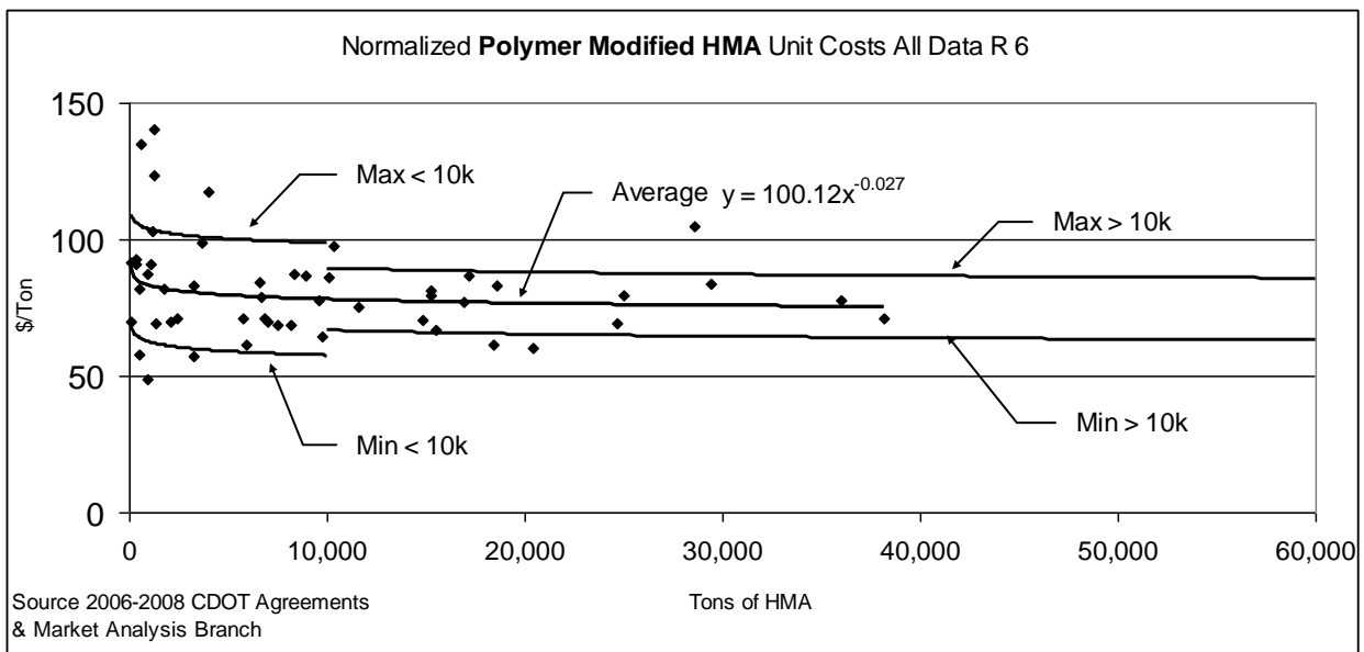
Figure 10.37 Polymer Modified HMA Unit Costs (Region 6 (prior to 7/1/2013))
