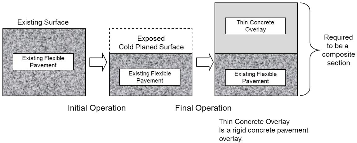
Figure 6.3 Thin Concrete Overlay Layer
