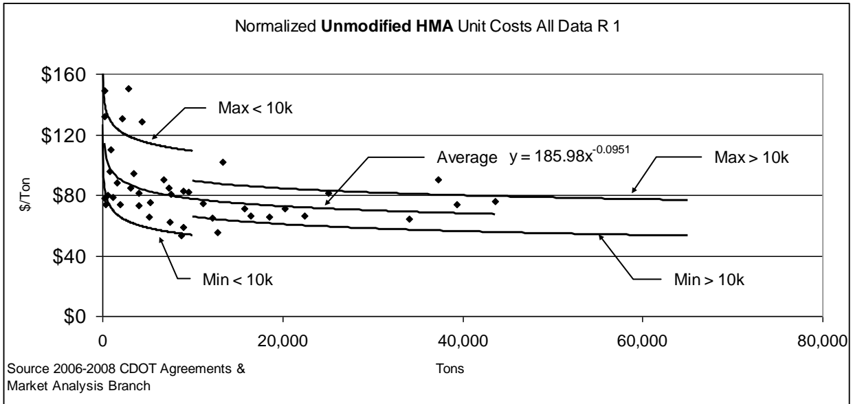
Figure 10.23 Unmodified HMA Unit Costs (Region 1 (prior to 7/1/2013))
