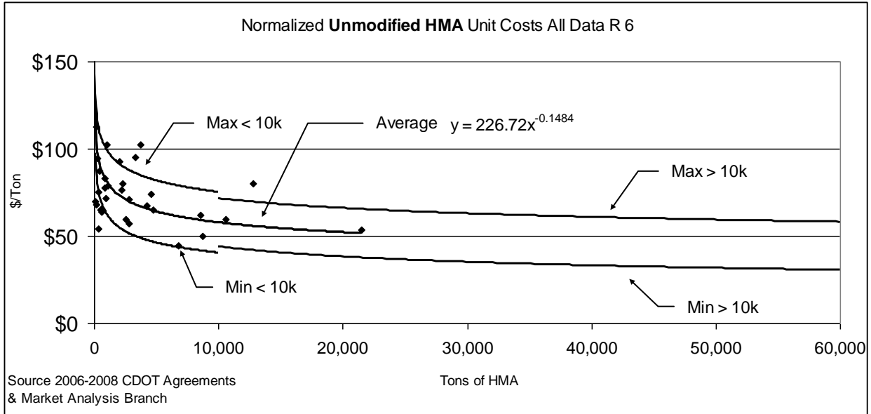
Figure 10.36 Unmodified HMA Unit Costs (Region 6 (prior to 7/1/2013))
