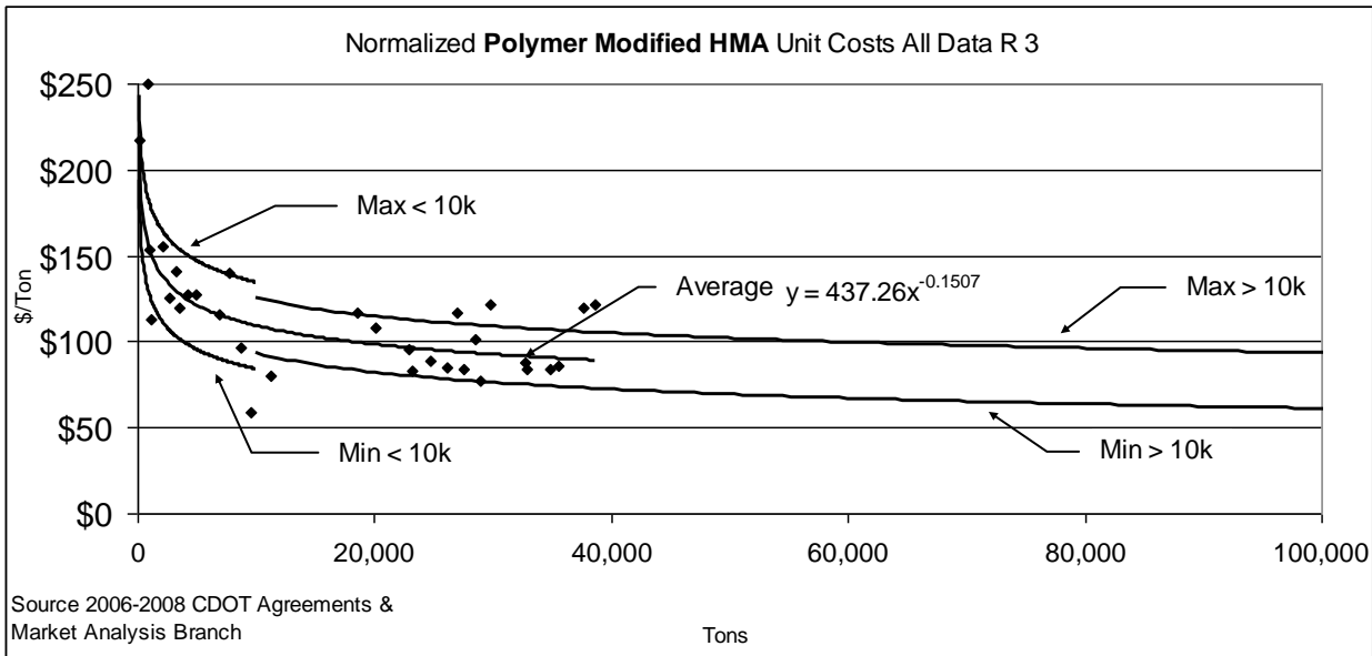
Figure 10.29 Polymer Modified HMA Unit Costs (Region 3 (prior to 7/1/2013))
