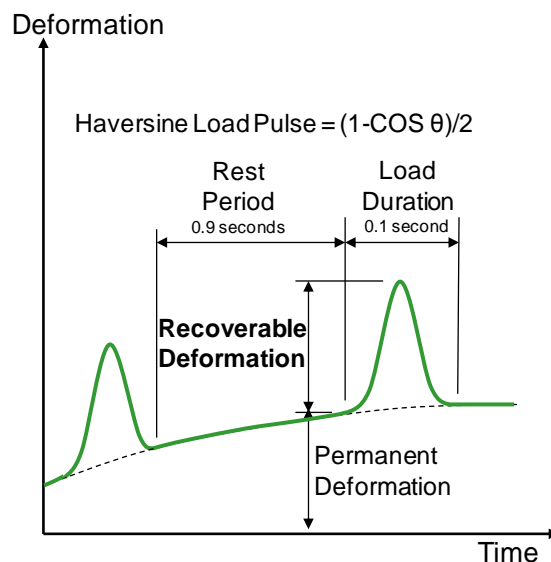
Figure S.24 Resilient Modulus Test Specimen Loading
