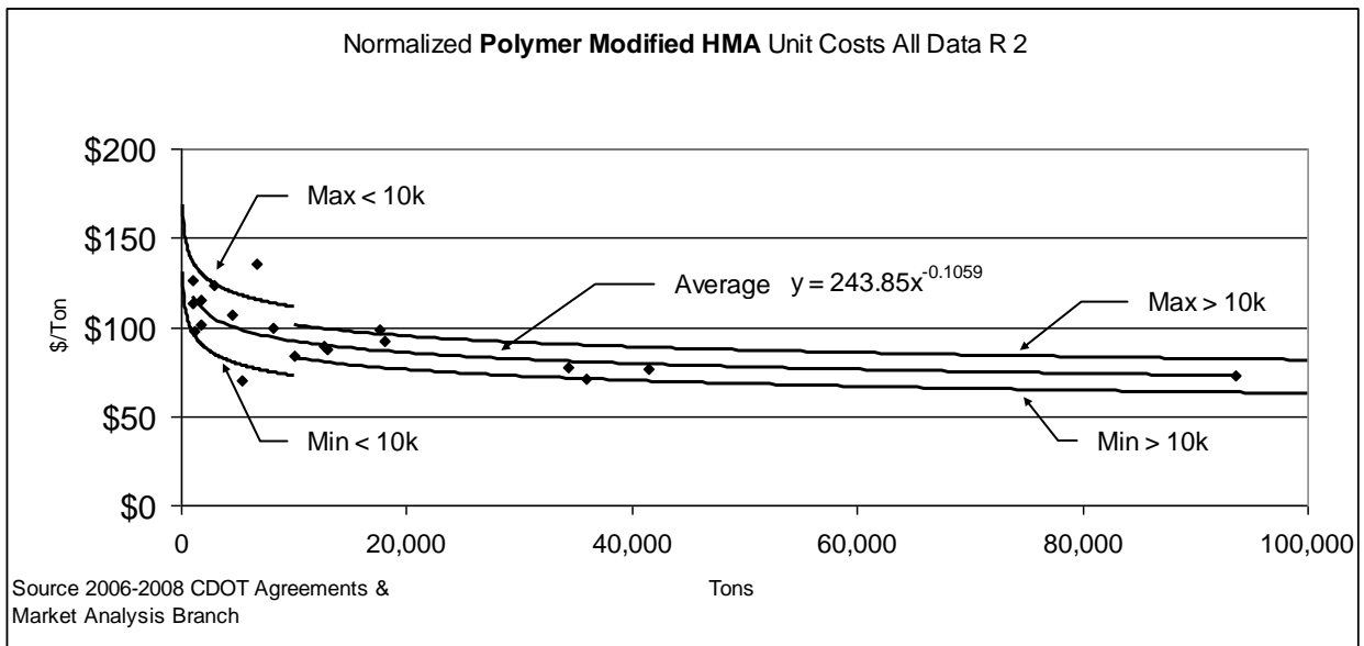
Figure 10.27 Polymer Modified HMA Unit Costs (Region 2 (prior to 7/1/2013))
