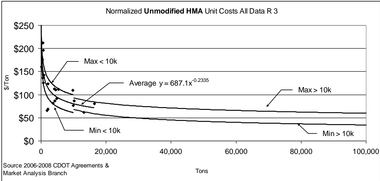
Figure 10.28 Unmodified HMA Unit Costs (Region 3 (prior to 7/1/2013))
