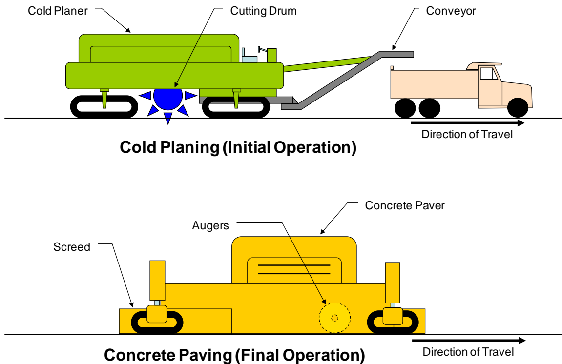
Figure 6.4 Schematic of Thin Concrete Overlay Equipment
