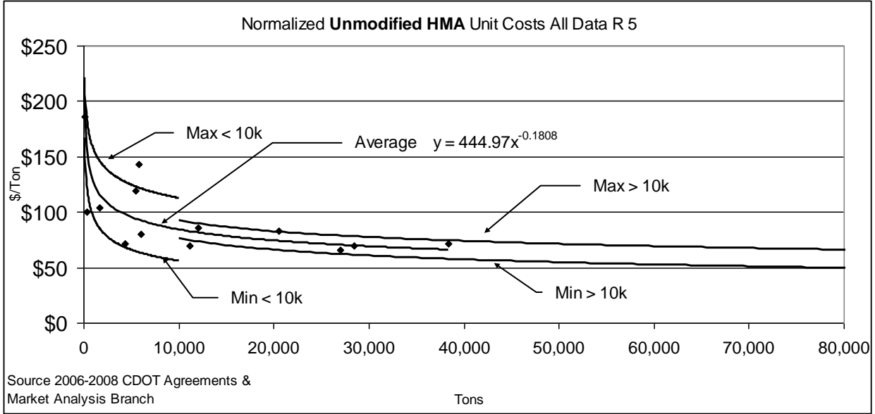
Figure 10.33 Unmodified HMA Unit Costs (Region 5 (prior to 7/1/2013))
