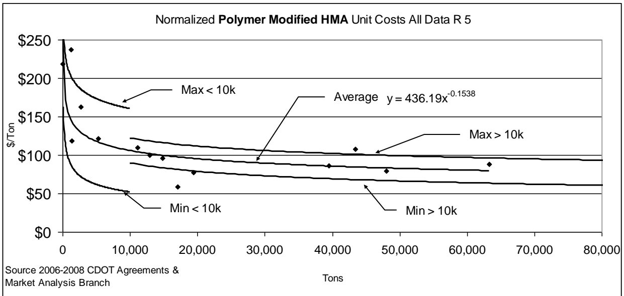
Figure 10.34 Polymer Modified HMA Unit Costs (Region 5 (prior to 7/1/2013))
