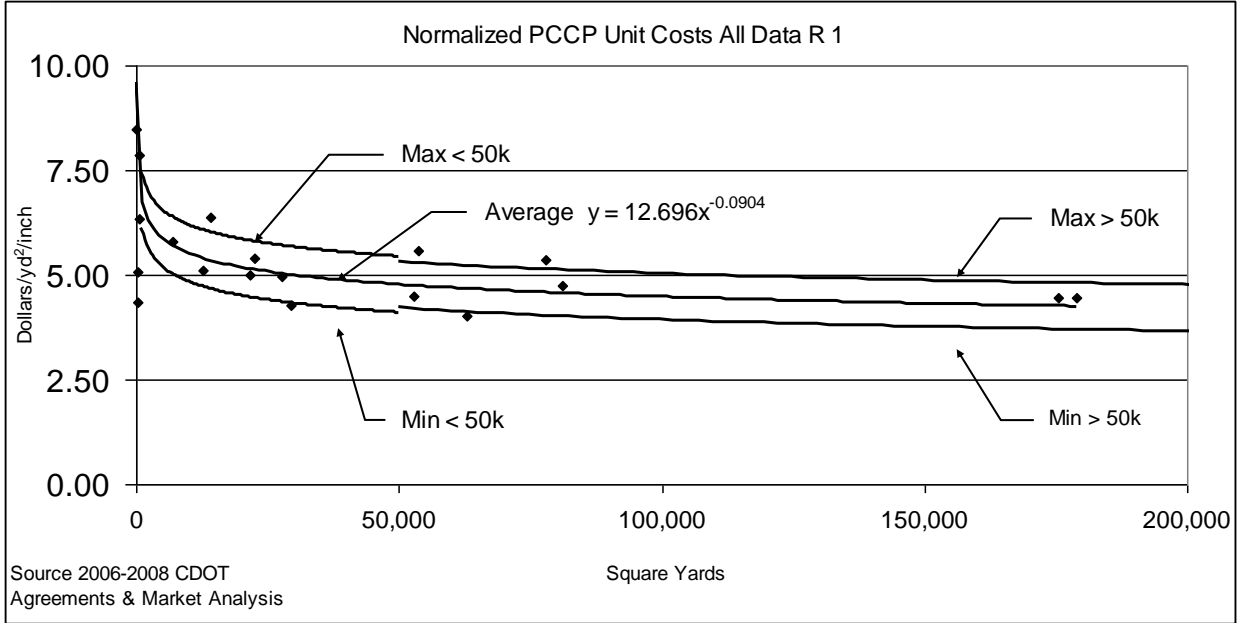
Figure 10.22 PCCP Unit Costs (Region 1 (prior to 7/1/2013))
