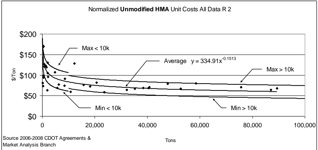
Figure 10.26 Unmodified HMA Unit Costs (Region 2 (prior to 7/1/2013))
