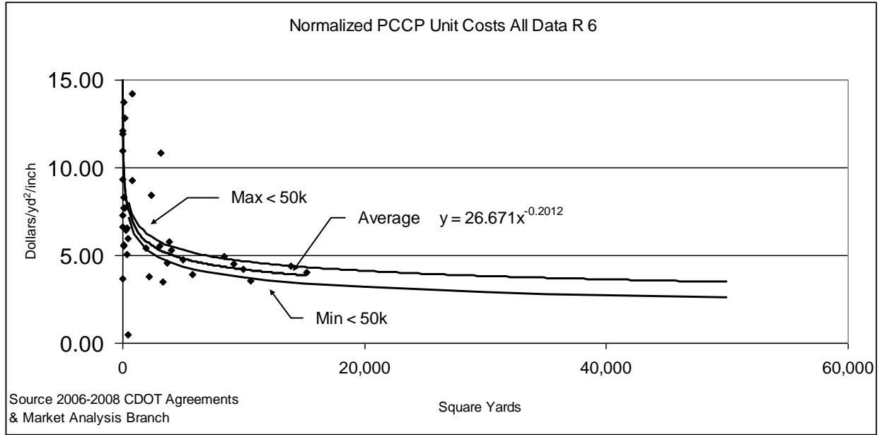
Figure 10.35 PCC Unit Costs (Region 6 (prior to 7/1/2013))
