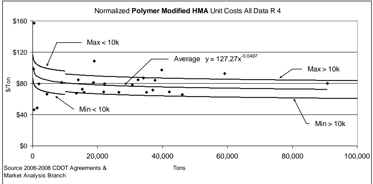
Figure 10.32 Polymer Modified HMA Unit Costs (Region 4 (prior to 7/1/2013))
