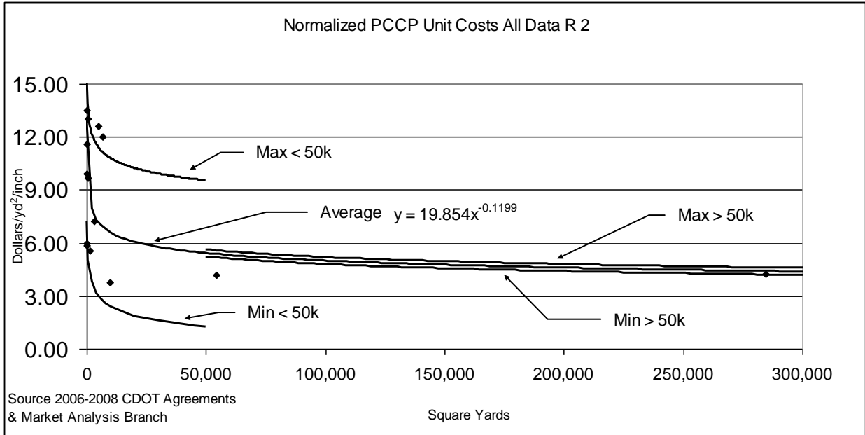
Figure 10.25 PCCP Unit Costs (Region 2 (prior to 7/1/2013))
