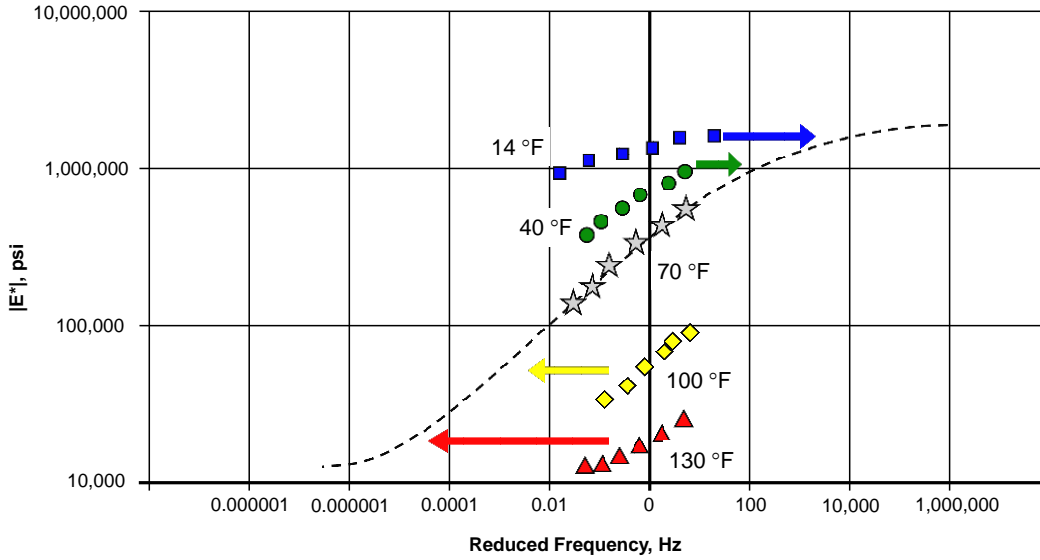
Figure S.11 Shifting of Various Mixture Plots
