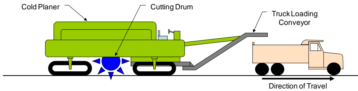
Figure 5.8 Schematic of Cold Planing Equipment
