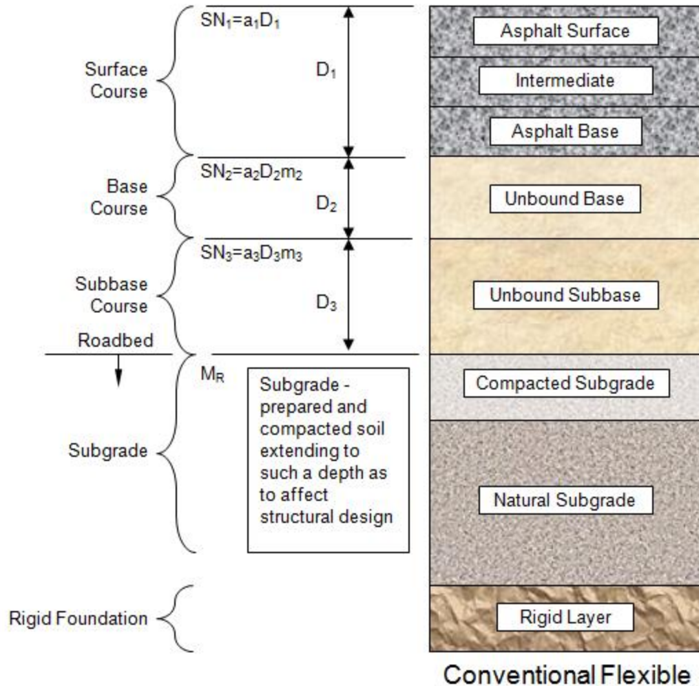
Figure 3.2 Structural Layers
