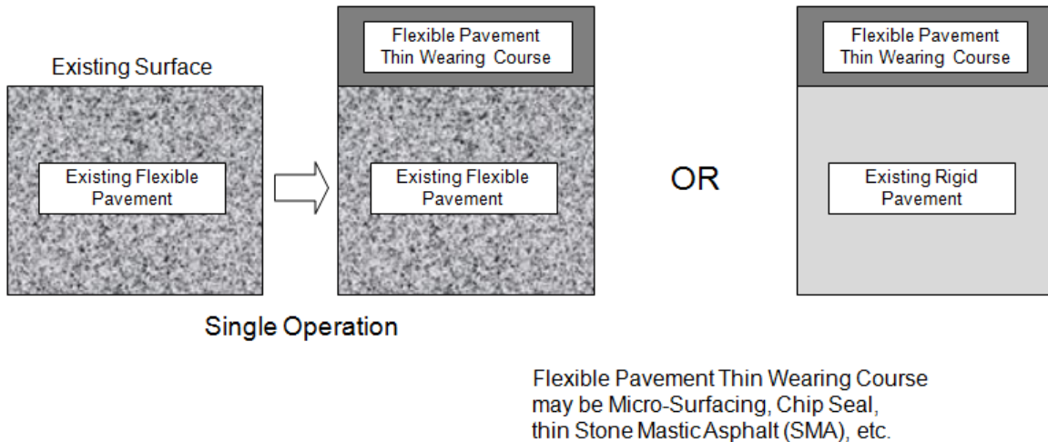
Figure 5.3 Thin Wearing Course Treatment Layer
