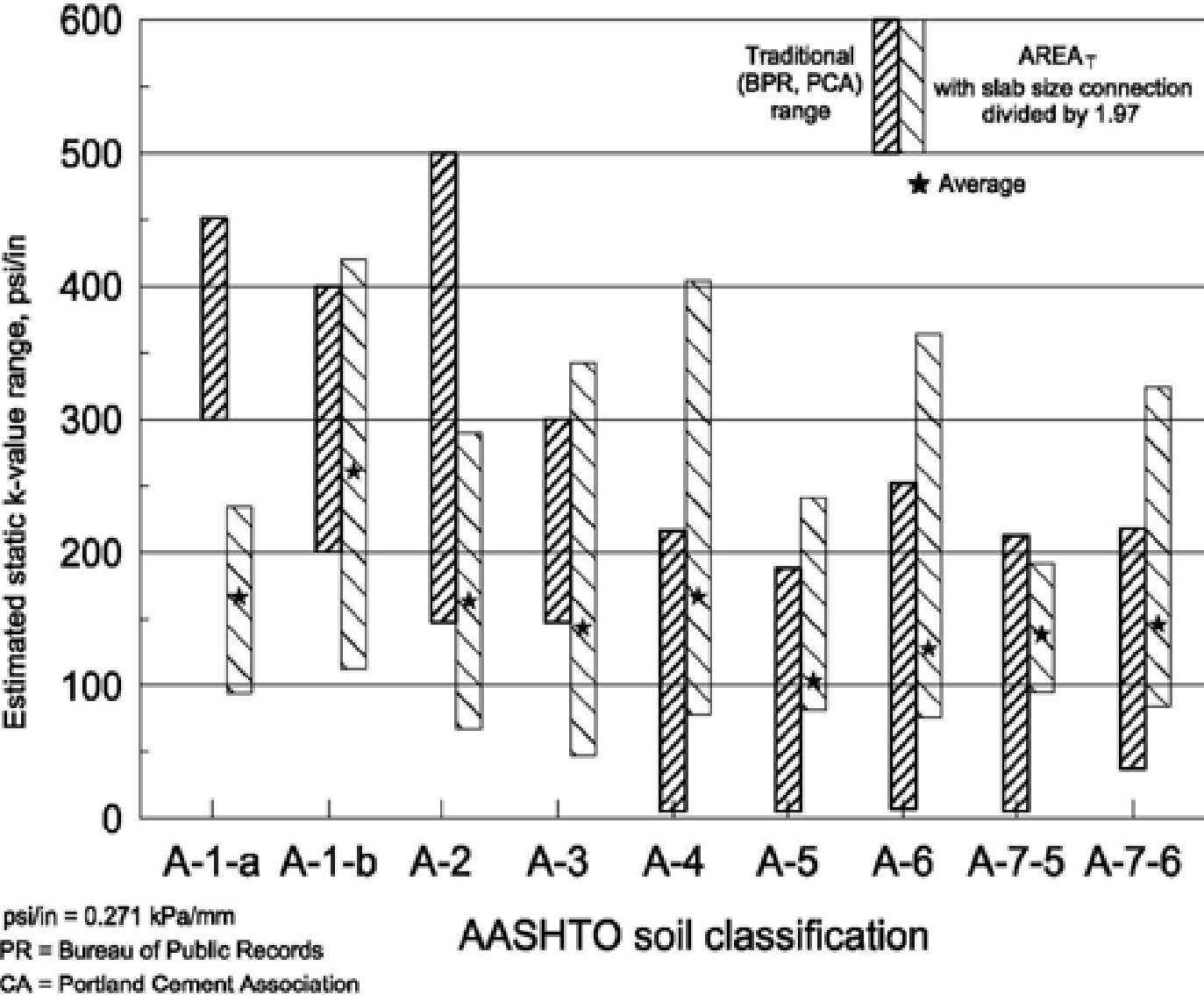
Figure 2.6 k-value vs. Soil Classification
