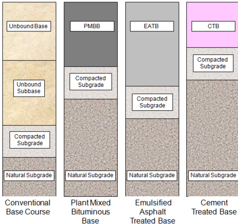
Figure 2.25 Stabilized Treated Structural Base Layers
