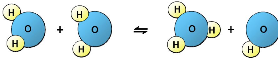
Figure S.6 Dissociation of Water
