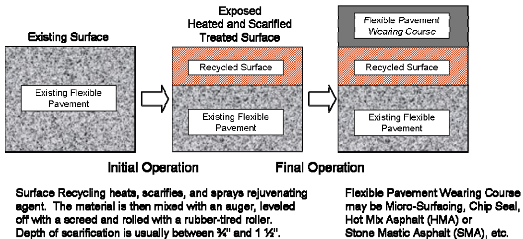
Figure 5.13 Surface Recycling Layers
