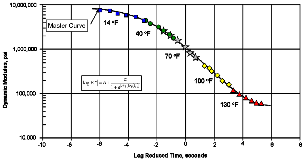
Figure S.12 Dynamic Modulus (E*) Master Curve
