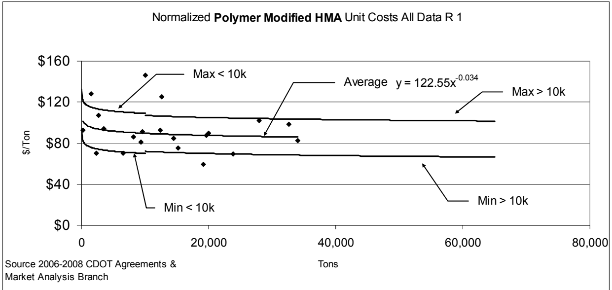
Figure 10.23 Polymer Modified HMA Unit Costs (Region 1)
