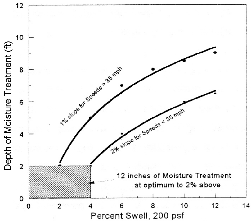
Figure 2.18 Recommended Depth of Moisture Treatment
