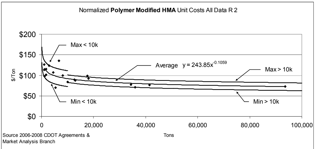
Figure 10.26 Polymer Modified HMA Unit Costs (Region 2)
