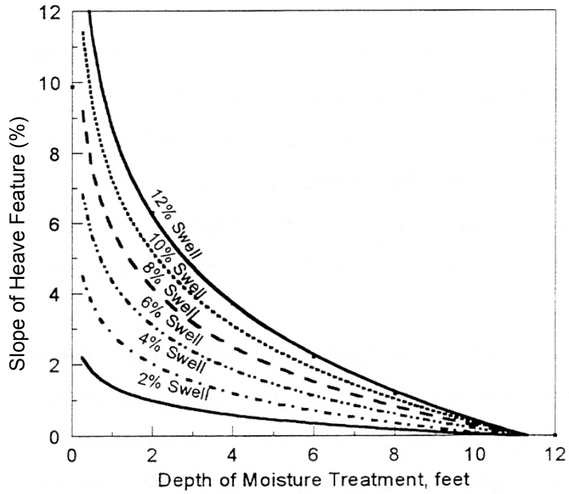
Figure 2.17 Effective Depth of Moisture Treatment
