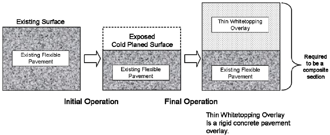
Figure 6.3 Thin Whitetopping Overlay Layer
