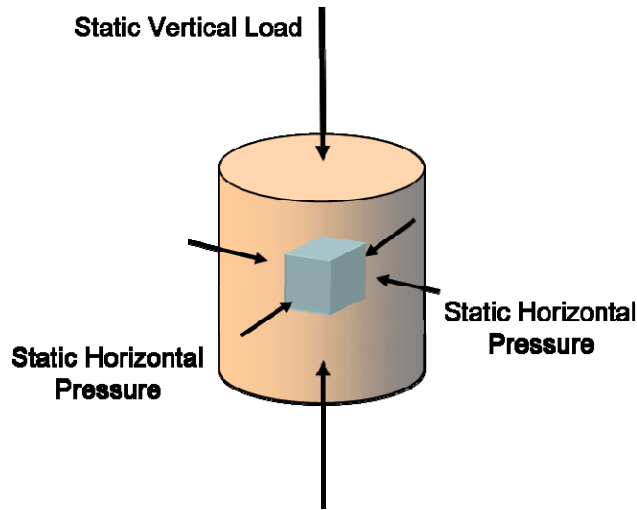
Figure S.26 Resistance R-value Test Specimen Loading State
