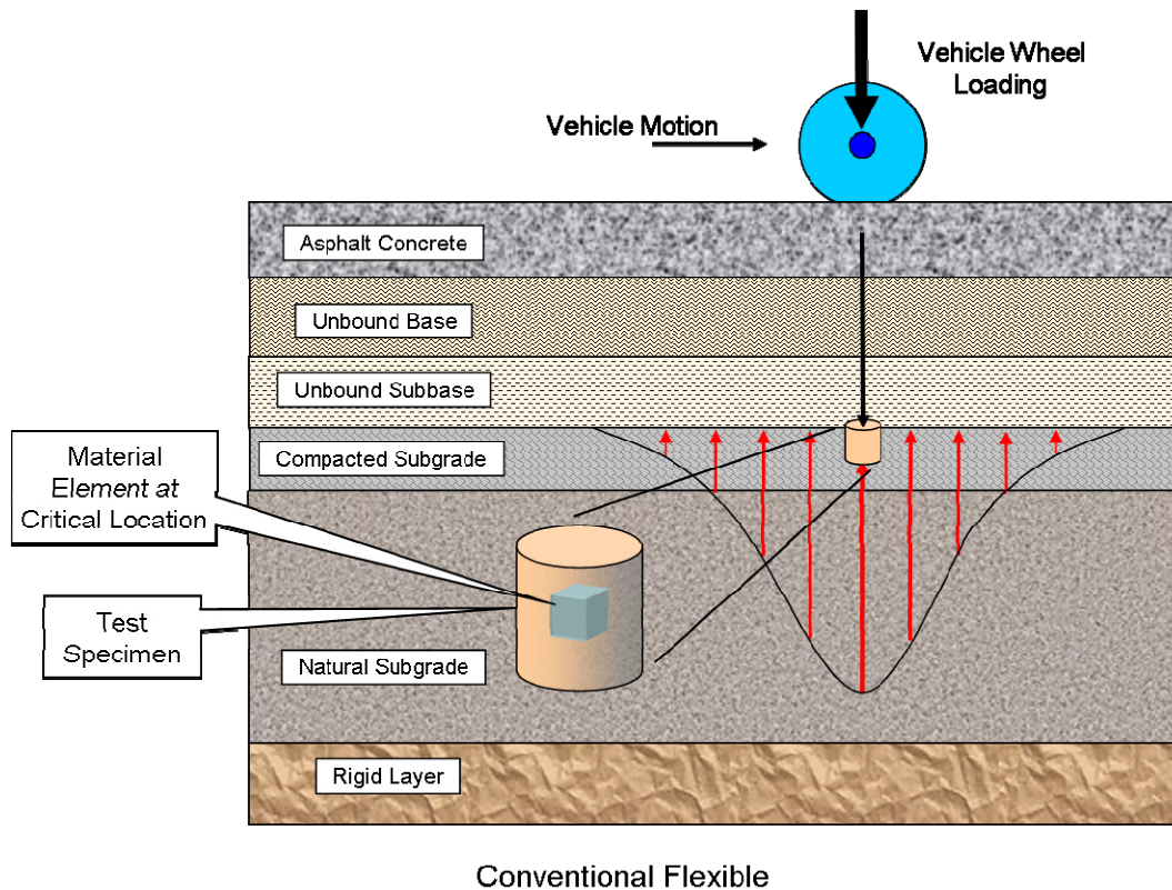
Figure S.22 Subgrade Material Element at Critical Location
