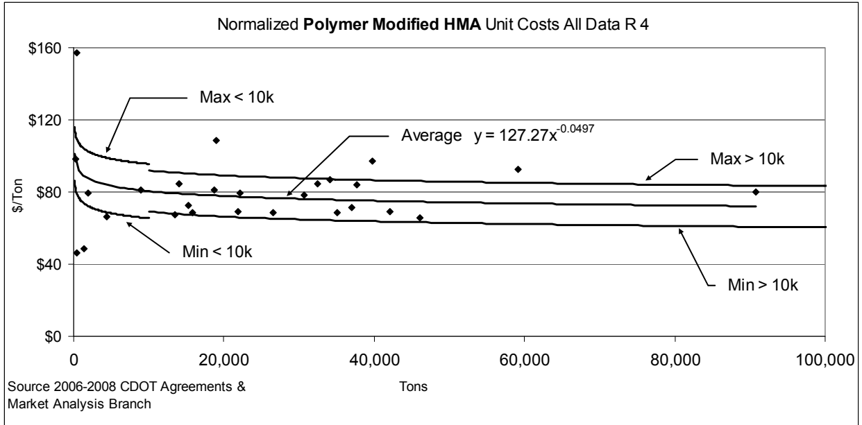
Figure 10.31 Polymer Modified HMA Unit Costs (Region 4)
