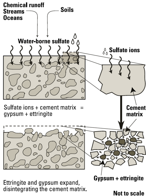
Figure 4.14 Sulfate Attack
