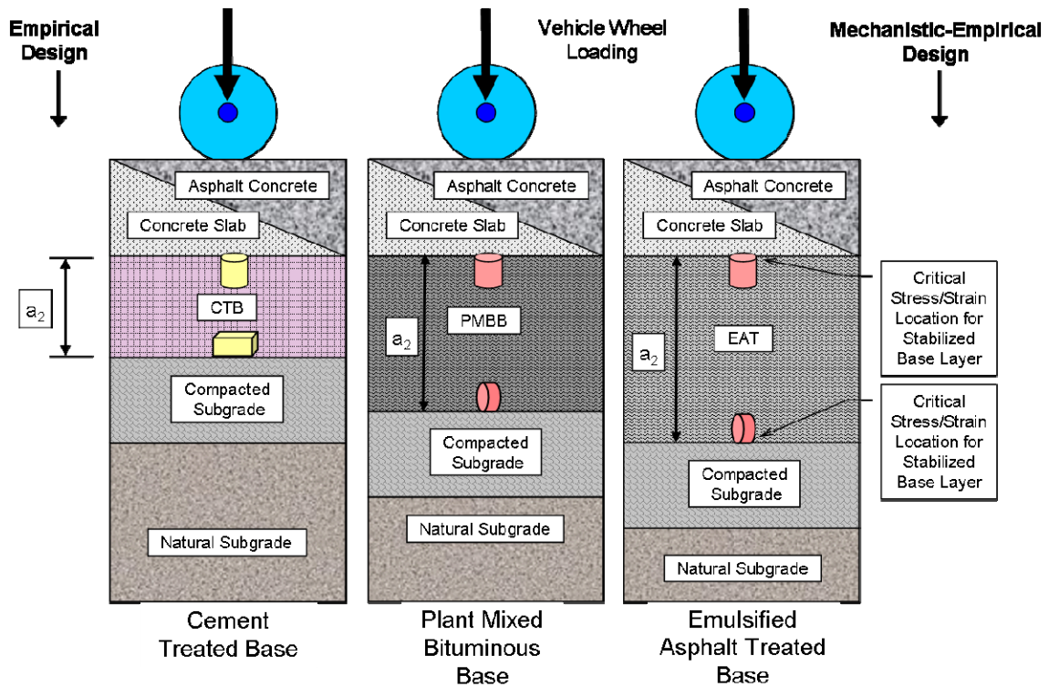
Figure S.29 Critical Stress/Strain Locations for Stabilized Bases
