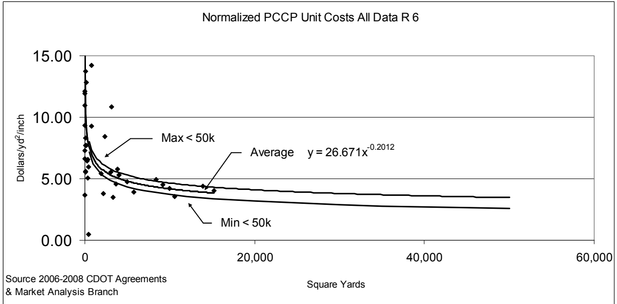
Figure 10.34 PCC Unit Costs (Region 6)
