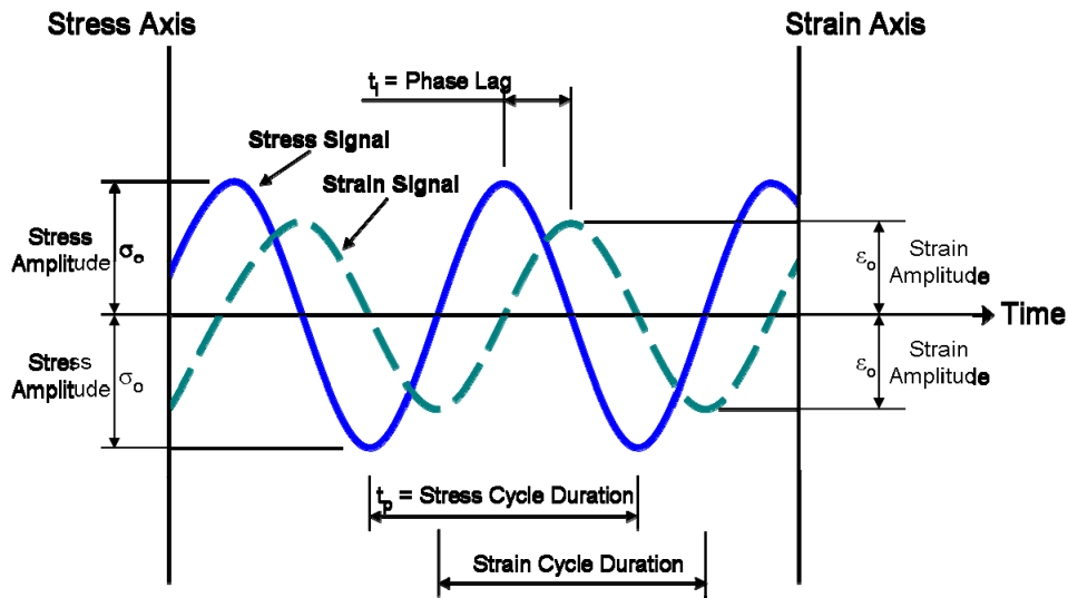
Figure S.9 Dynamic Modulus Stress-Strain Cycles
