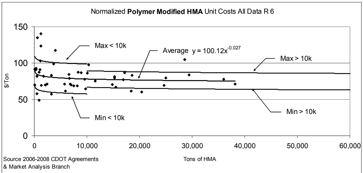
Figure 10.36 Polymer Modified HMA Unit Costs (Region 6)
