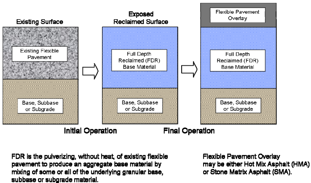
Figure 5.19 Full Depth Reclamation (FDR) Layers
