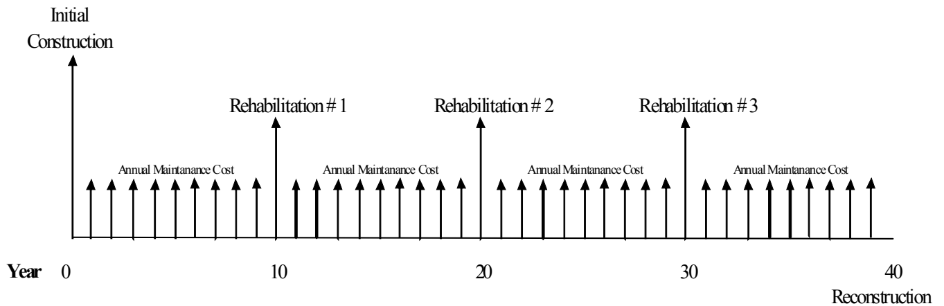
Figure 10.2 Unmodified HMA Cash Flow Diagram
