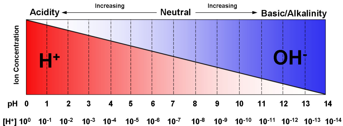
Figure S.7 pH Scale
