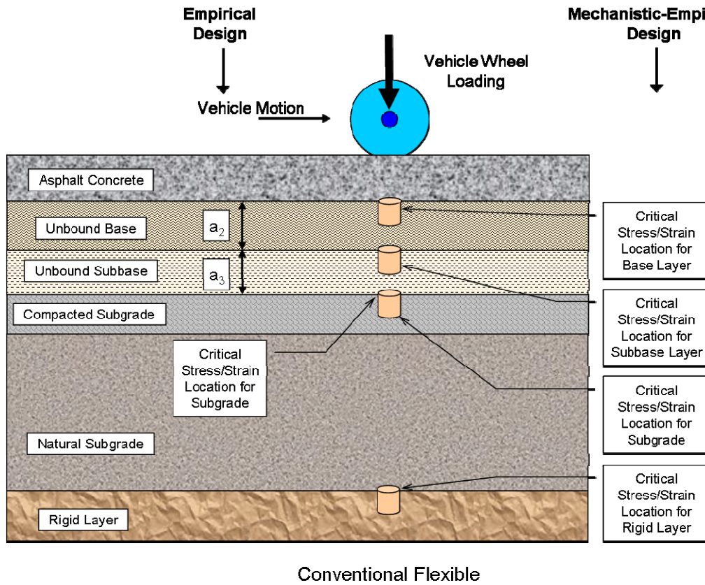
Figure S.21 Critical Stress/Strain Locations for Bases, Subbases, Subgrade, and Rigid Layer
