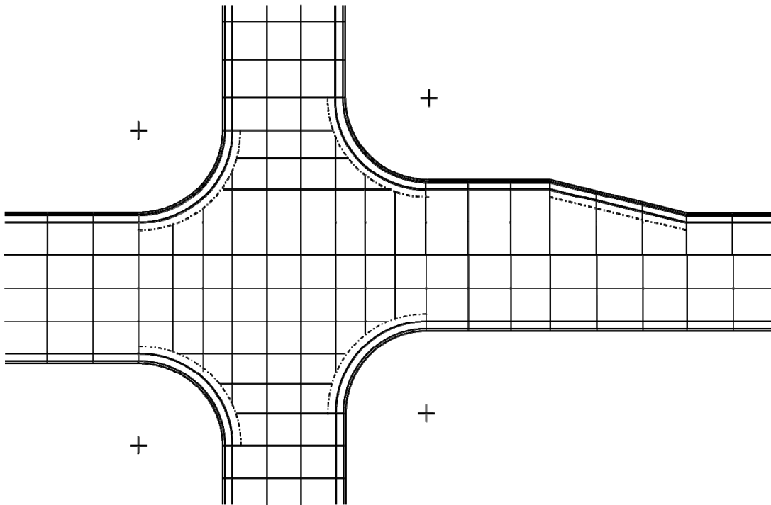
Figure 9.8 Typical Joint Layout for a Rigid Pavement Intersection (Shows lane configuration, Steps 9)
