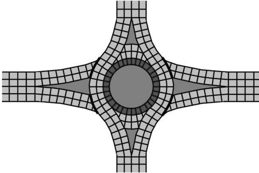
Figure 9.12 Pavement Joint Layout
