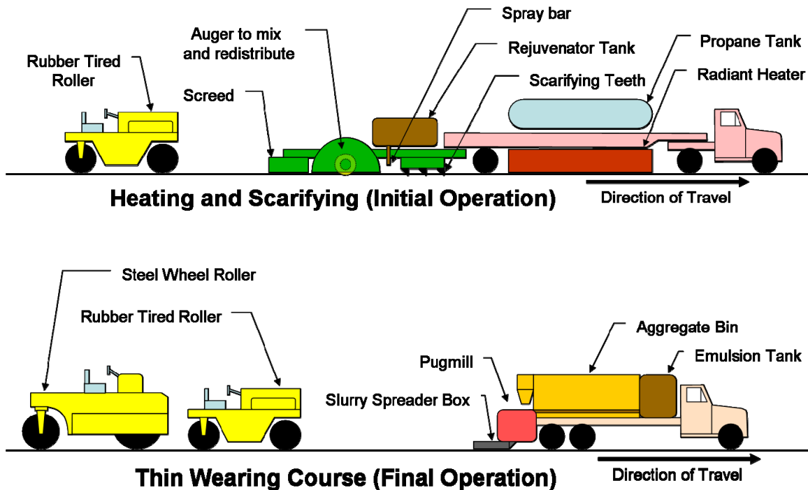
Figure 5.14 Schematic of Surface Recycling Equipment
