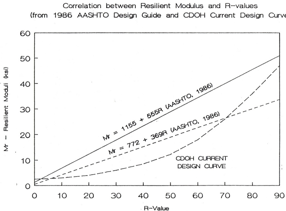
Figure S.27 Correlation Plot between Resilient Modulus and R-value ( Resilient Properties of Colorado Soils , pg 15, Figure 2.10, 1989 (6))
