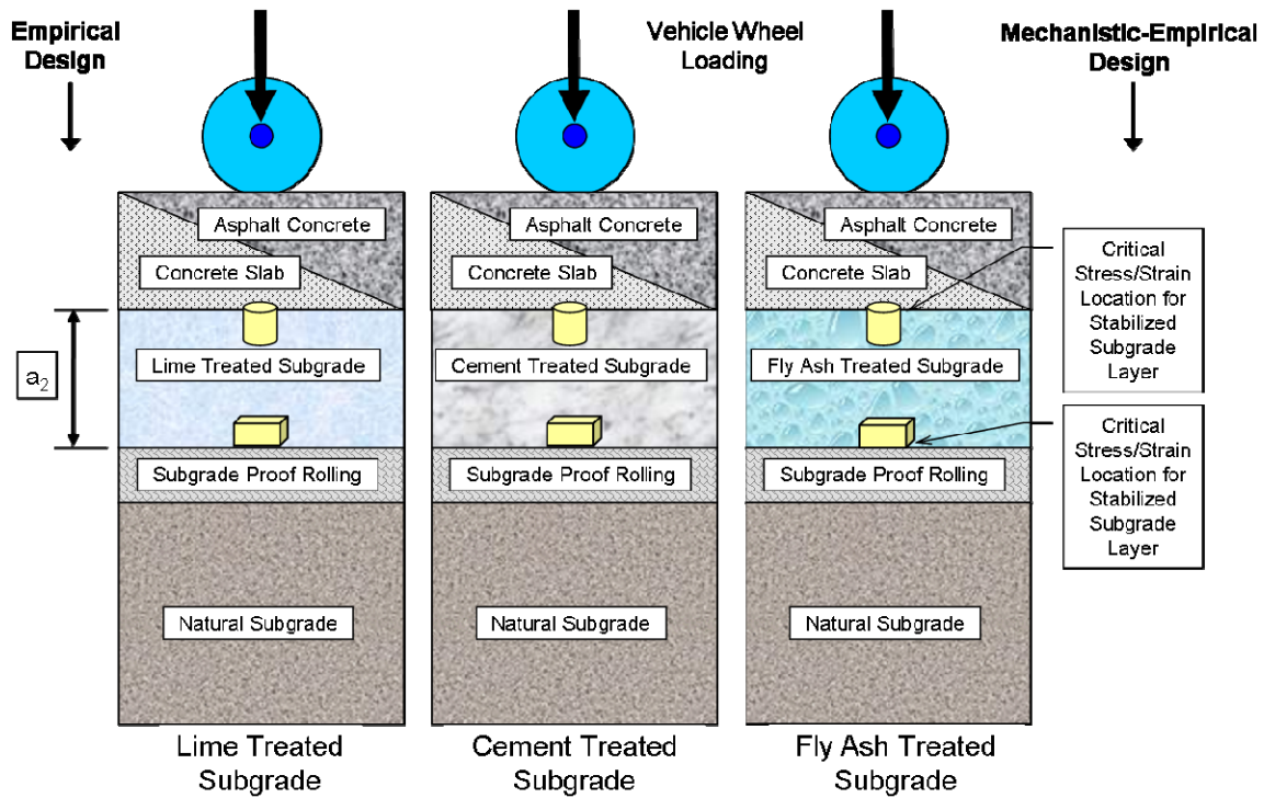
Figure S.28 Critical Stress Locations for Stabilized Subgrade
