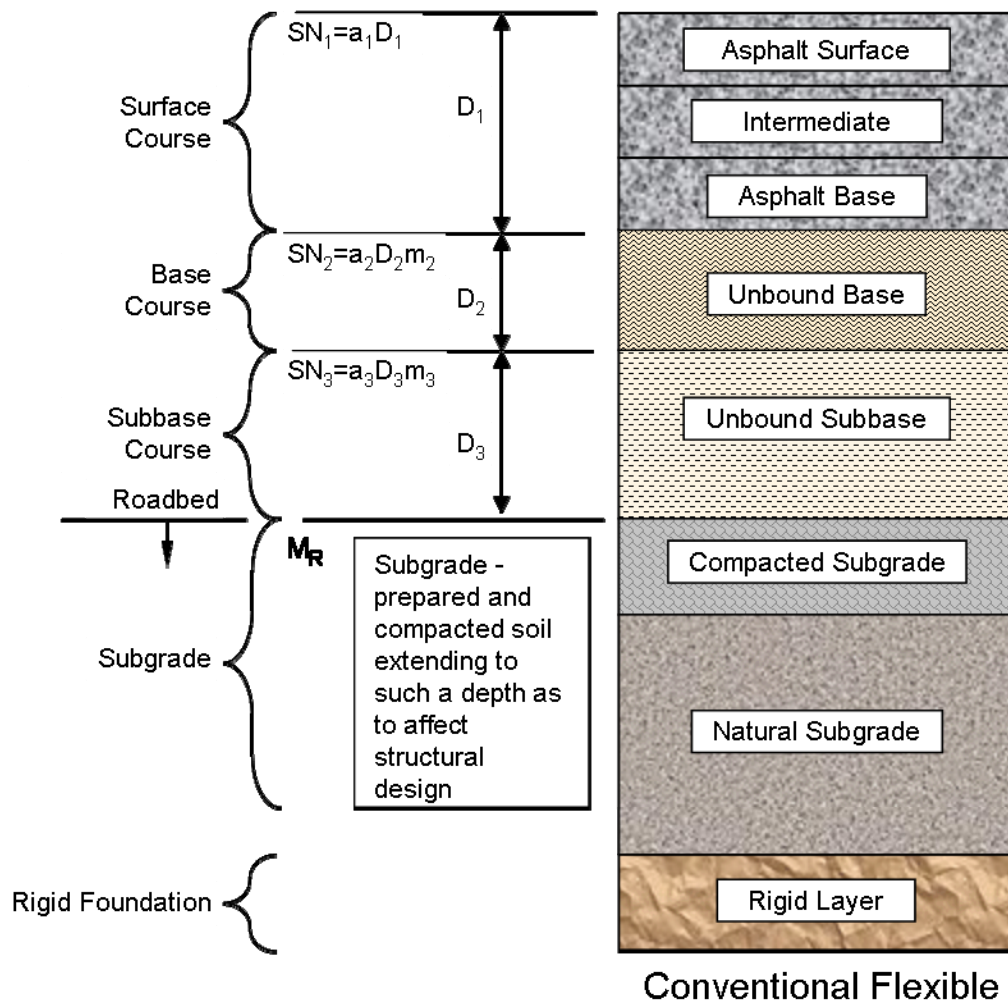
Figure 3.2 Structural Layers
