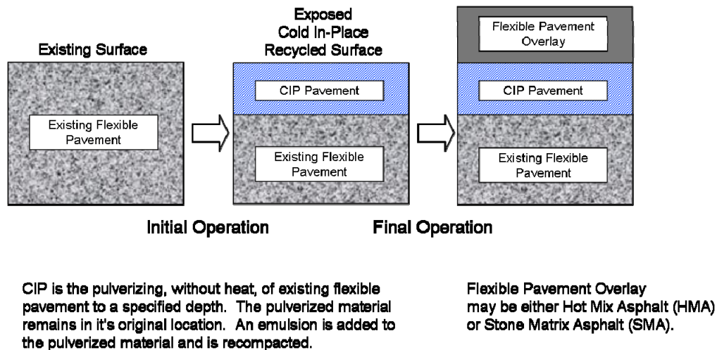
Figure 5.11 Cold In-Place Recycling Layers
