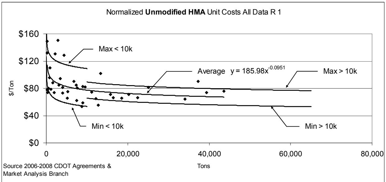
Figure 10.22 Unmodified HMA Unit Costs (Region 1)
