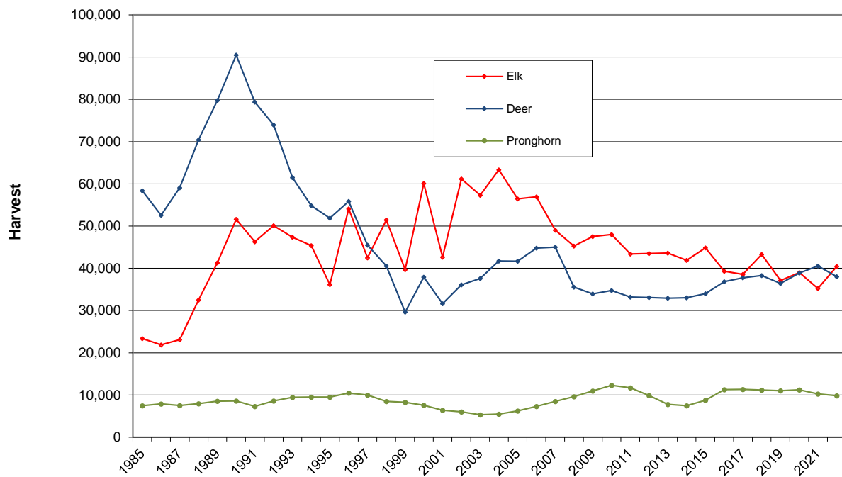
Figure 2. Elk, deer, and pronghorn harvest from 1985 to 2022.
