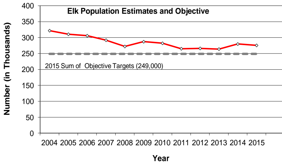
Figure 3. Estimated statewide post-hunt elk population versus total DAU population objectives for 2015. Current estimates based on 2015 models.
